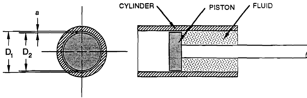
Figure 9.1 Typical Single Acting Actuator
