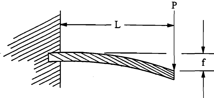
Figure 4.6 Typical Cantilever Spring
