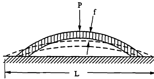
Figure 4.7 Typical Beam Spring
