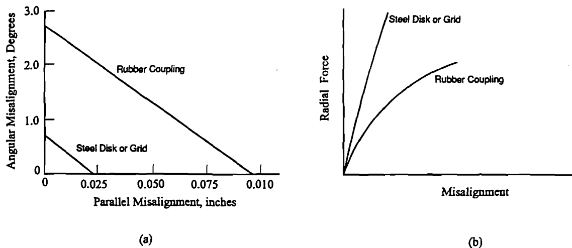
Figure 17.4 Coupling Characteristics
