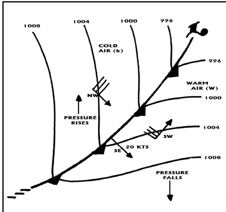
Figure 3-11 Cold Front
