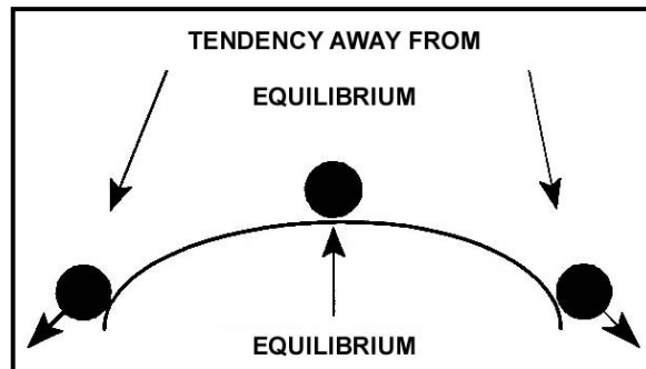
Figure 2-21 Unstable
