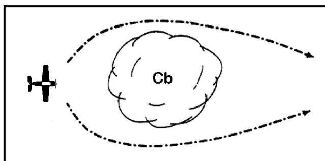
Figure 4-10 Around a Thunderstorm
