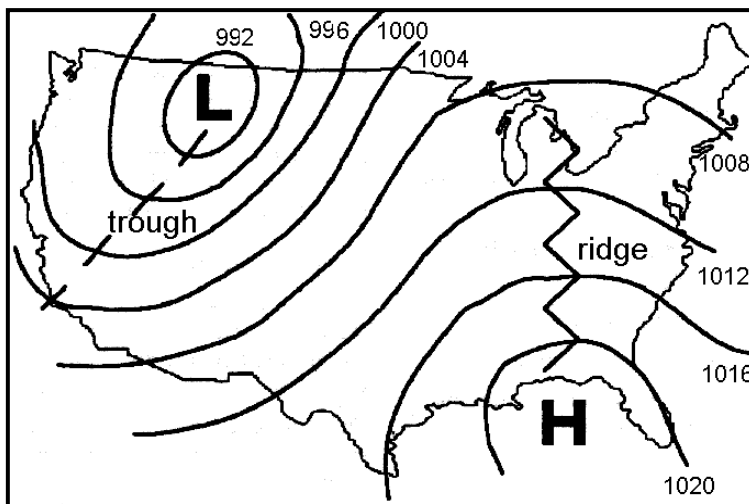
Figure 1-6 Pressure Systems
