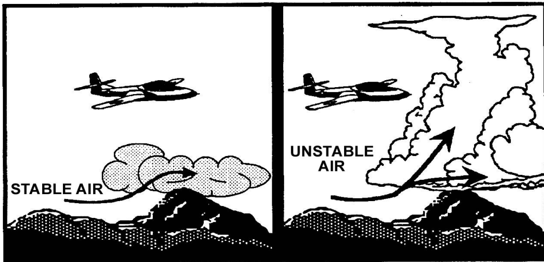
Figure 2-24 Clouds in Stable and Unstable Air
