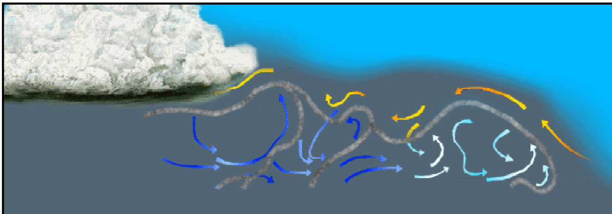
Figure 4-2 Gust Front
