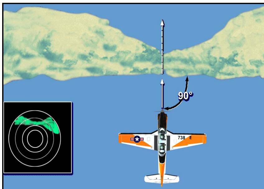
Figure 4-14 Thunderstorm Penetration
