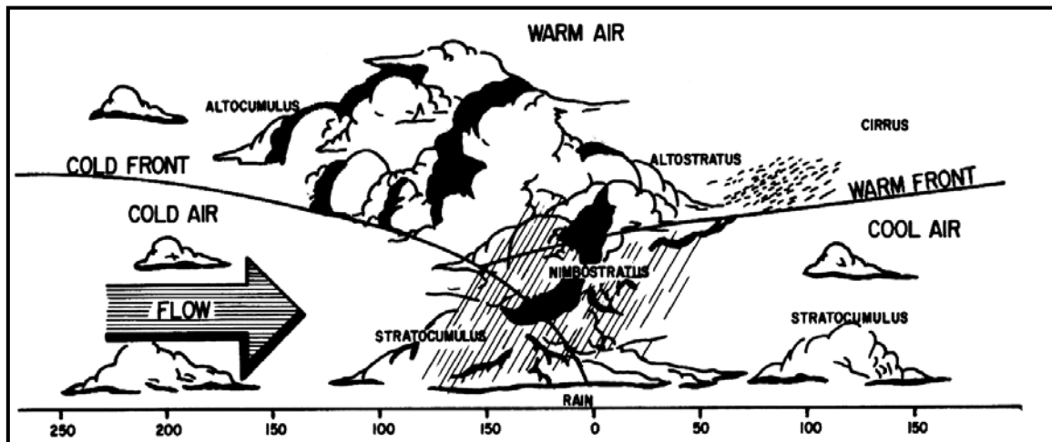
Figure 3-17 Occluded Front
