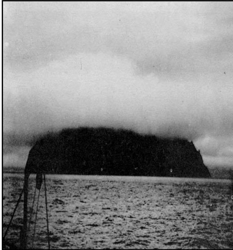
Figure 2-14 Stratus
