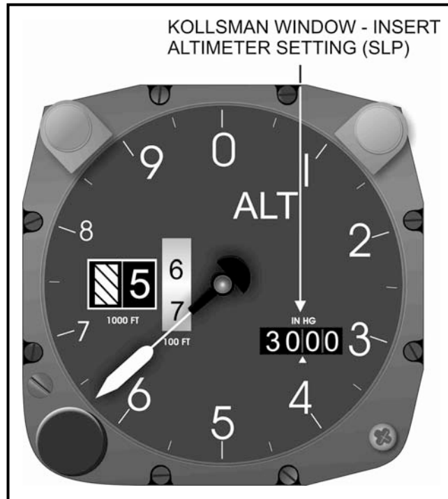
Figure 1-7 Barometric Altimeter (aka Pressure Altimeter)
