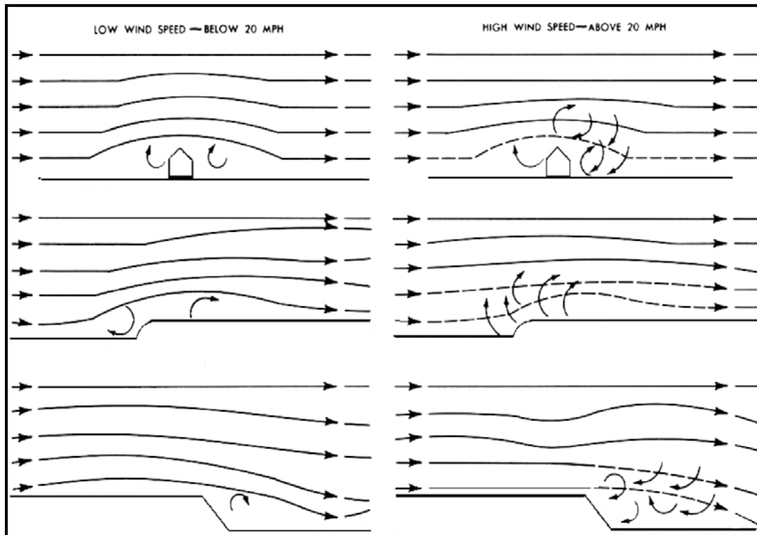
Figure 5-3 Airflow Over Irregular Terrain
