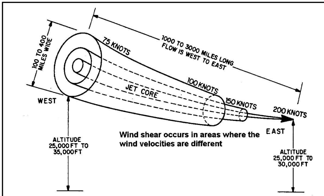
Figure 2-9 Jet Stream
