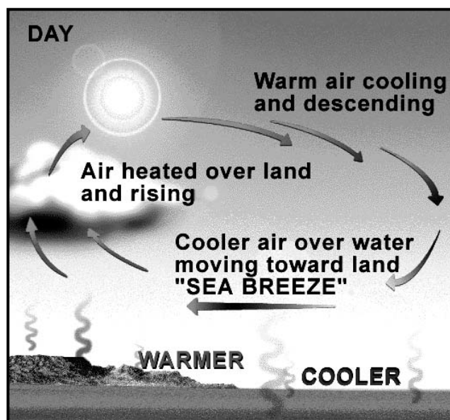
Figure 2-10 Sea Breeze
