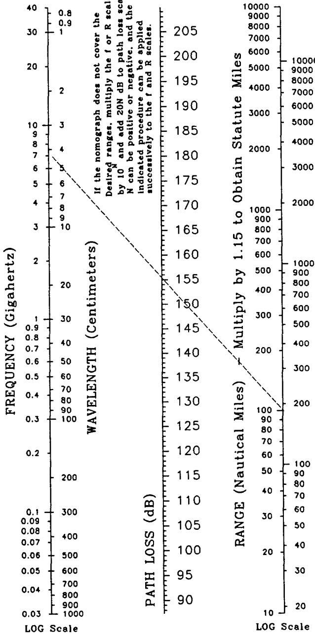
Figure 6. One-Way Space Loss Nomograph For Distances Greater Than 10 Nautical Miles
