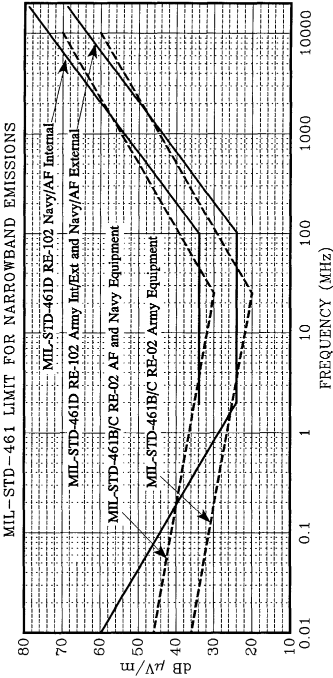
Figure 2. MIL-STD-461 Narrowband Radiated Emissions Limits
