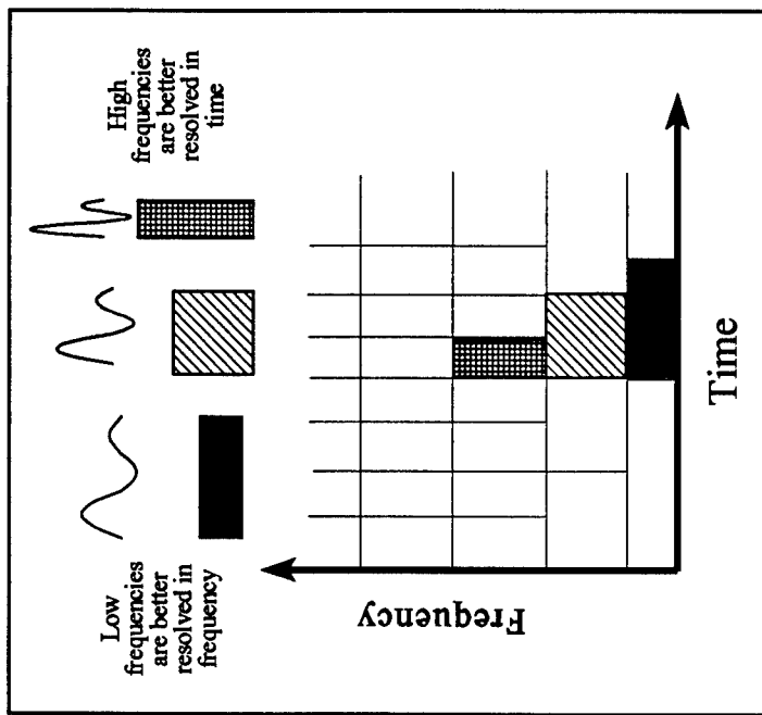
Figure 6 Wavelet Transform
