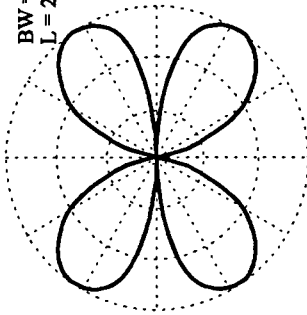
Figure 1. Frequency Effects
