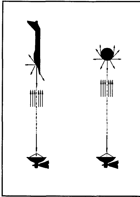
Figure 1. Concept of Radar Cross Section
