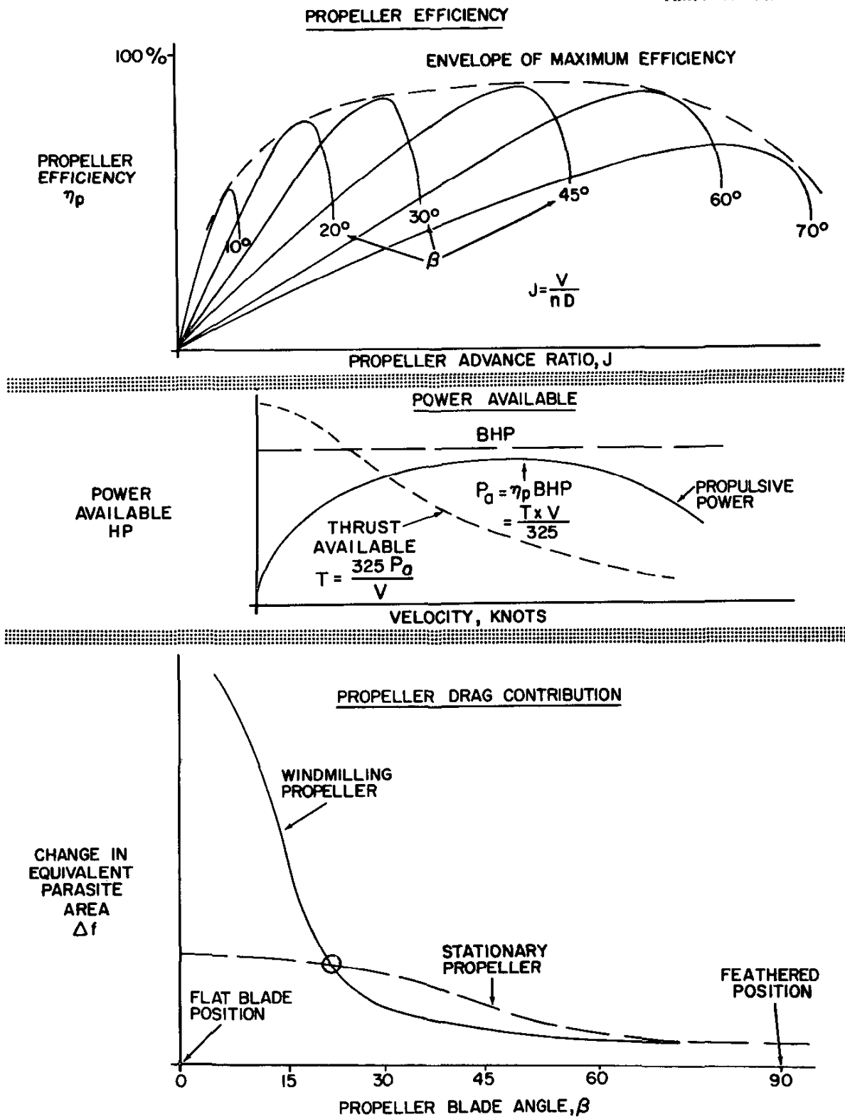
Figure 2.19. Propeller Operation
