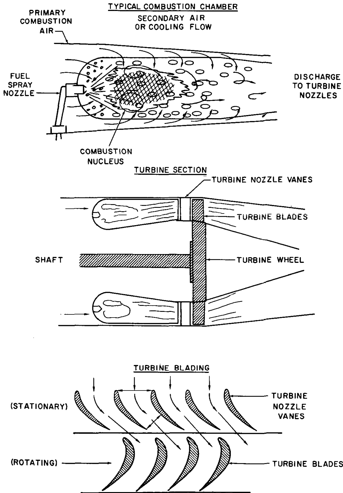
Figure 2.8. Combustion Chamber and Turbine Components
