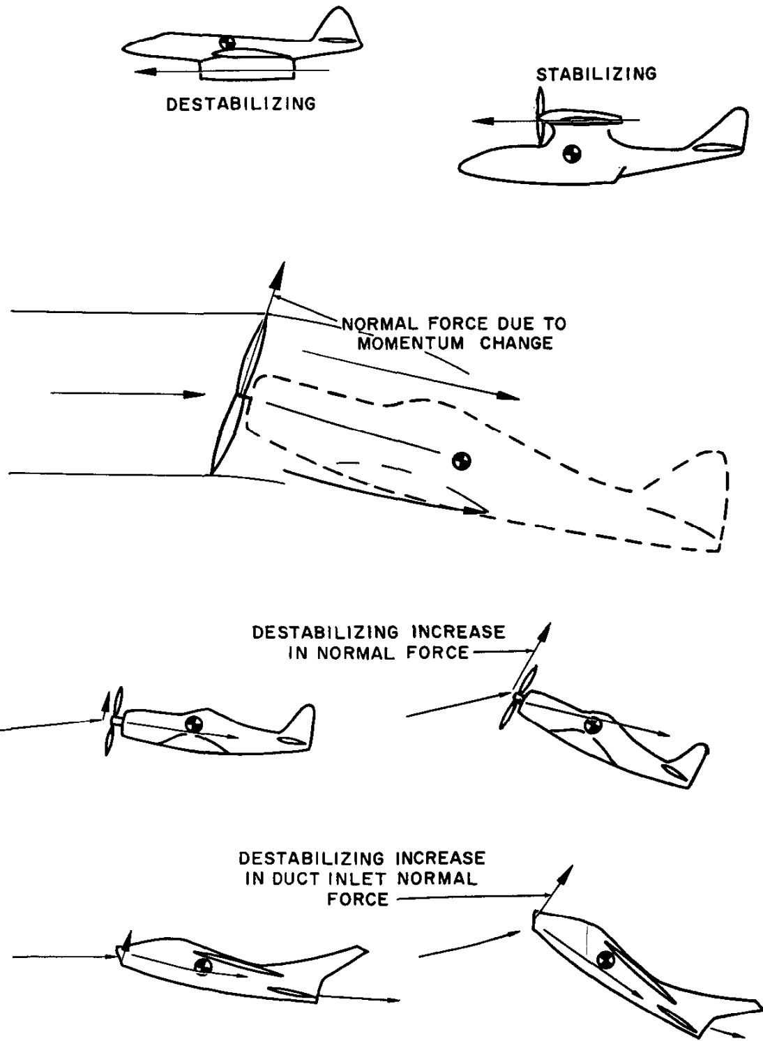
Figure 4.11. Direct Power Effects
