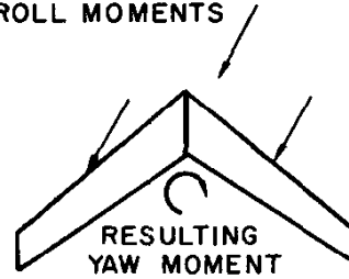
SWEPT WING IN A SIDESLIP TO THE RIGHT RESULTING YAW MOMENT
