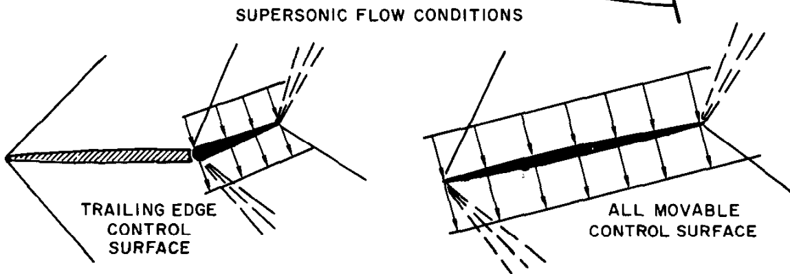
Figure 3.19. Planform Effects and Control Surfaces
