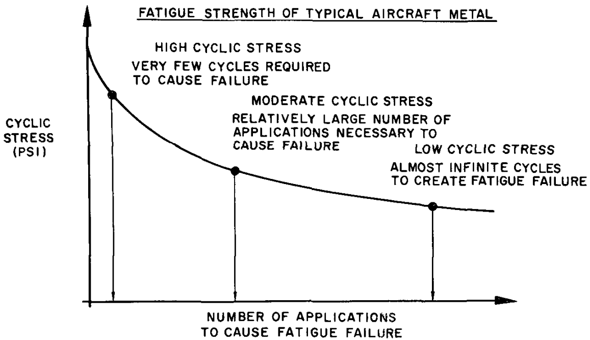
Figure 5.1. Strength Characteristics
