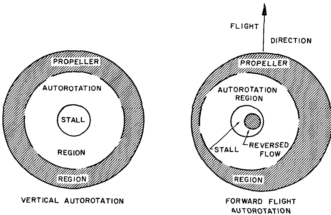
Figure 6.17. Rotor Autorotation Flow Conditions
