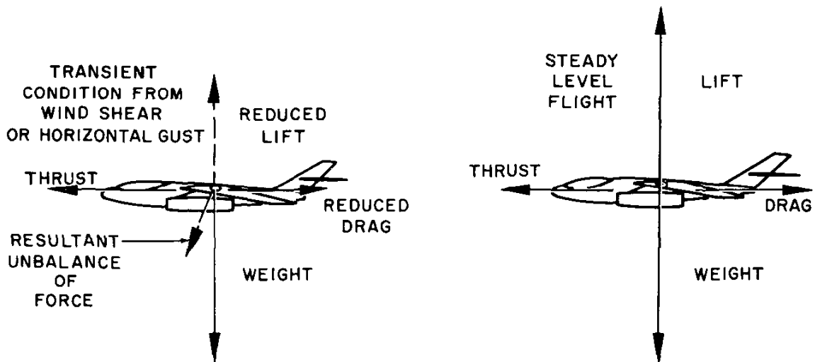
Figure 6.5. Effect of Wind Shear
