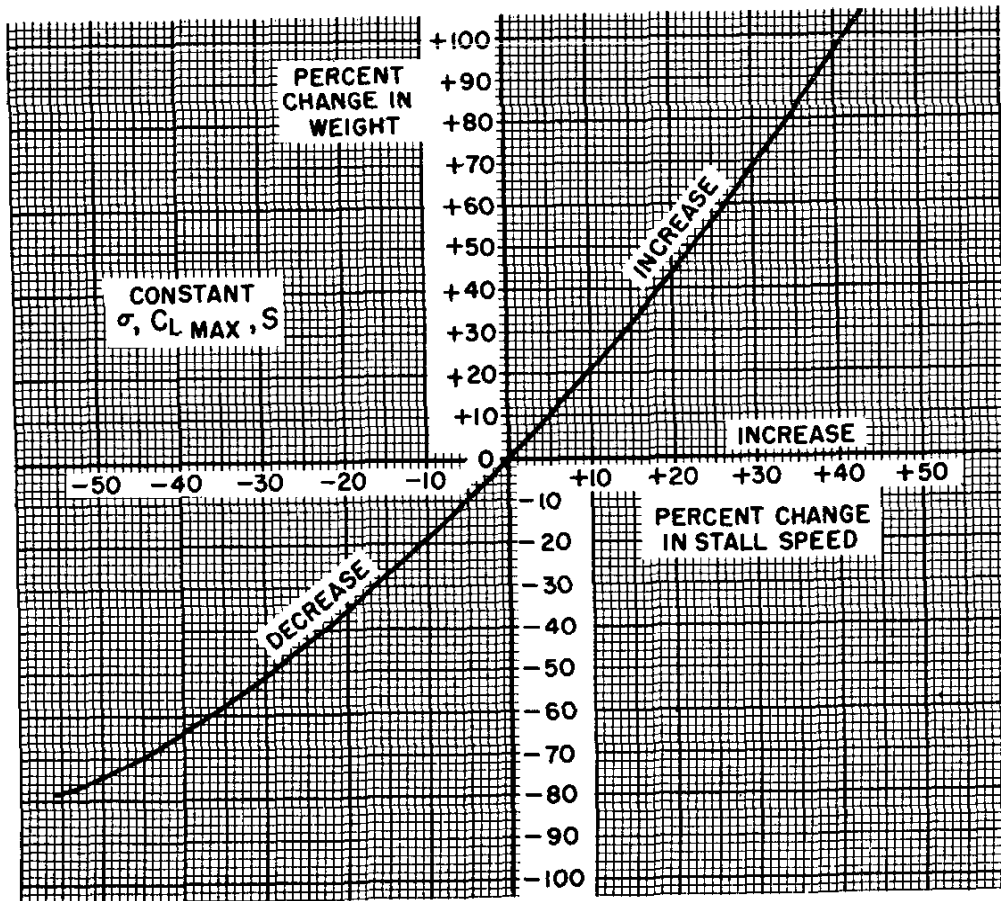
Figure 1.15. Flight at High Lift Conditions
