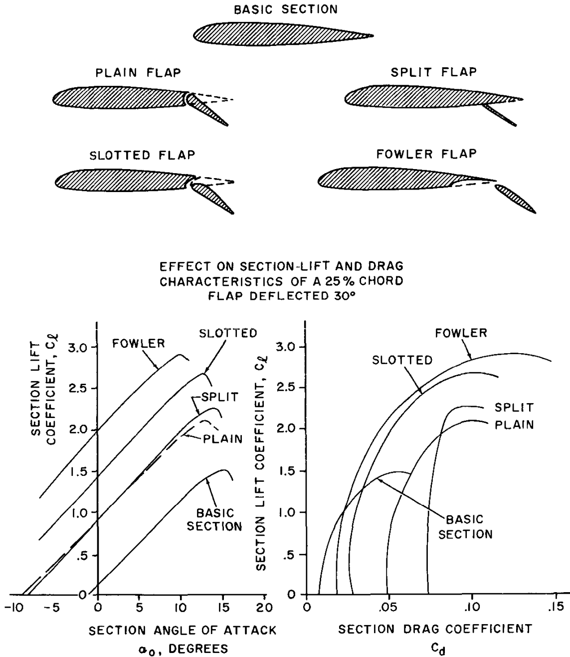
Figure 1.17. Flap Configurations
