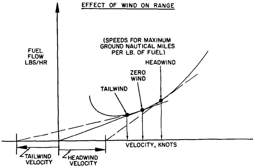
Figure 2.26. Range Performance
