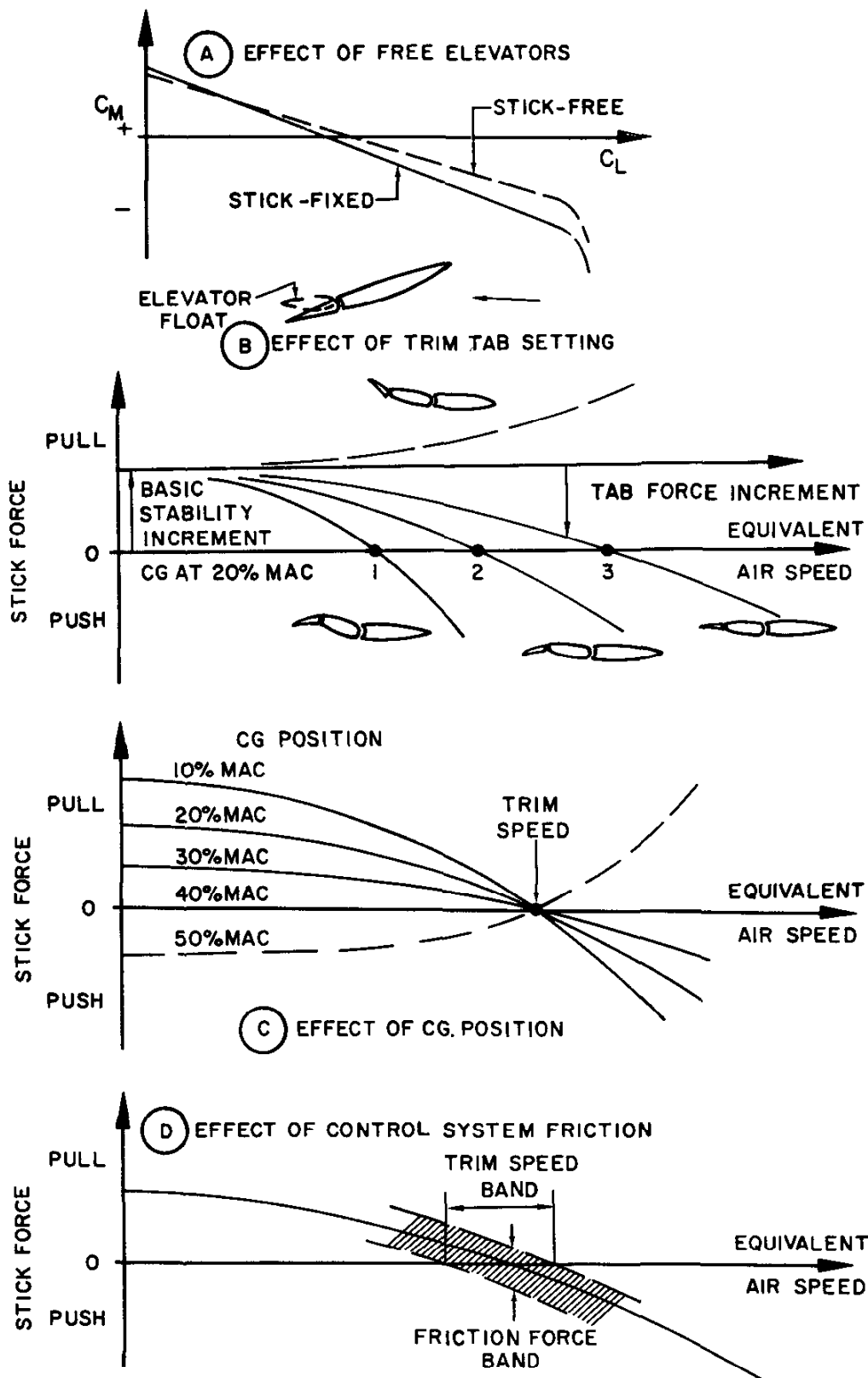
Figure 4.14. Control Force Stability
