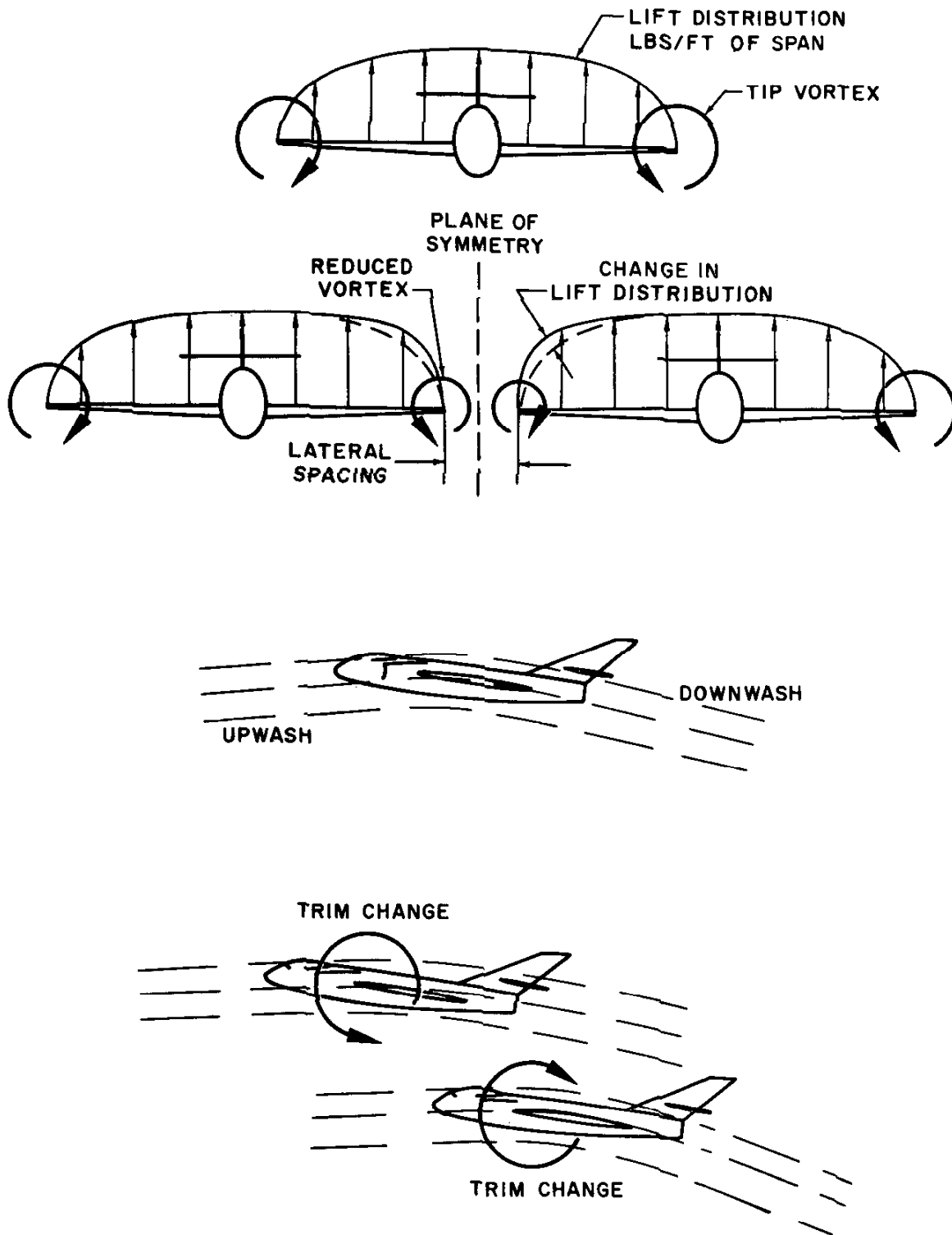
Figure 6.10. Interference Between Airplanes in Flight
