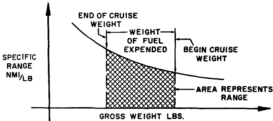
Figure 2.23. General Range Performance
