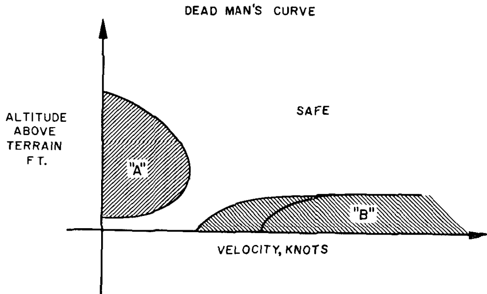
Figure 6.18. Autorotation Characteristics
