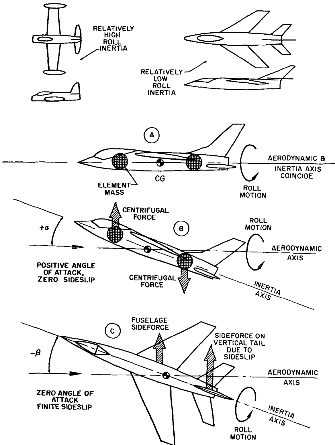
Figure 4.34. Roll Coupling
