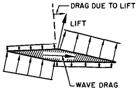
(f) DOUBLE WEDGE PRESSURE DISTRIBUTION AT POSITIVE LIFT
