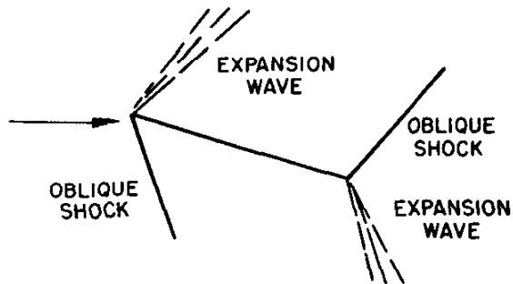
(a) FLAT PLATE WAVE PATTERN
