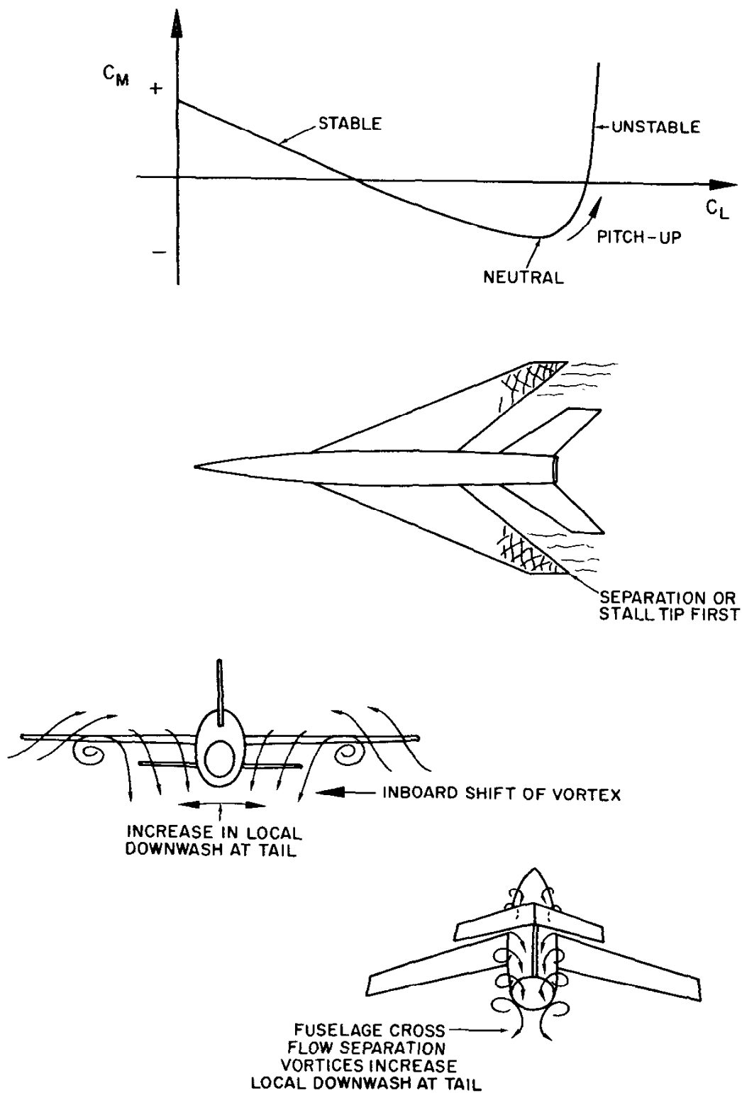
Figure 4.33. Pitch-up
