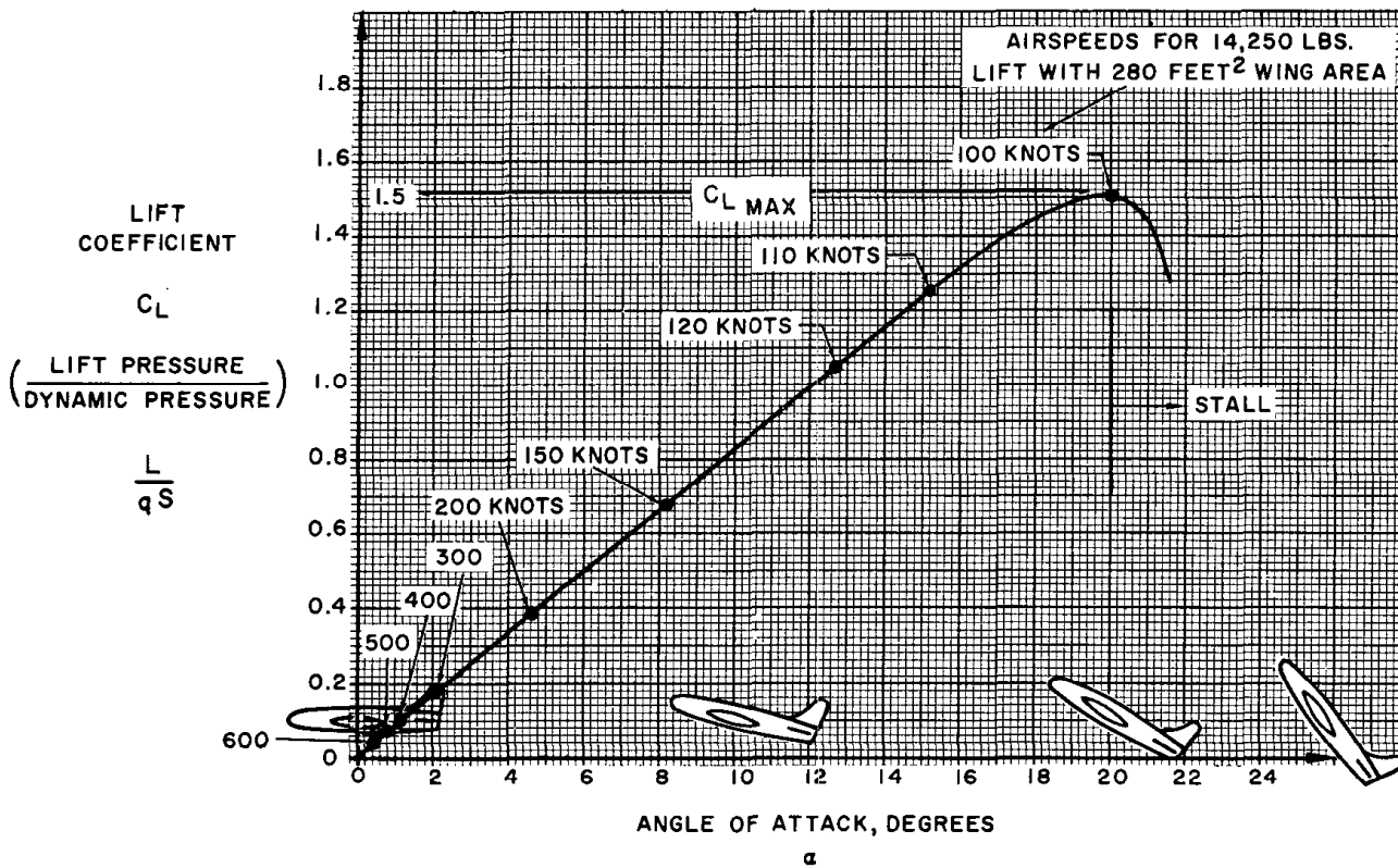
Figure 1.11. Typical Lift Characteristics
