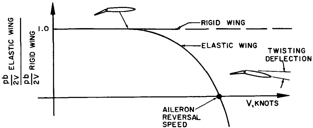
Figure 4.30. Control in Roll
