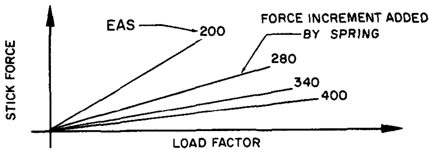
Figure 4.16. Tailoring Control Forces
