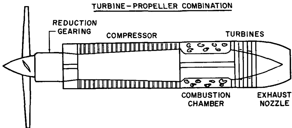
Figure 2.14. Thrust Augmentation and the Gas Turbine-Propeller Combination
