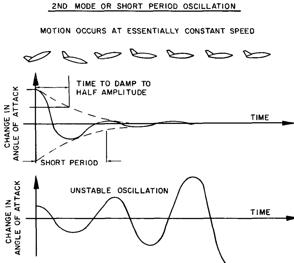
Figure 4.20. Longitudinal Dynamic Stability
