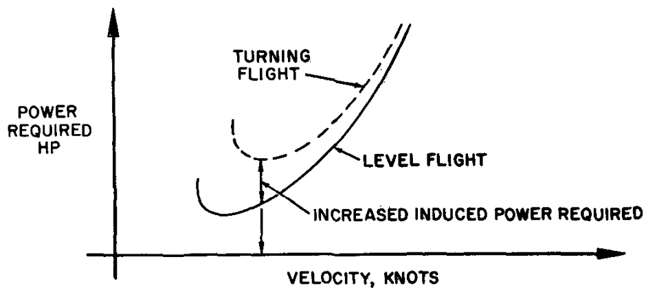
Figure 2.28. Effect of Turning Flight
