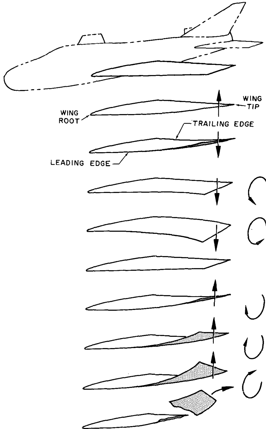
Figure 5.5. Aeroelastic Effects (Sheet 2 of 2)
