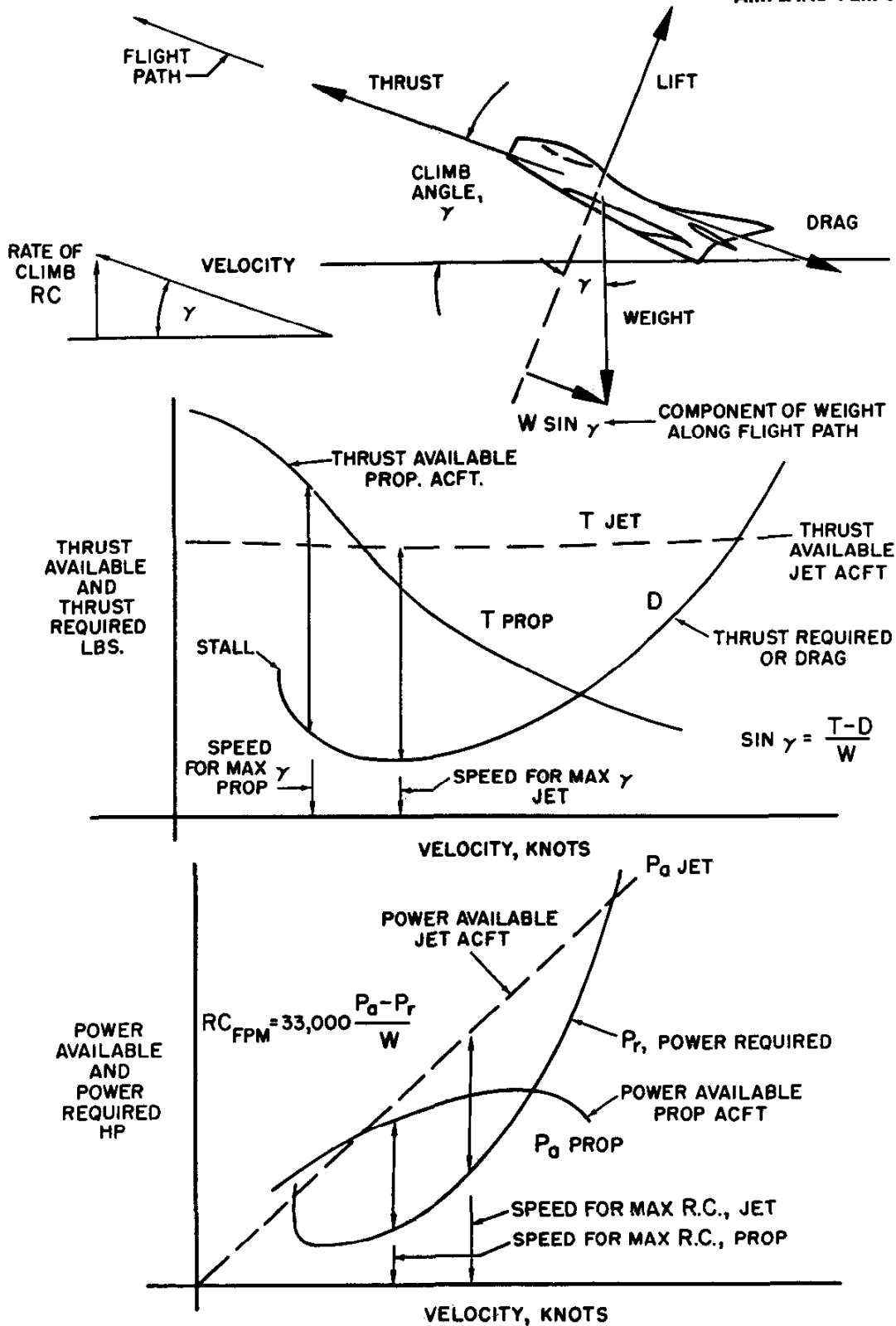
Figure 2.21. Climb Performance
