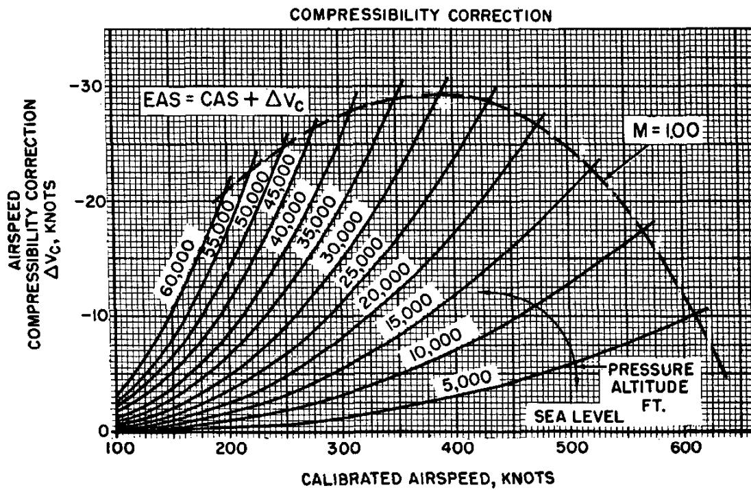
Figure 1.6. Airspeed Corrections (sheet 1 of 2)
