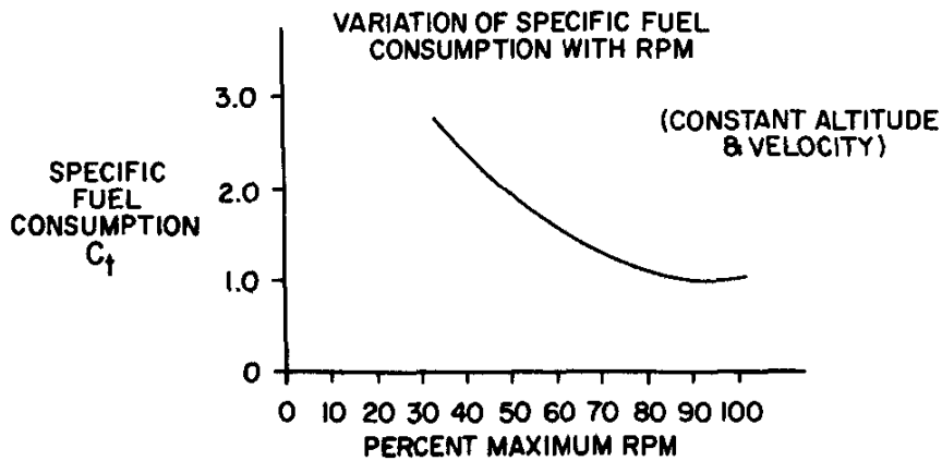
Figure 2.10. Turbojet Performance
