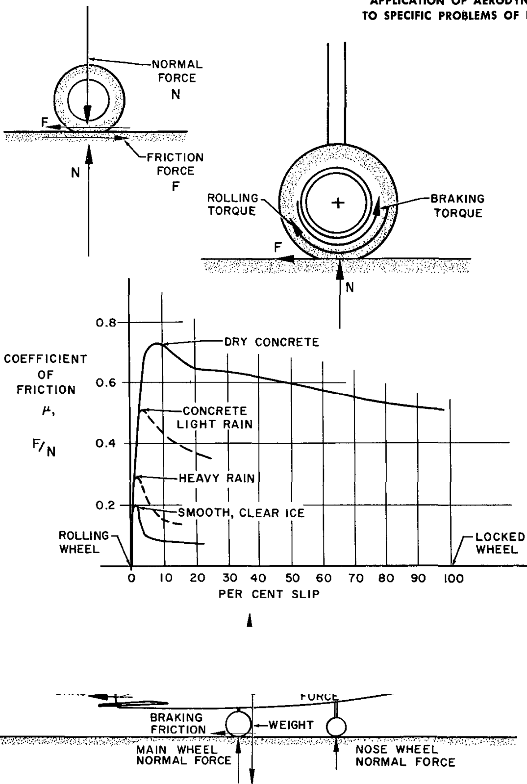
Figure 6.11. Braking Performance
