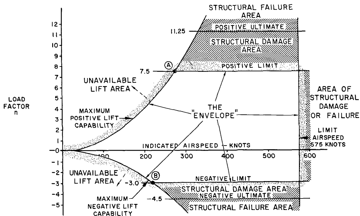
Figure 5.4. Significance of the V-n Diagram
