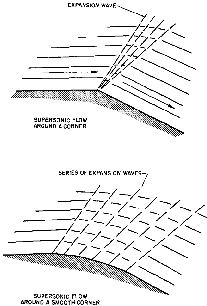
Figure 3.7. Expansion Wave Formation
