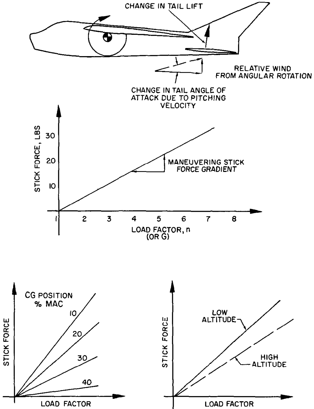
Figure 4.15. Maneuvering Stability
