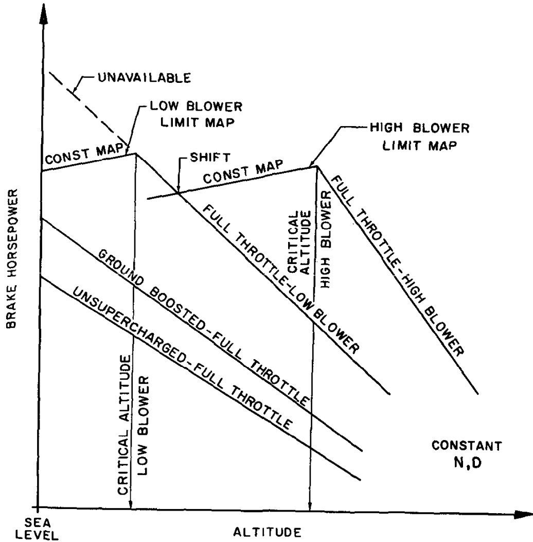
Figure 2.17. Effect of Supercharging on Altitude Performance
