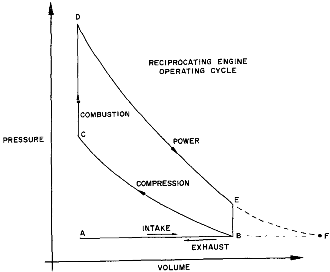
Figure 2.15. Reciprocating Engines
