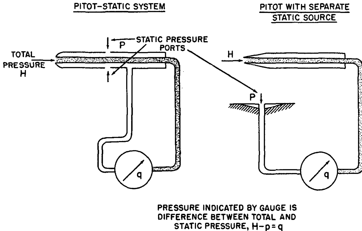
Figure 1.5. Airspeed Measurement
