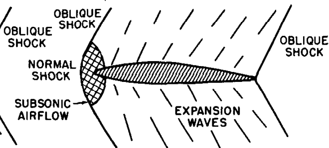
(b) CONVENTIONAL BLUNT NOSE AIRFOIL
