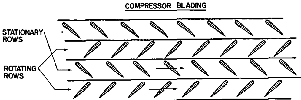
Figure 2.7. Compressor Types
