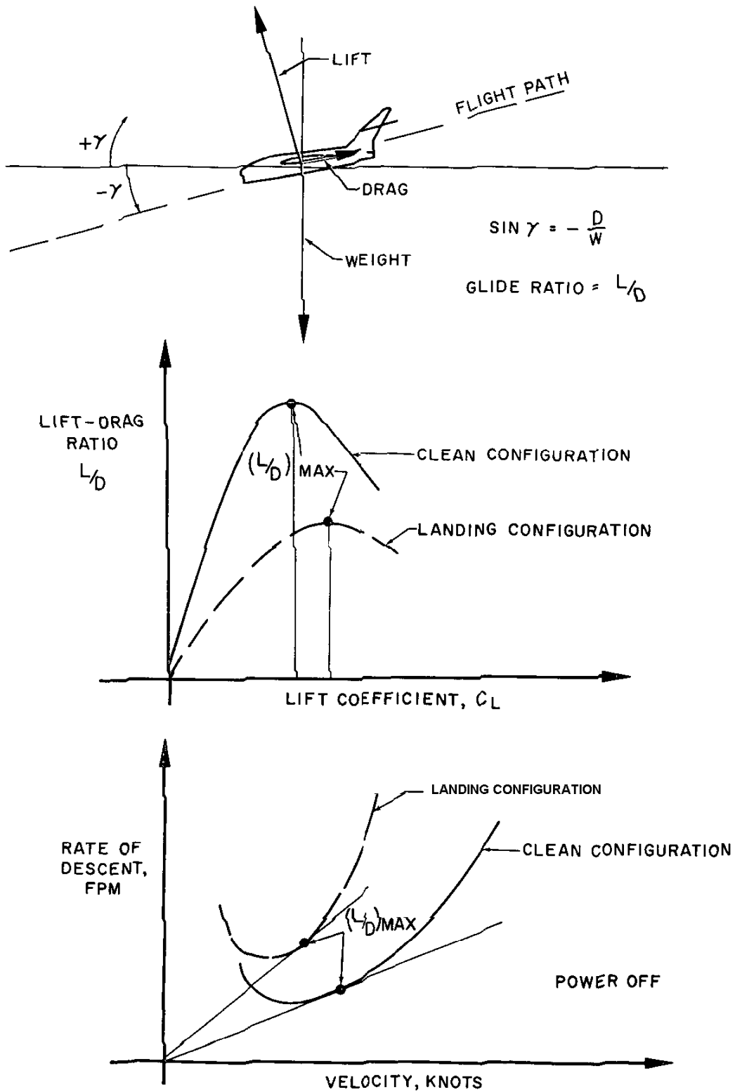
Figure 6.6. Glide Performance
