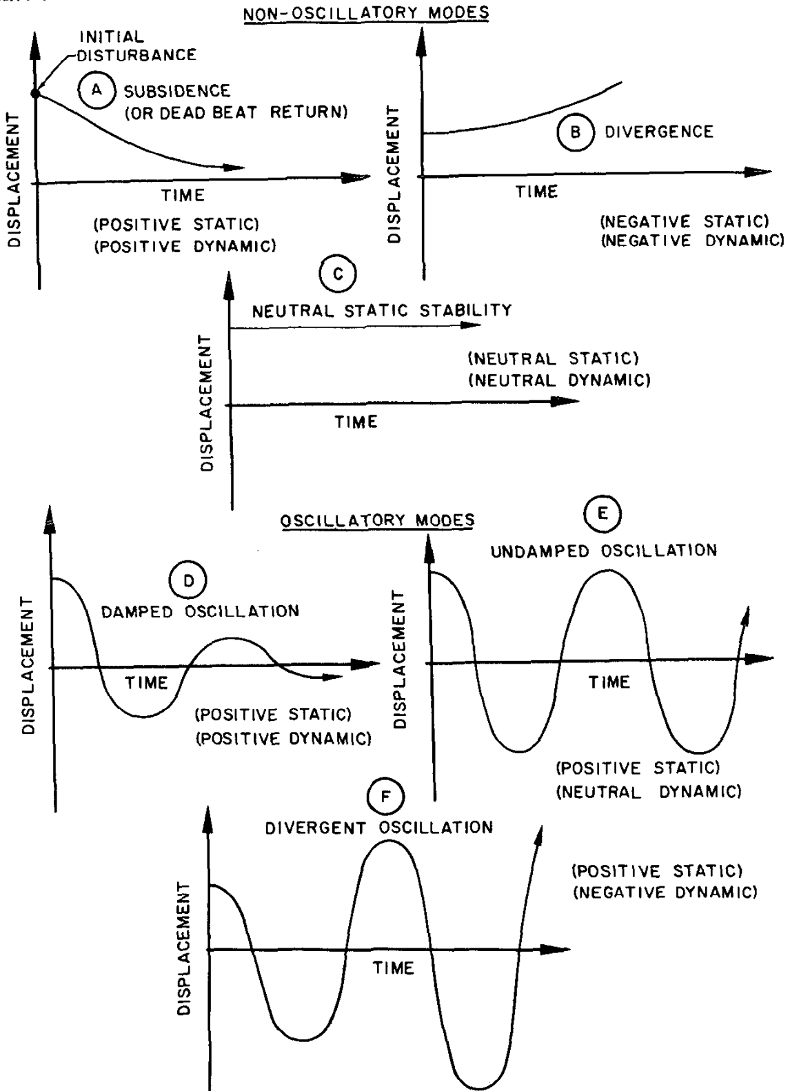
Figure 4.2. Dynamic Stability
