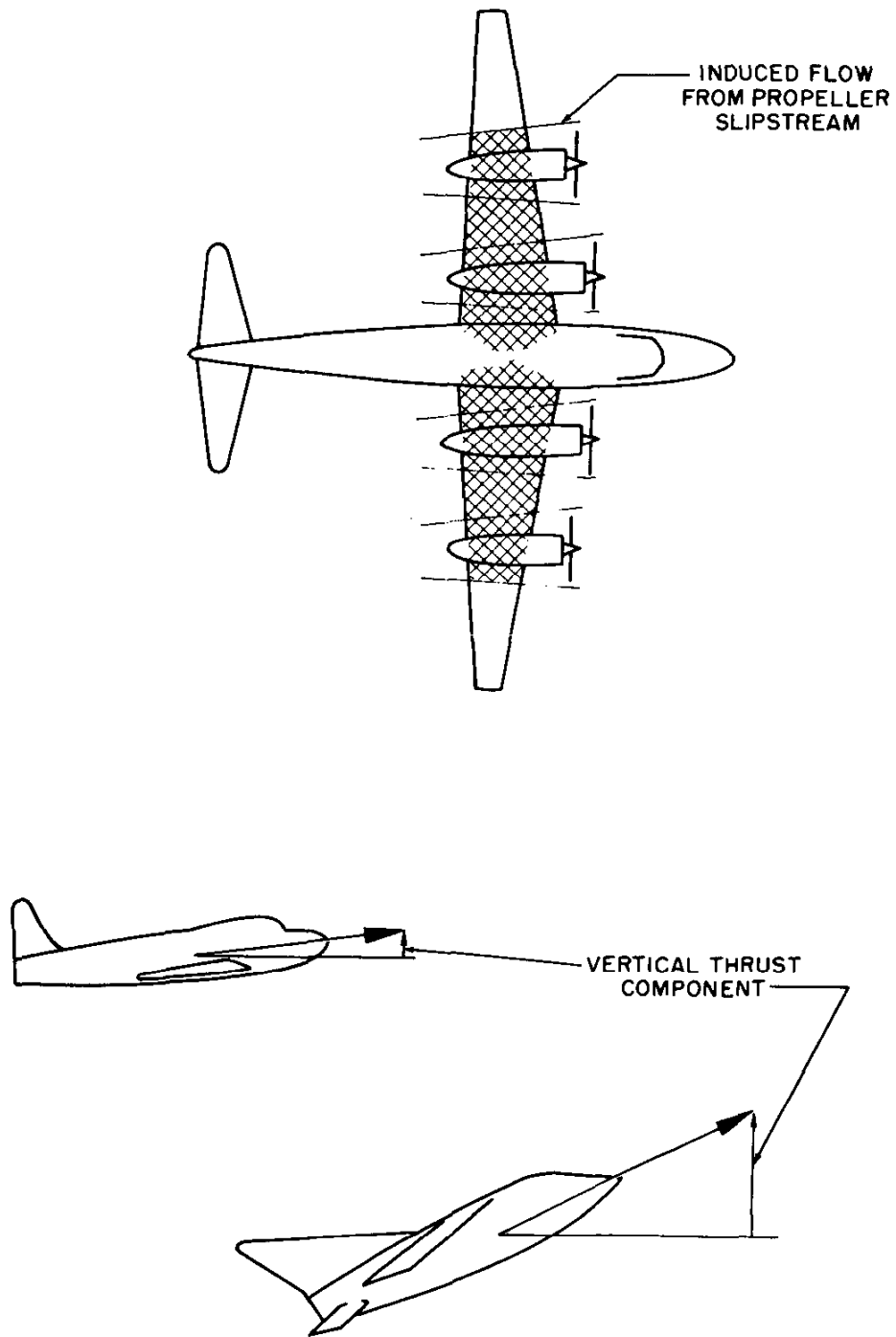
Figure 1.20. Power Effects
