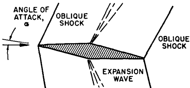
(e) DOUBLE WEDGE WAVE PATTERN AT POSITIVE ANGLE OF ATTACK
