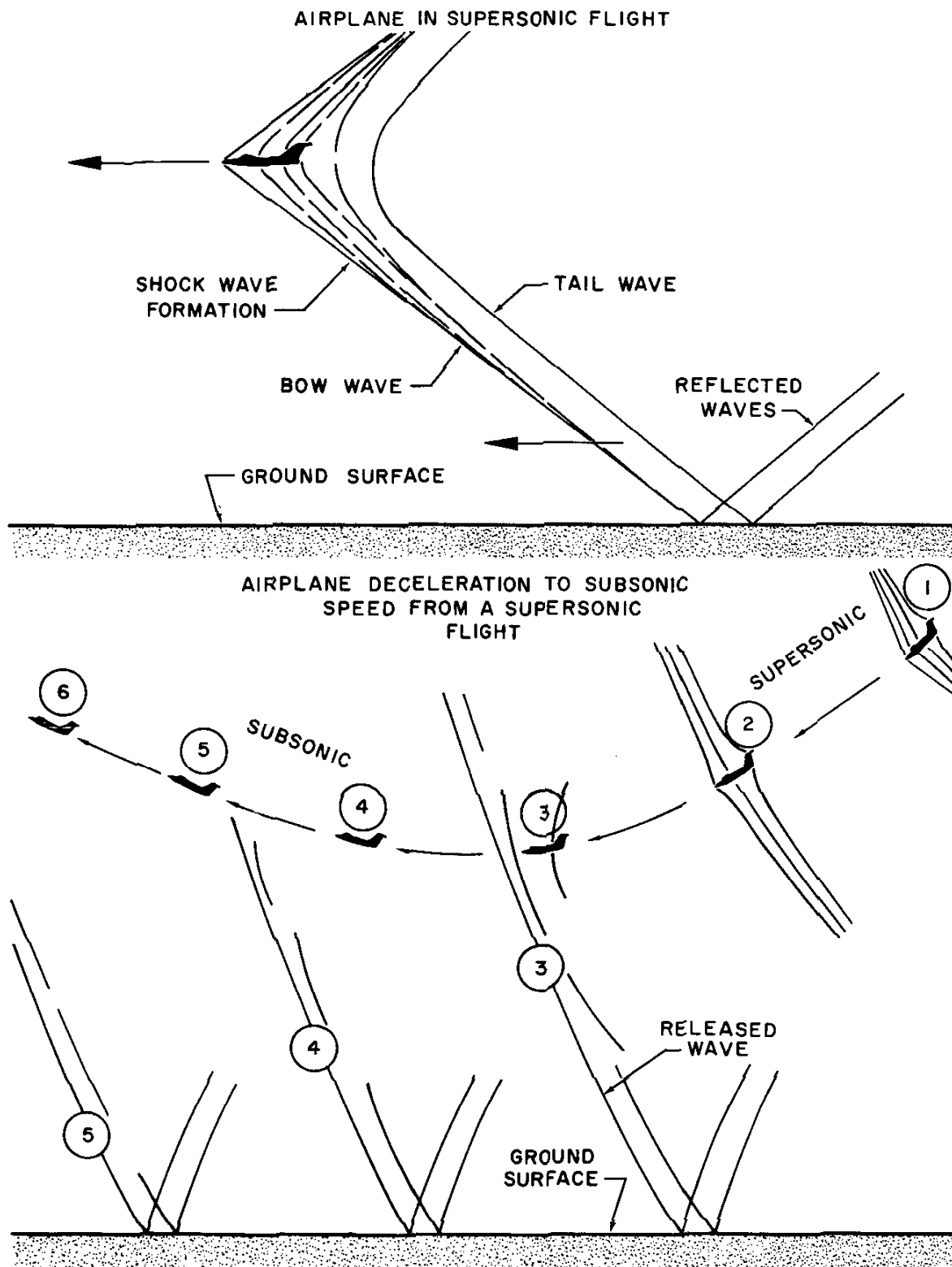
Figure 6.14. Sonic Booms
