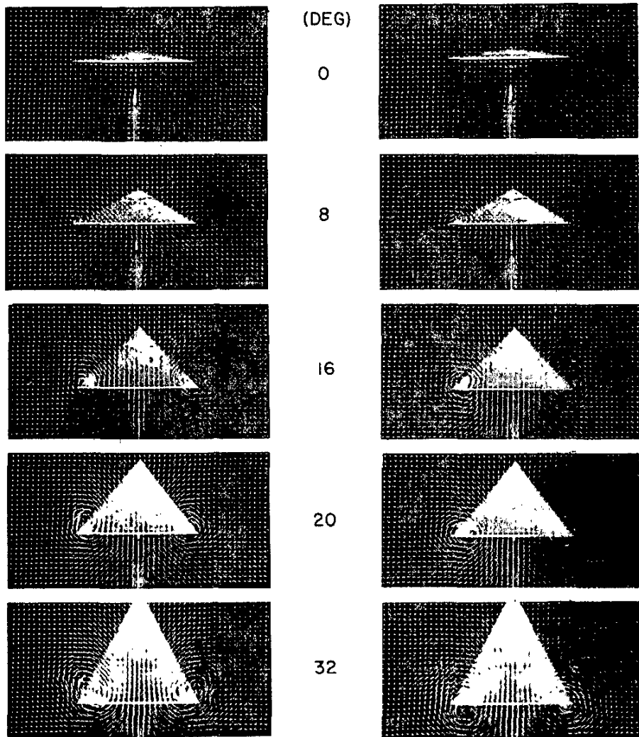
(a) TUFT GRID 6 INCHES FROM TRAILING EDGE.
