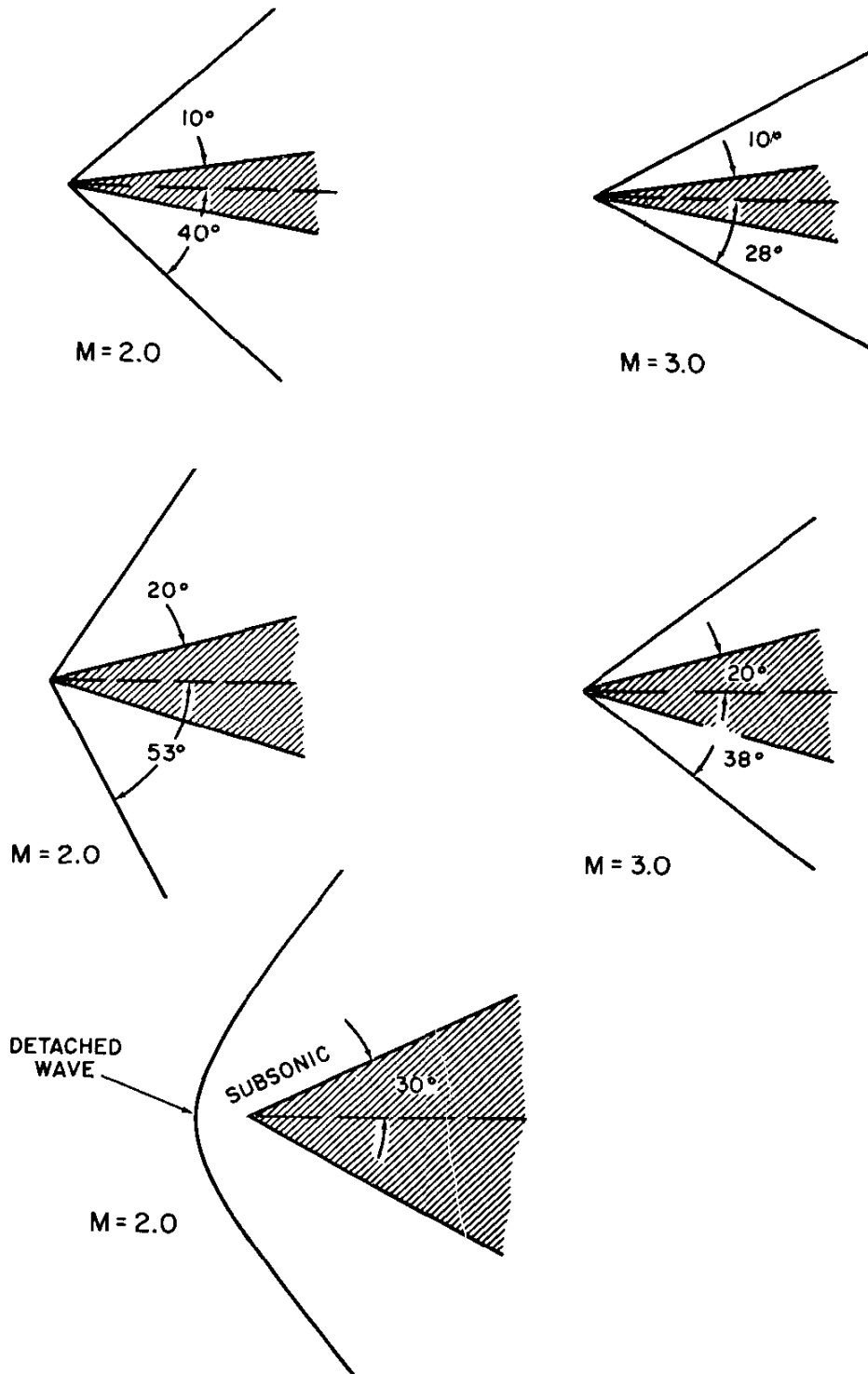
Figure 3.4. Shock Waves Formed by Various Wedge Shapes
