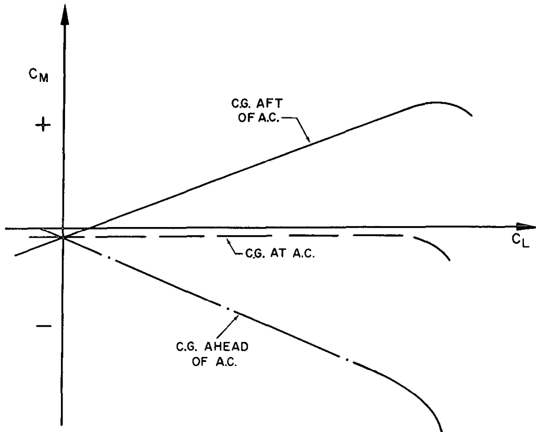
Figure 4.6. Wing Contribution
