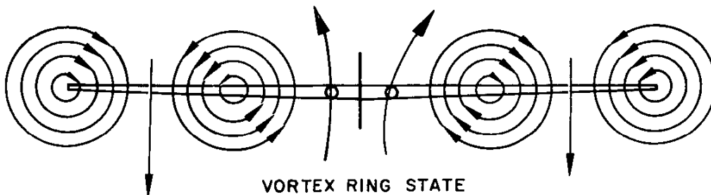
Figure 6.19. Rotor Downwash Distribution
