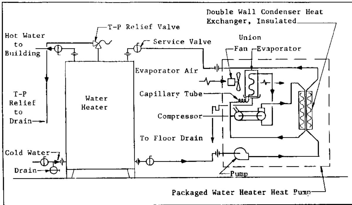
FIGURE 2 Air Source Heat Pump
