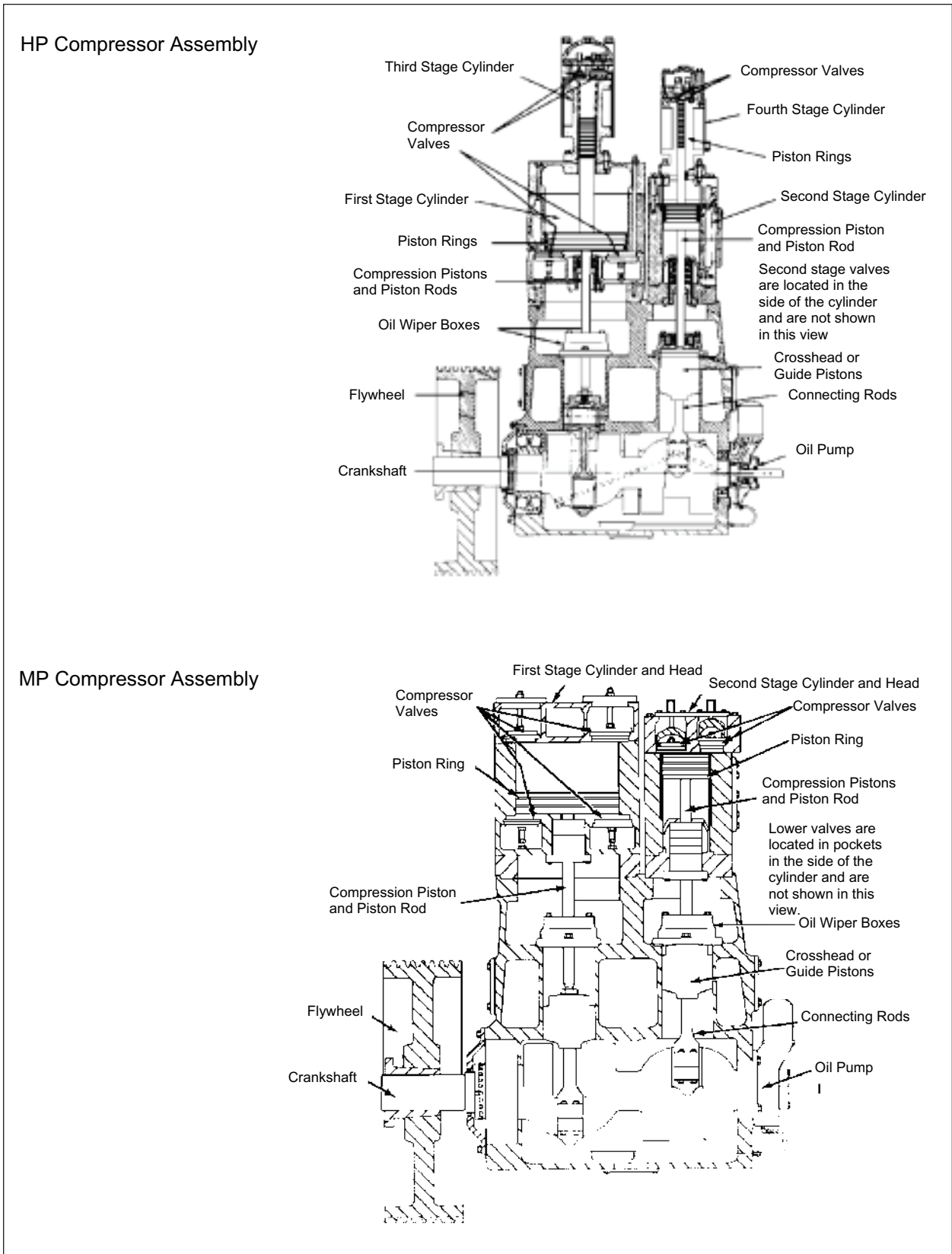
Figure 8-10. HP Compressor Assembly (top); MP Compressor Assembly (bottom).
