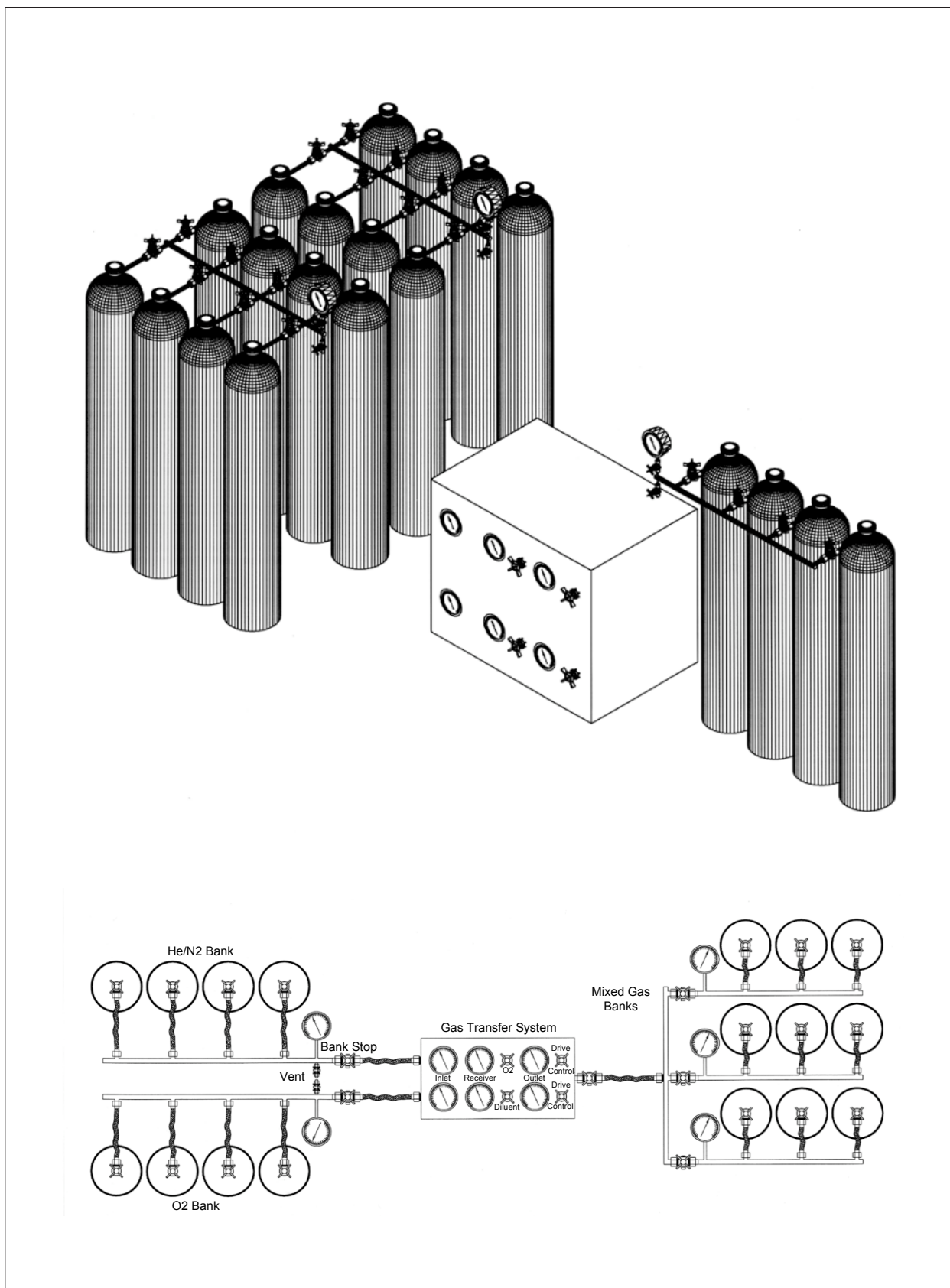
Figure 16-2. Mixing with Gas Transfer System.
