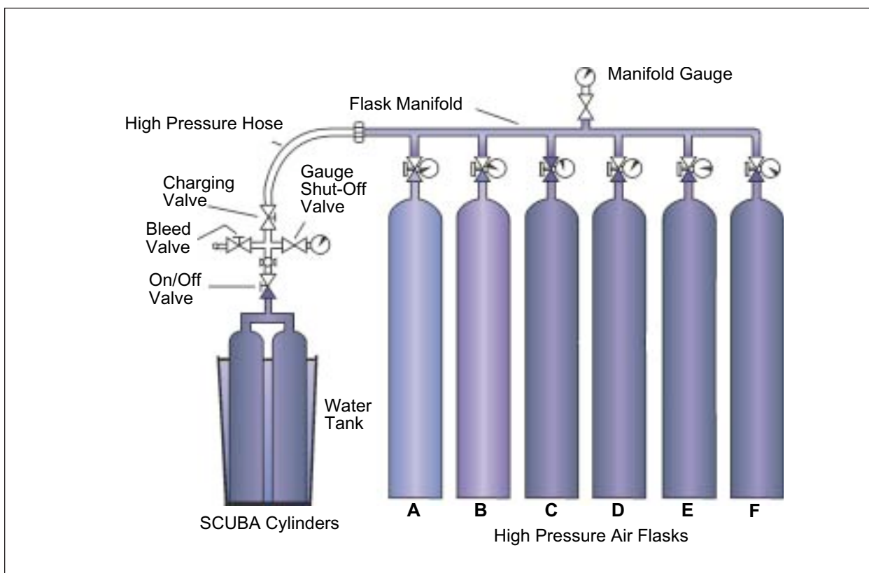
Figure 7-6. Cascading System for Charging SCUBA Cylinders.
