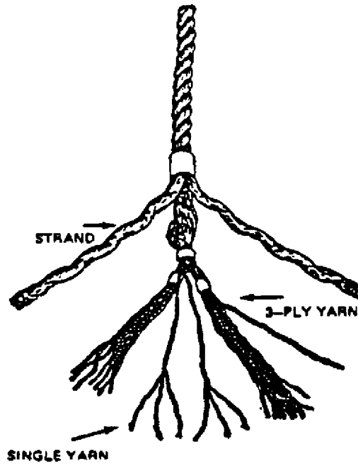
Figure 613-2-1. Synthetic Fiber Plain-Laid Rope
