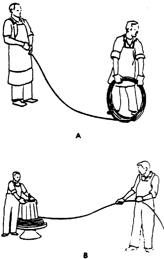
Figure 613-1-7. Uncoiling Wire Rope
