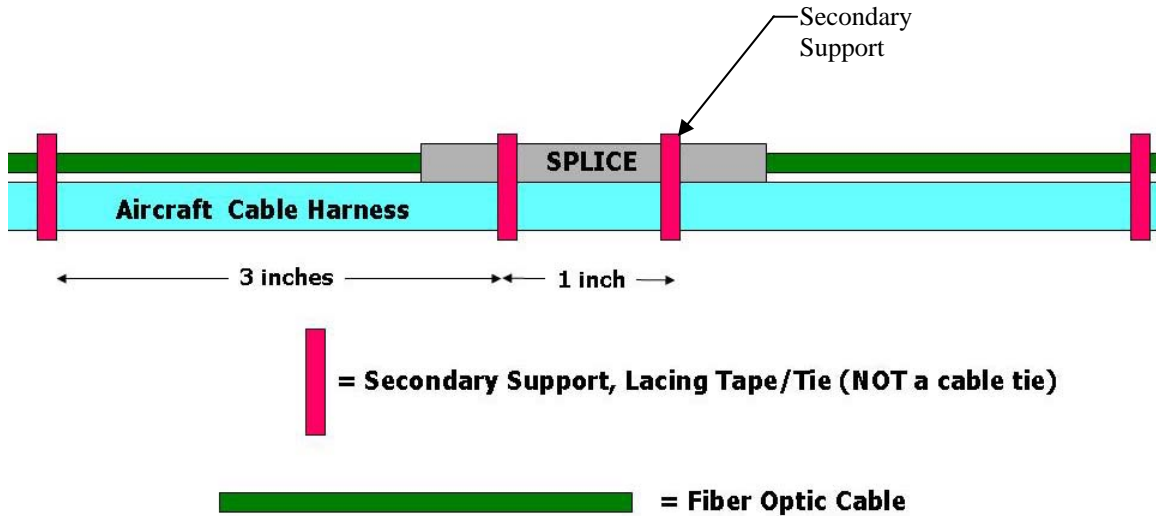
Figure 1. Secondary support spacing to secure mechanical splice to cable harness.
