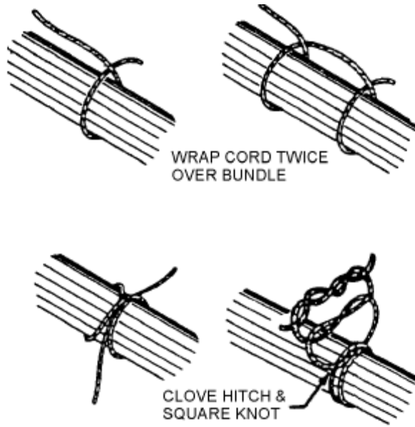
Figure 4. Lacing process for secondary support.
