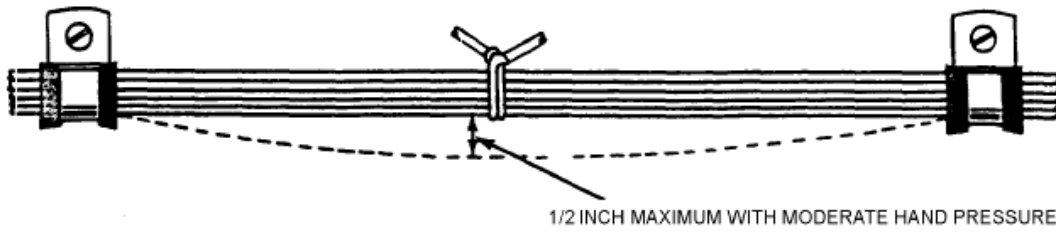
Figure 3. Allowed slack between primary supports.
