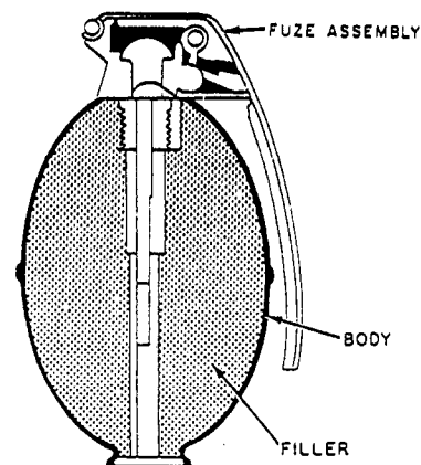
Figure 12-7.—Three main parts of the grenade.
