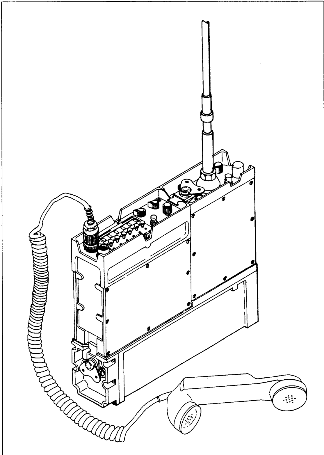
Figure 11-5C.—Radio Set AN/PRC-104 equipment supplied.
