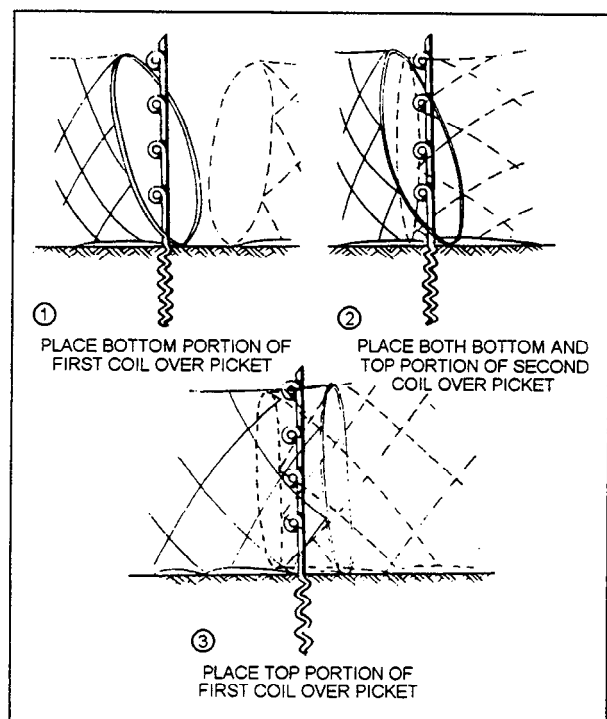
Figure 8-28.—Joining concertina.
