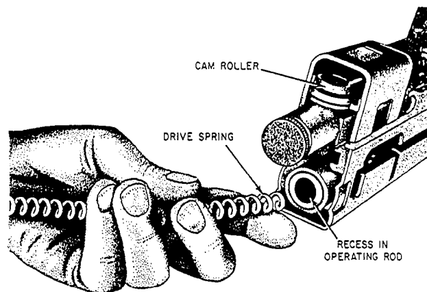
Figure 13-26.—Inserting the drive spring.
