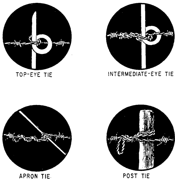
Figure 8-13.—Ties for erecting entanglements as seen from the friendly side.
