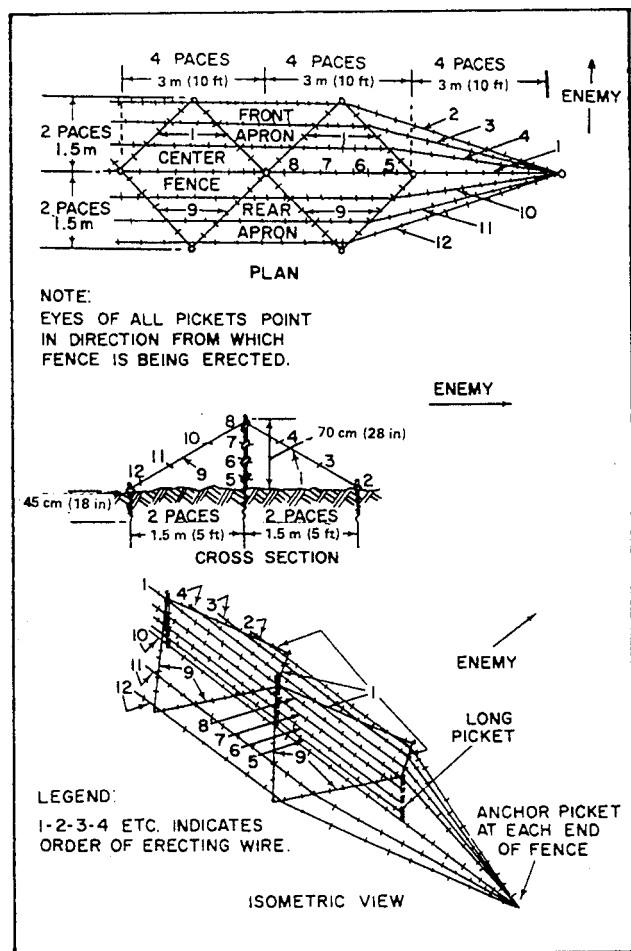
Figure 8-20.—Double-apron fence.
