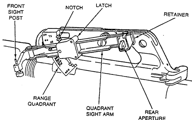
Figure 3-3.—Quadrant sight assembly.
