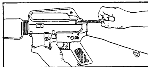
Figure 3-8.—Locking the bolt open.
