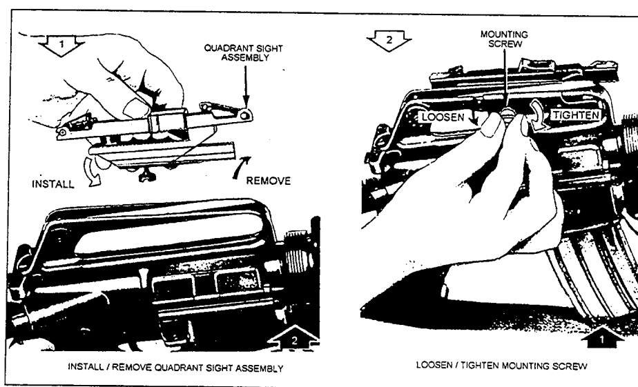
Figure 3-4.—Installation/removal of quadrant sight assembly.
