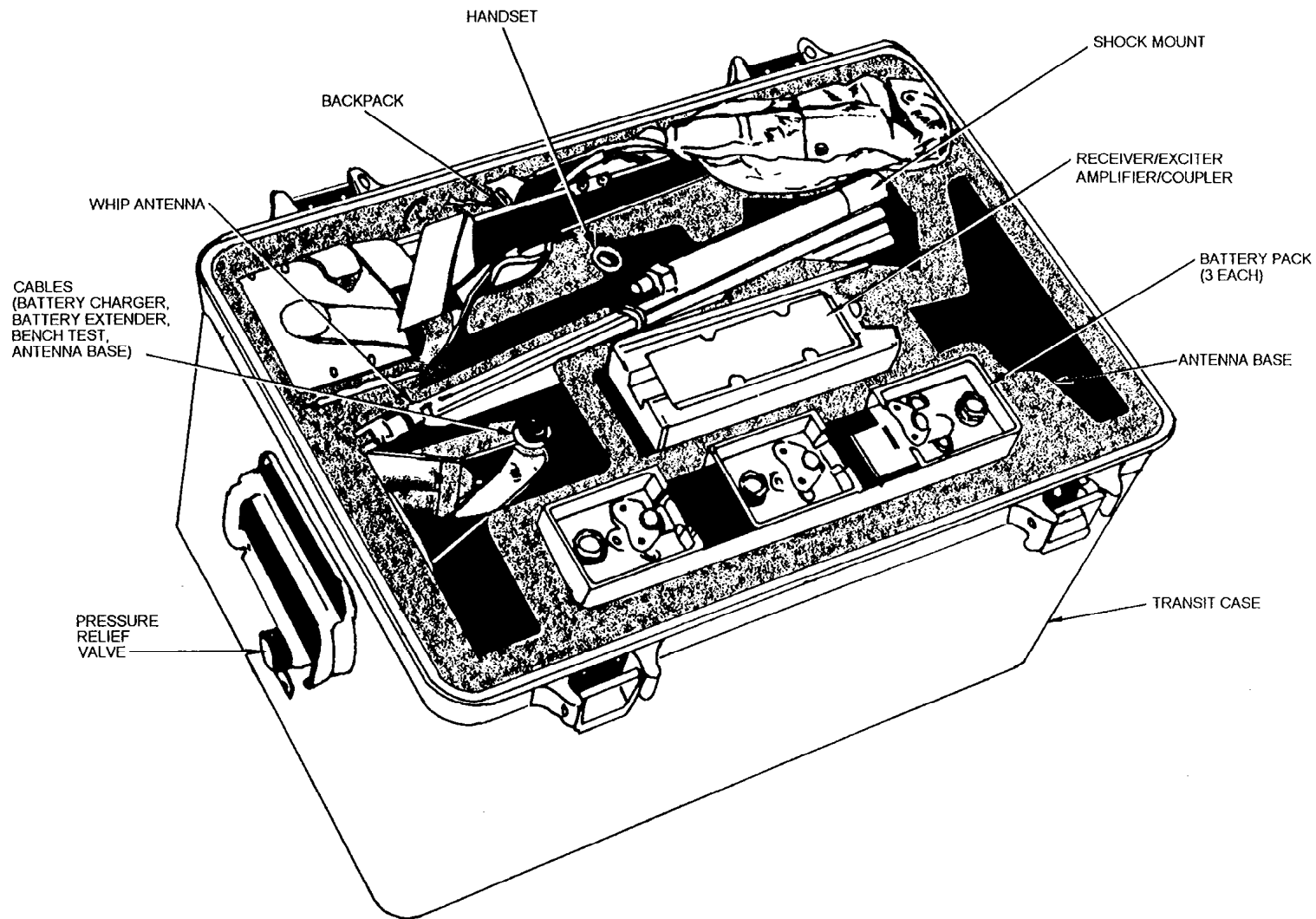
Figure 11-5A.—Radio Set AN/PRC-104 equipment supplied.
