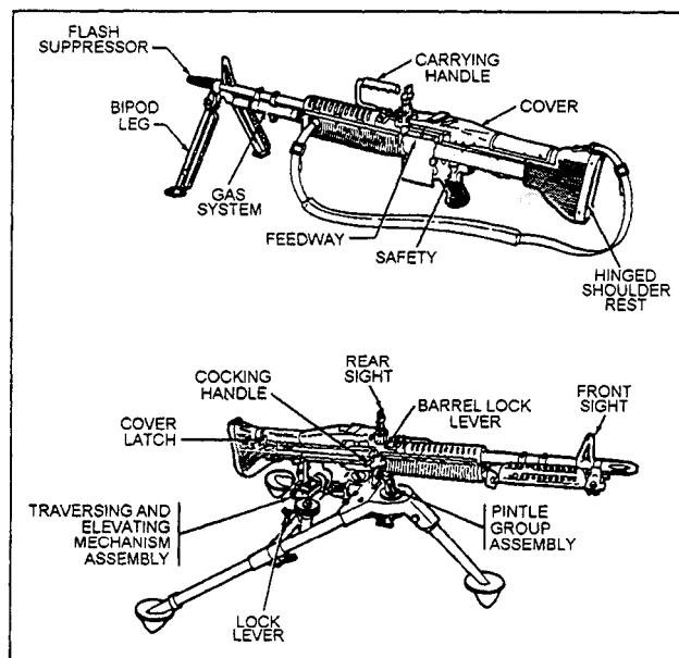
Figure 13-6.—External nomenclature of the M60 machine gun.
