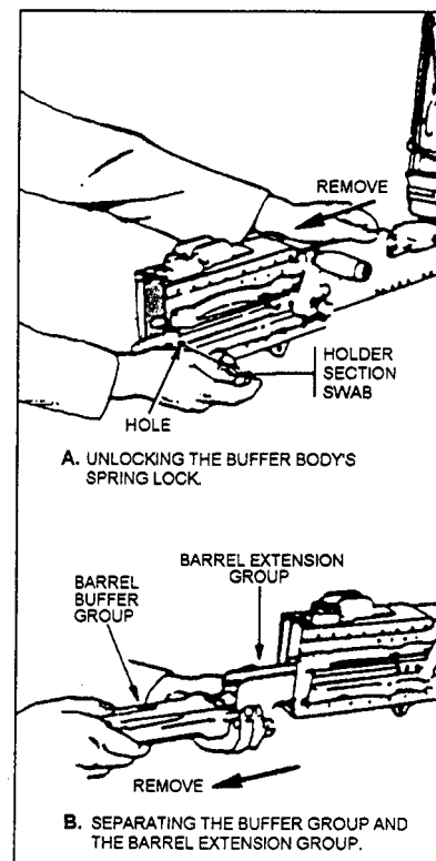
Figure 13-41.—Removing the buffer body and barrel extension groups.
