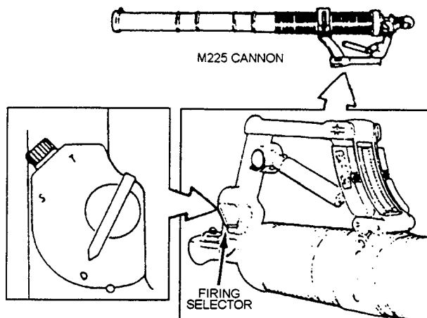
Figure 14-2.—M225 cannon.
