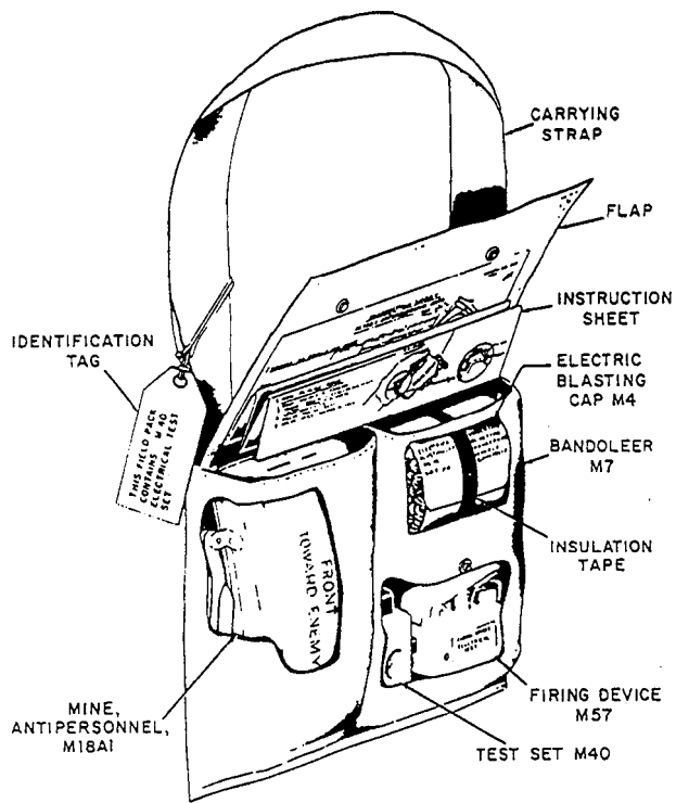
Figure 12-14.—The M18A1 antipersonnel mine and accessories packed in the M7 bandoleer.
