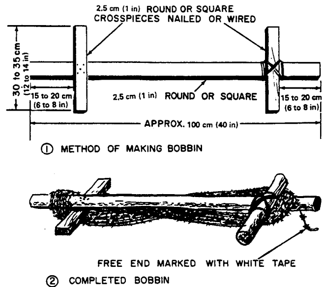
Figure 8-6.—Barbed-wire bobbin.
