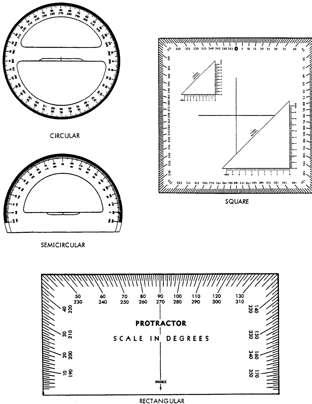
Figure 5-33.—Types of protractors.
