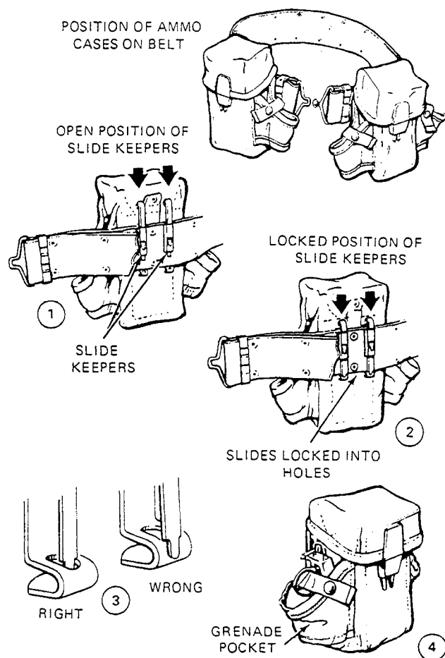
Figure 2-4.—Attaching ammo pouch to belt.
