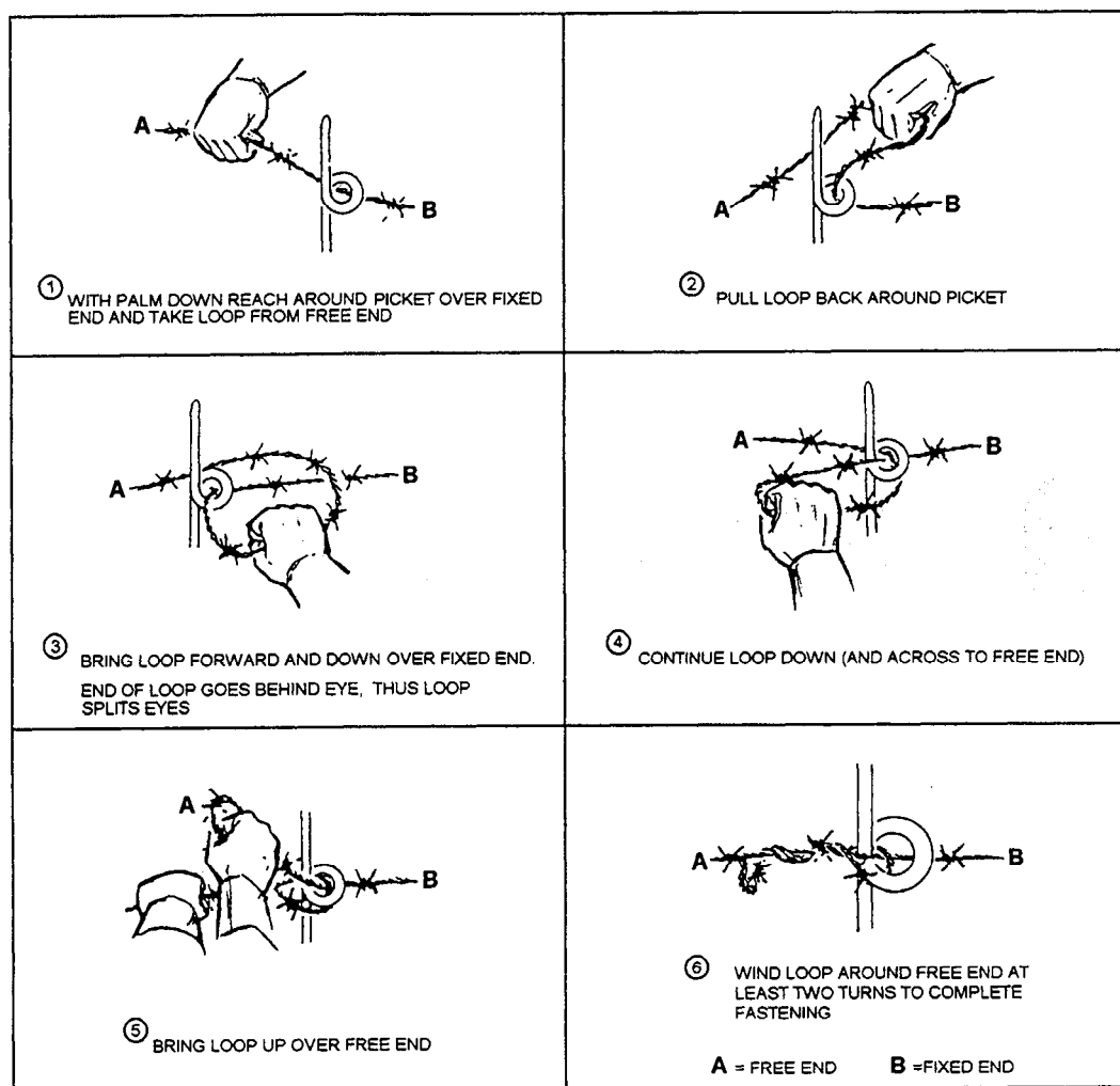
Figure 8-15.—Intermediate-eye tie.
