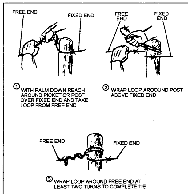
Figure 8-17.—Post tie.
