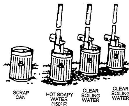
Figure 10-57.—Immersion heaters for mess kit washing setup.
