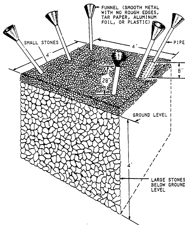
Figure 10-56.—Urinal pipes and soakage pit.
