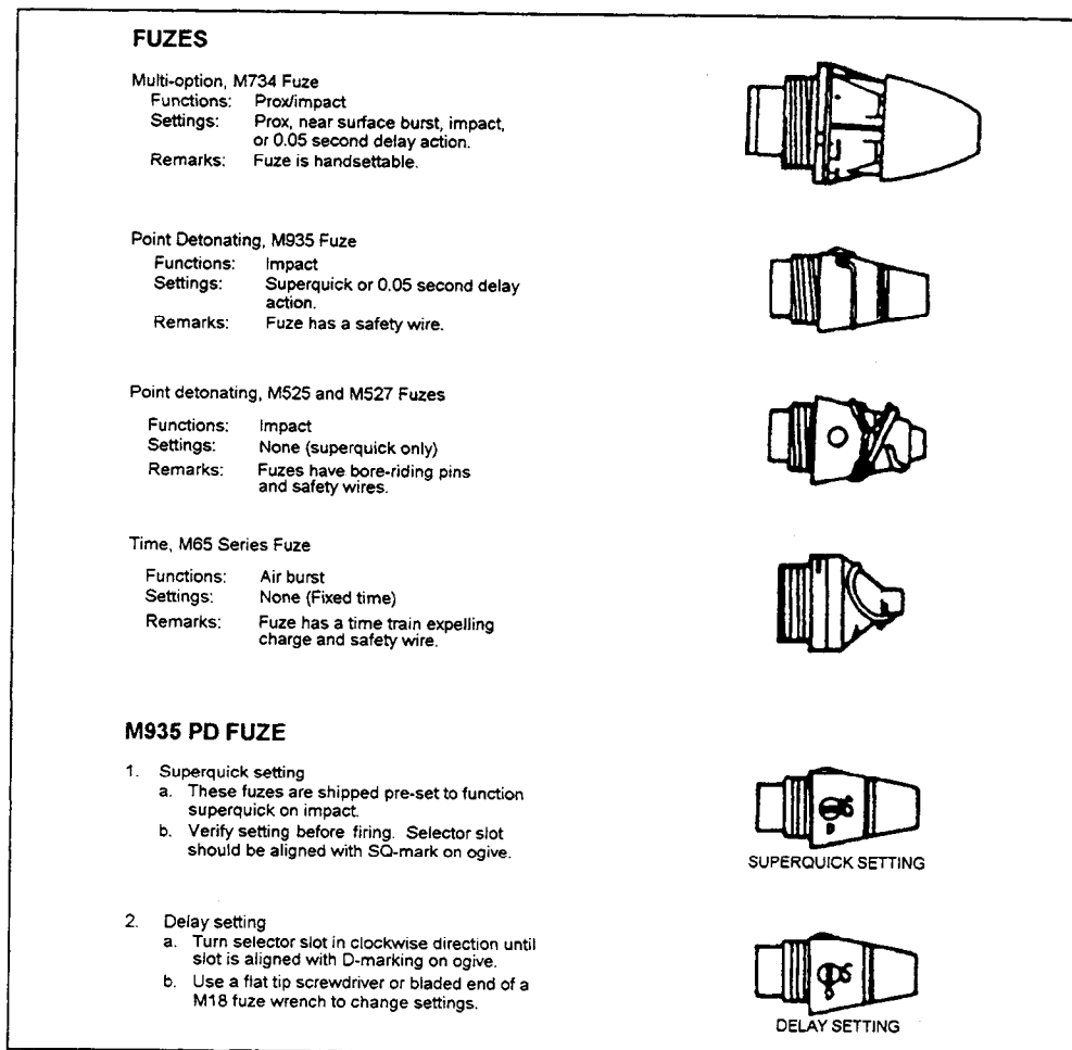
Figure 14-11.—Fuzes.
