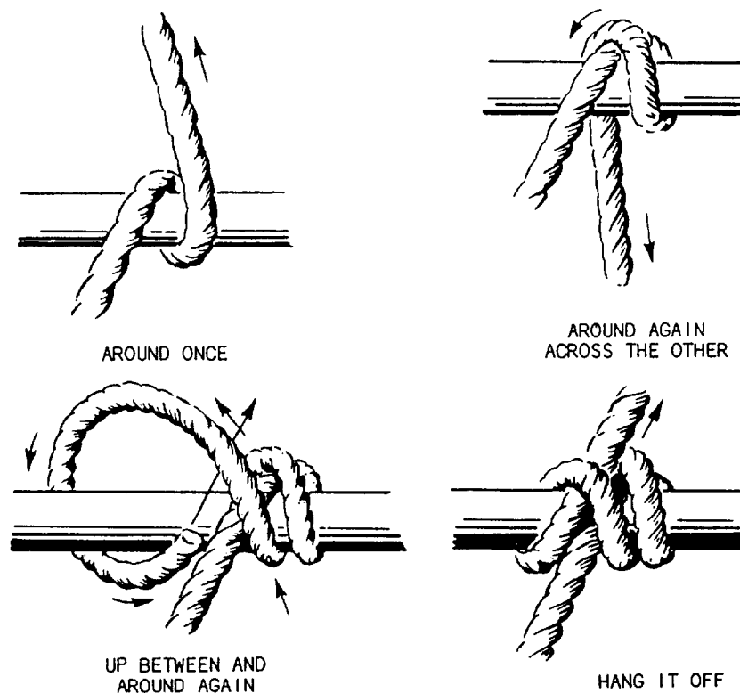
Figure 3-21.—Stopper hitch.
