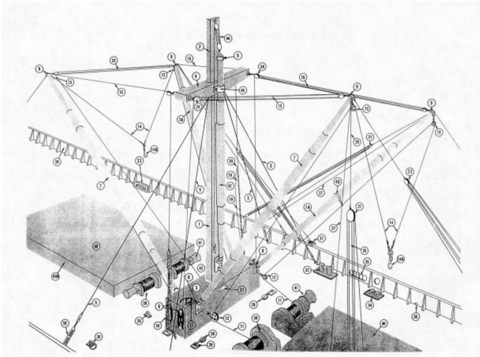
Figure 4-21.-Yard-and-stay rig.
