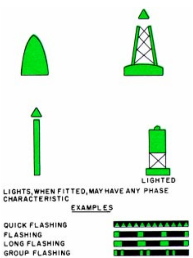
Figure 5-22.—IALA Maritime Buoyage System, International Buoyage Region A starboard-hand marks (buoys).
