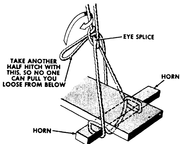
Figure 4-32.—Eye splice rig on a stage.
