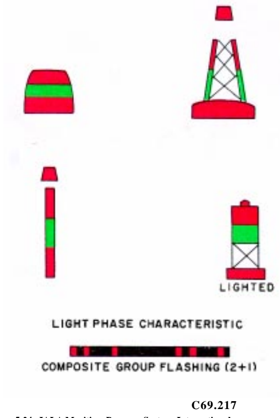
Figure 5-24.—IALA Maritime Buoyage System, International Buoyage Region A preferred channel to starboard.
