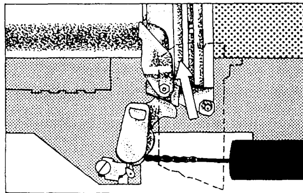
Figure 6-11.—The sliding-wedge breechblock.
