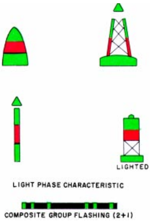
Figure 5-23.—IALA Maritime Buoyage System, International Buoyage Region A preferred channel to port.
