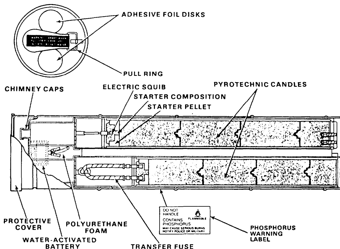
Figure 6-6.—The Mk 58 Mod 1 marine location marker.
