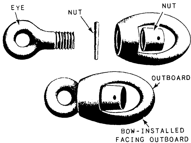
Figure 4-3.—Chain swivel.
