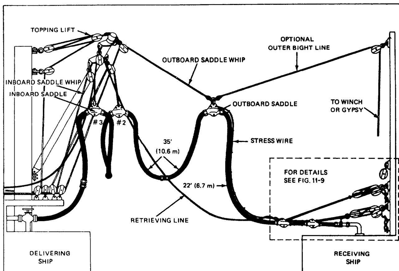
Figure 4-28.—Close-in rig.
