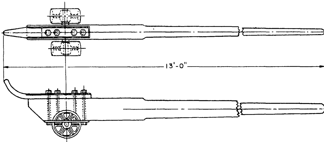
Figure 4-8.—Cable jack.
