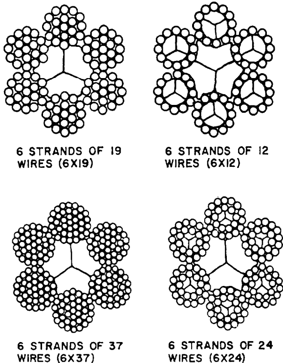
Figure 3-25.—Arrangement of strands in wire rope.
