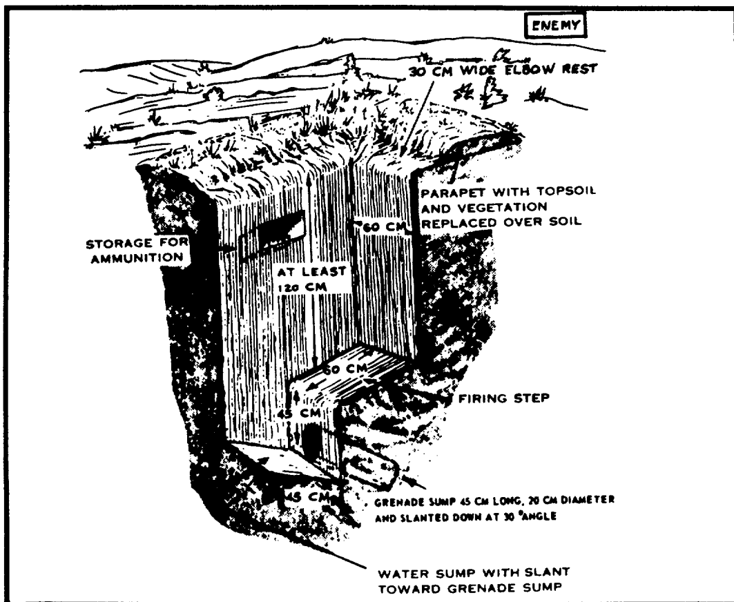
Figure 4-32. Elbow Rest.
