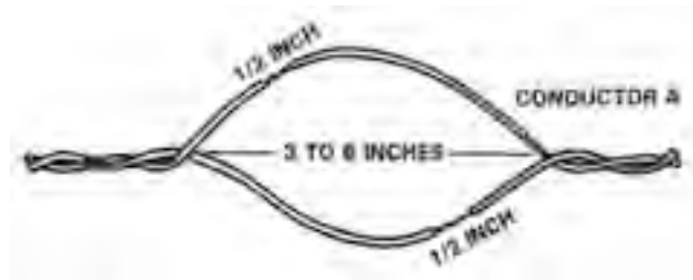
Figure 6-75. Connection of Other Telephones to the Wire Loop.
