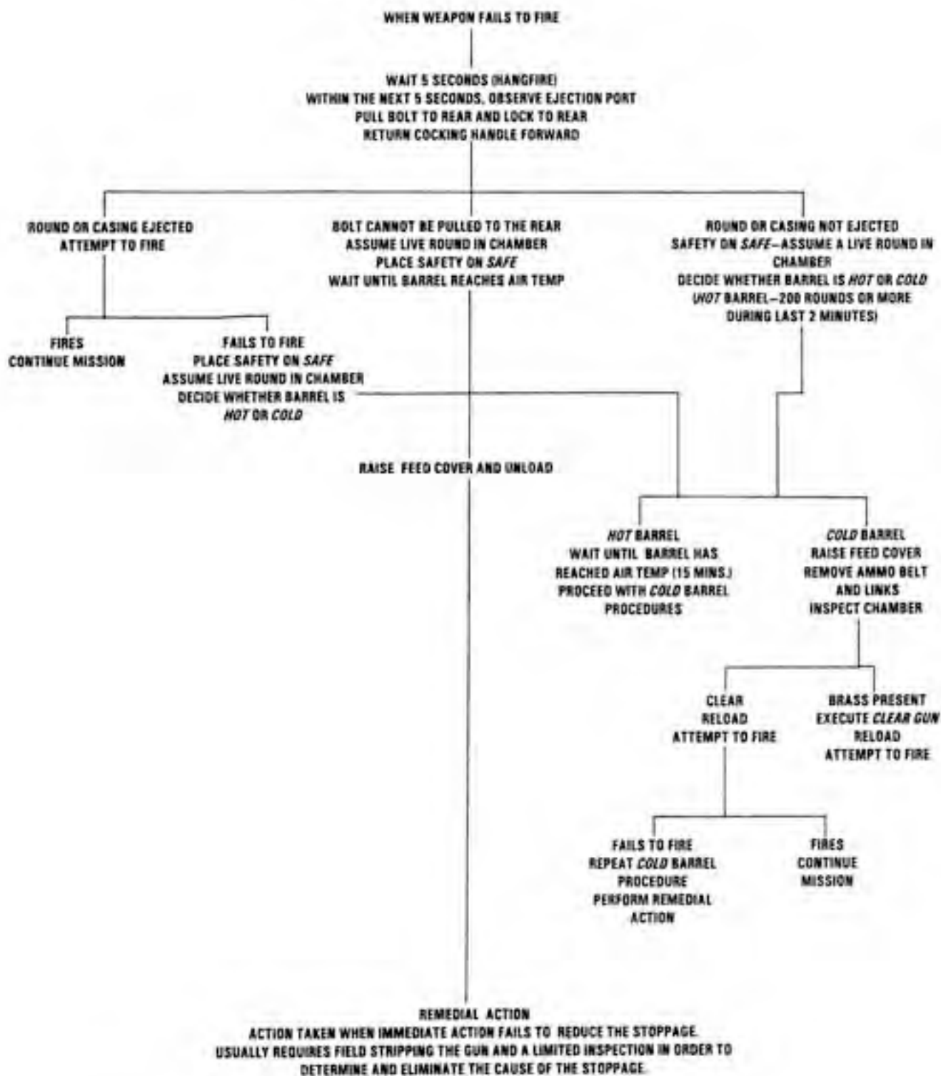
Figure 3-33. Immediate Action.
