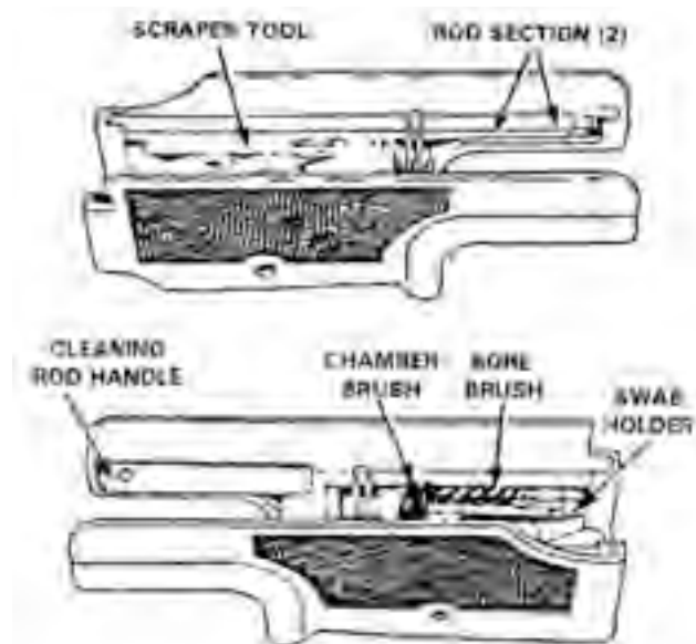
Figure 2-34. SAW Tool Storage.
