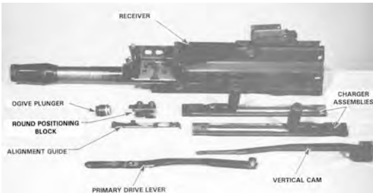
Figure 5-16. Receiver Assembly, Detailed Disassembled.
