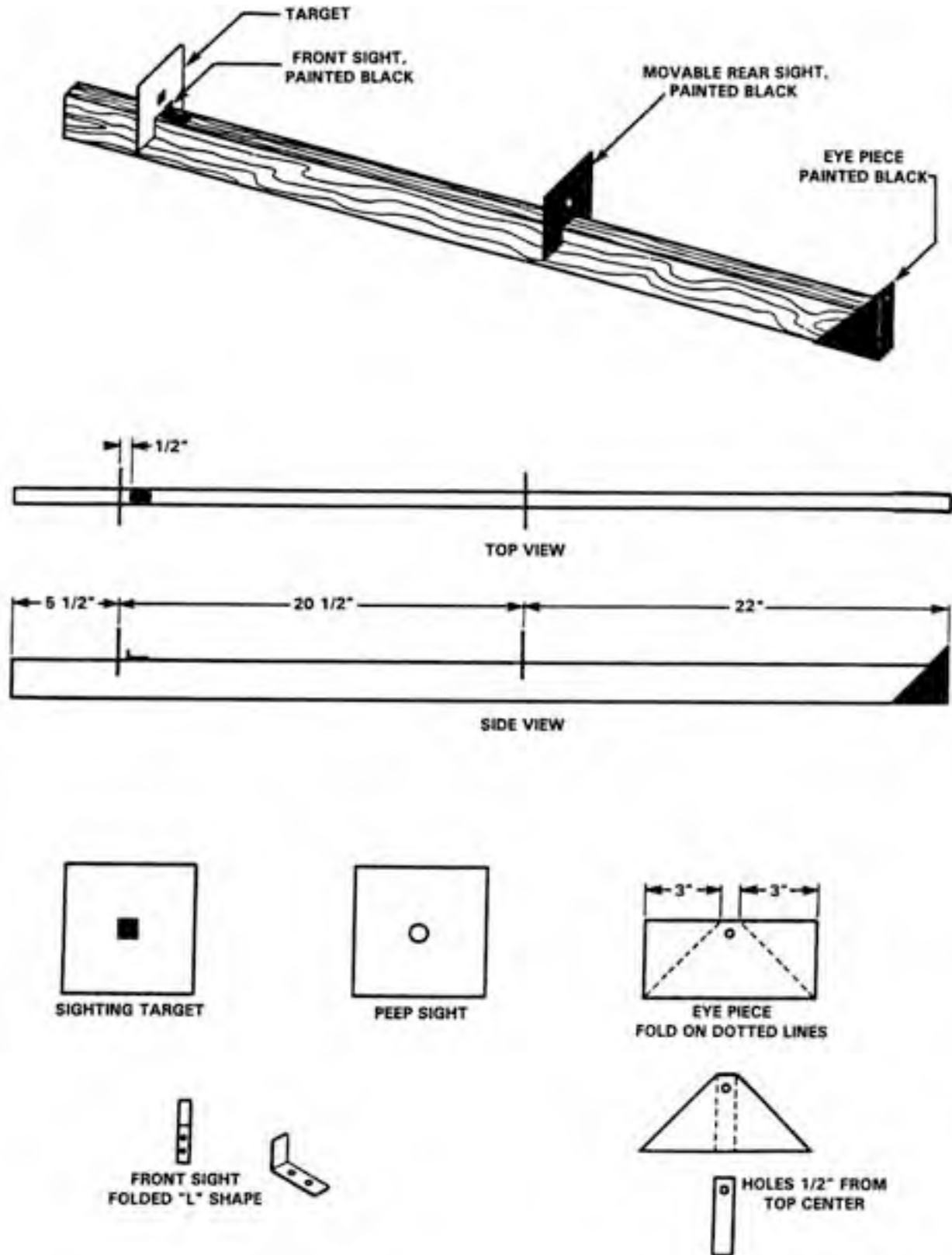
Figure 4-107. Sighting Bar.
