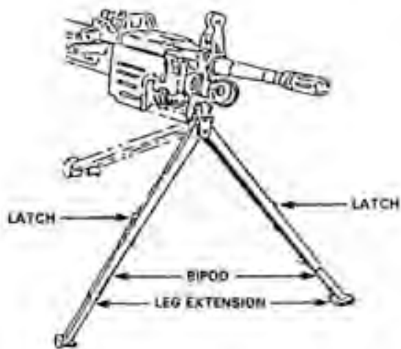
Figure 2-28. Lowering the Bipod.
