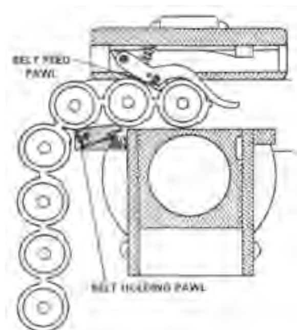
Figure 4-61. Belt Feed Slide Moving Inside the Cover.
