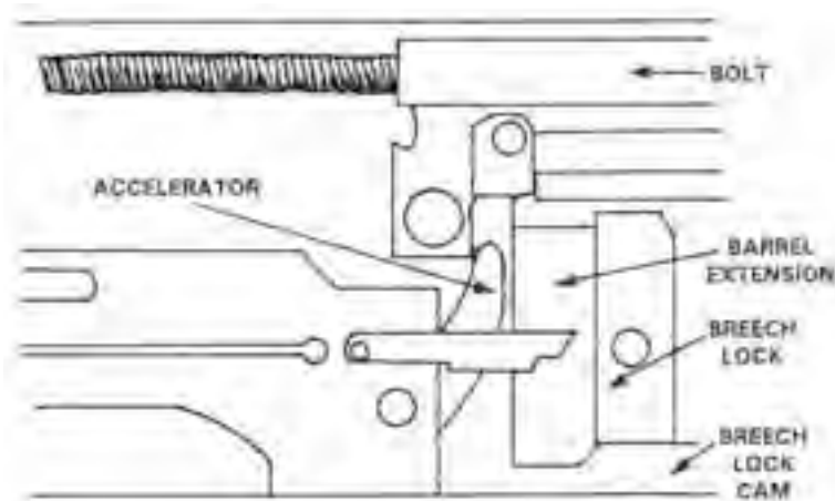
Figure 4-63. Locking.
