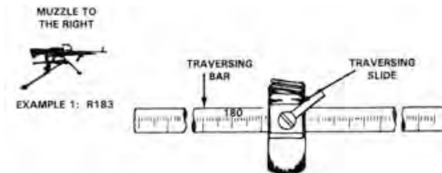
Figure 6-28. Direction Reading.
