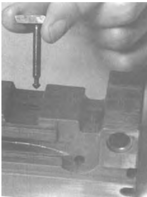
Figure 4-25. Drifting the Sear Stop Pin Free From Engagement with the Firing Pin Spring.
