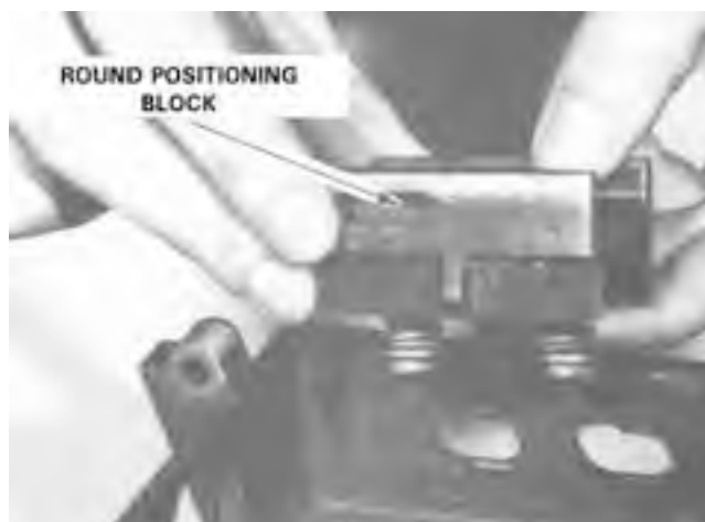
Figure 5-21. Removing of Round Positioning Block.
