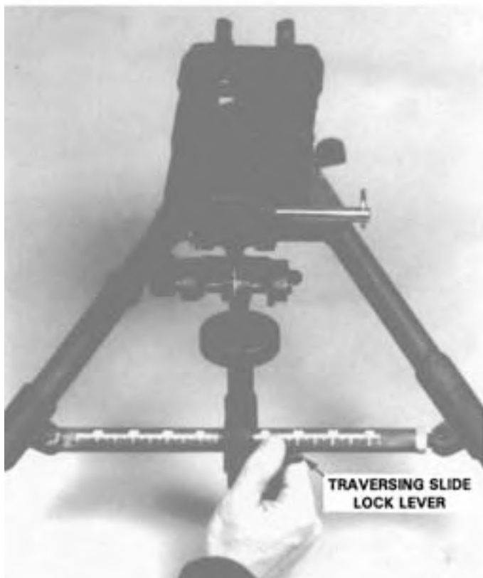
Figure 3-42. Attaching the Flex-mount to the Tripod—Continued.
