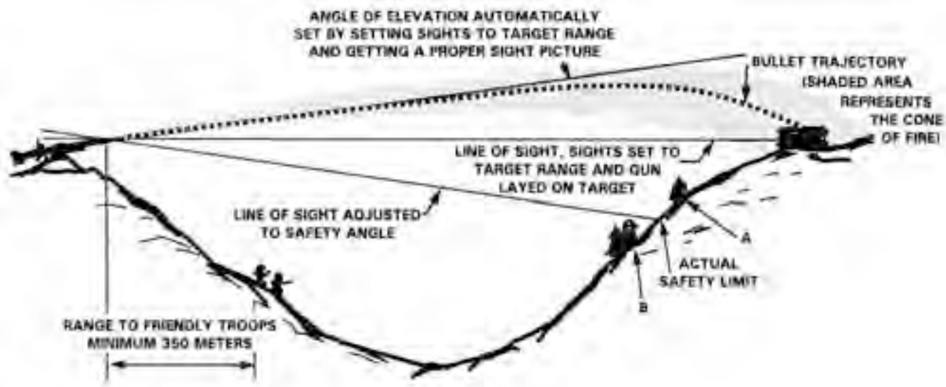
Figure 6-26. Leader's Rule.
