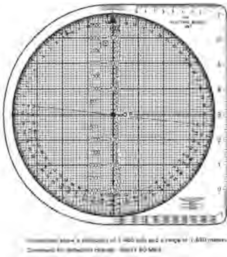
Figure F-5. Deflection Correction.
