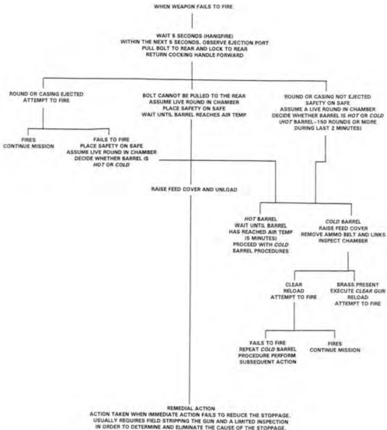
Figure 4-67. Immediate Action.
