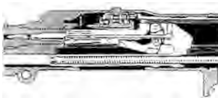
Figure 3-27. Firing.
