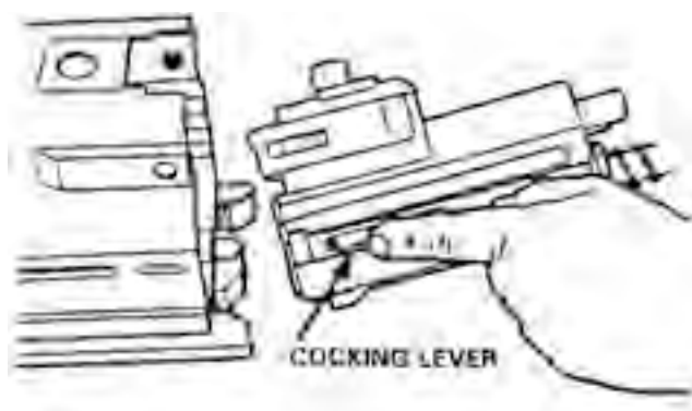
Figure 5-14. Inserting the Bolt and Backplate Assembly Into Receiver.
