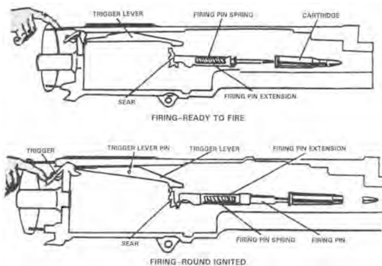
Figure 4-64. Firing.
