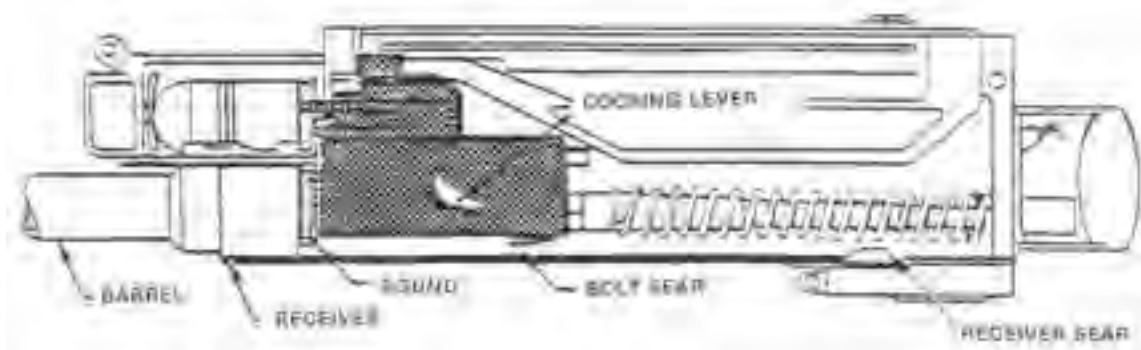
Figure 5-31. Extracting/Ejecting/Feeding/Cocking.
