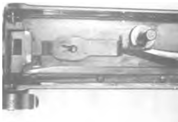
Figure 4-45. Replacing the Cover Latch Spring.
