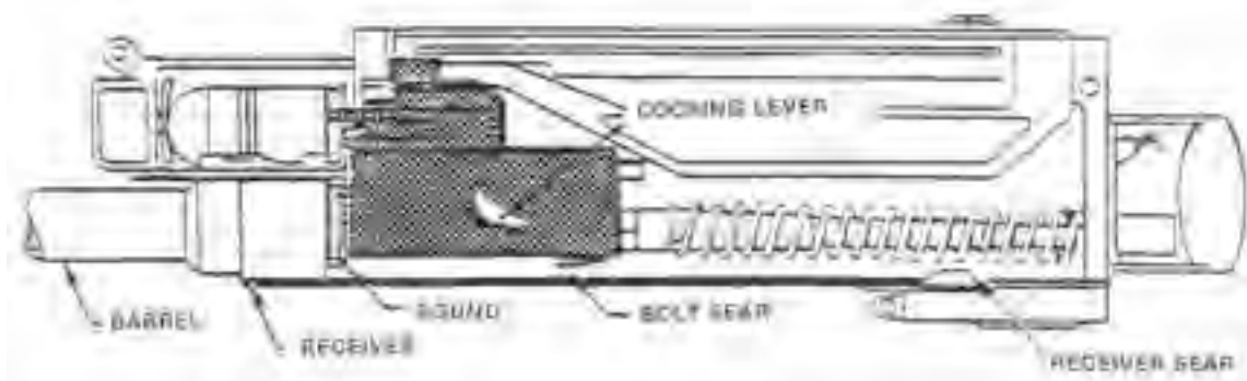
Figure 5-30. Firing/Unlocking.
