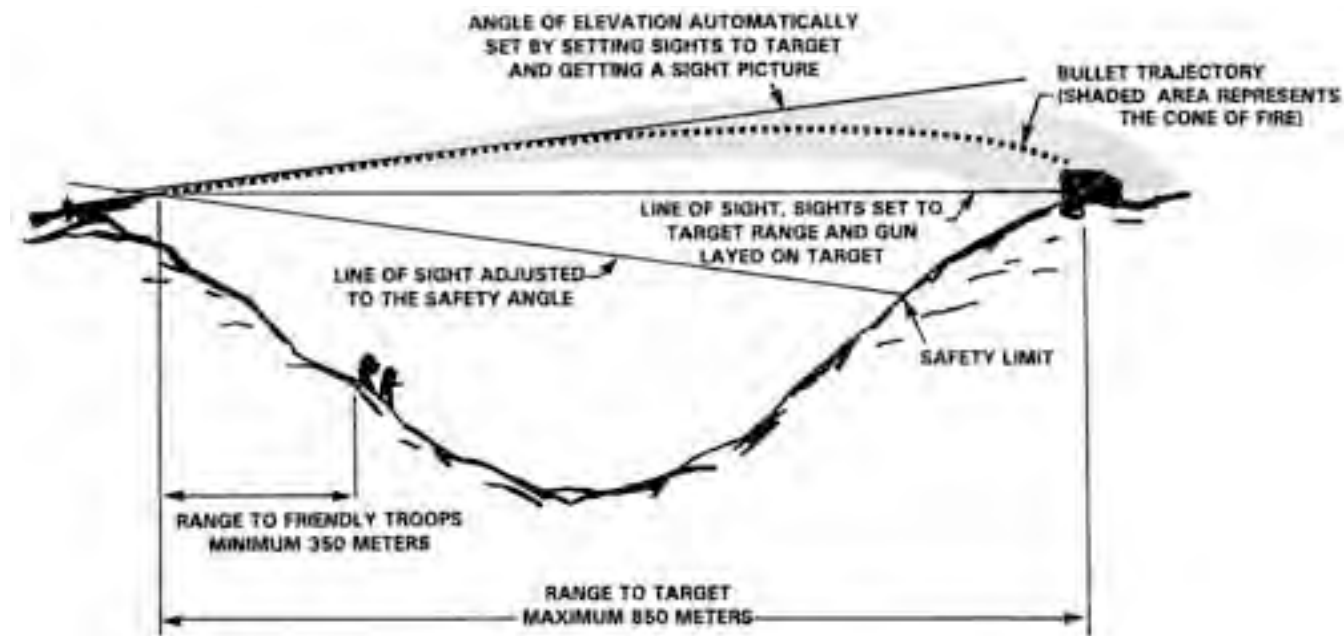
Figure 6-25. Gunner's Rule.
