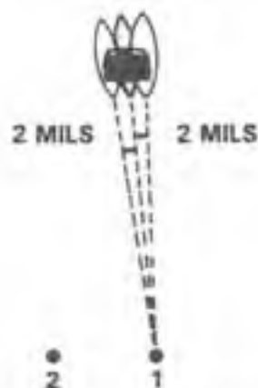
Figure 6-29. Elevation Reading.
