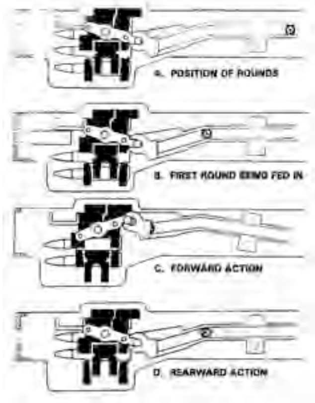
Figure 3-23. Feeding.
