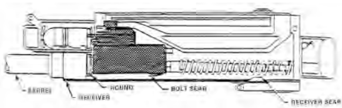
Figure 5-29. Chambering/Locking.
