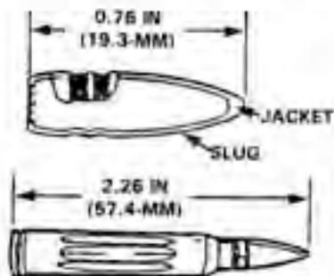
CARTRIDGE, DUMMY, 5.56-MM, M199
