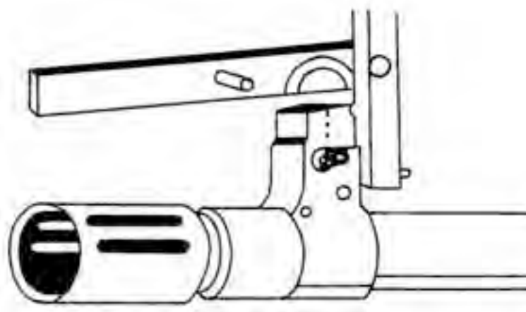
Figure 3-75. Unlocking the Front Sight Retaining Strap.
