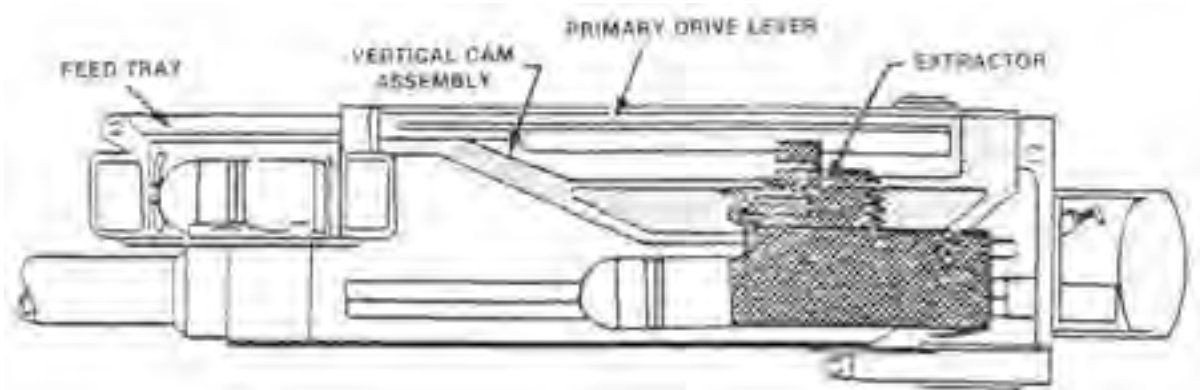
Figure 5-26. Round Cammed Down Onto Face of Bolt.
