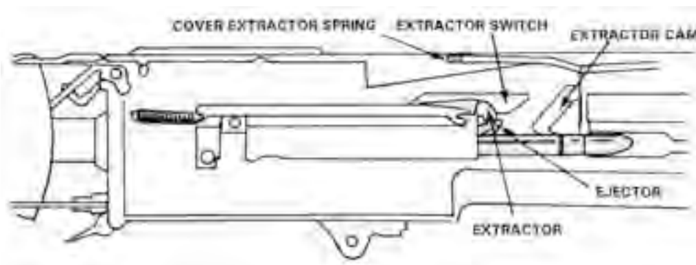
Figure 4-62. Chambering.
