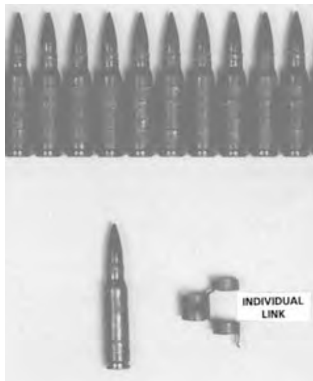
Figure 3-51. Belt of Disintegrating Link Ammunition.
