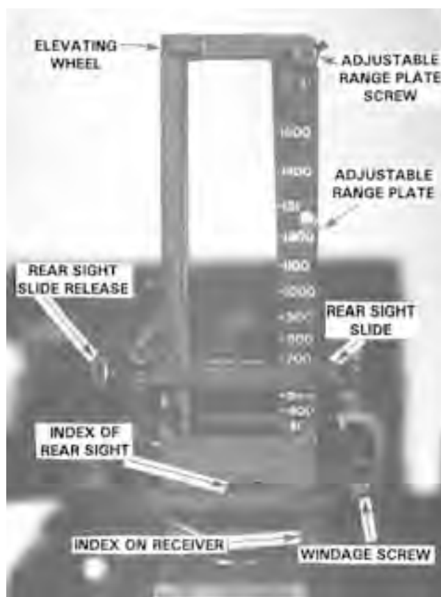
Figure 5-3. Rear Sight.
