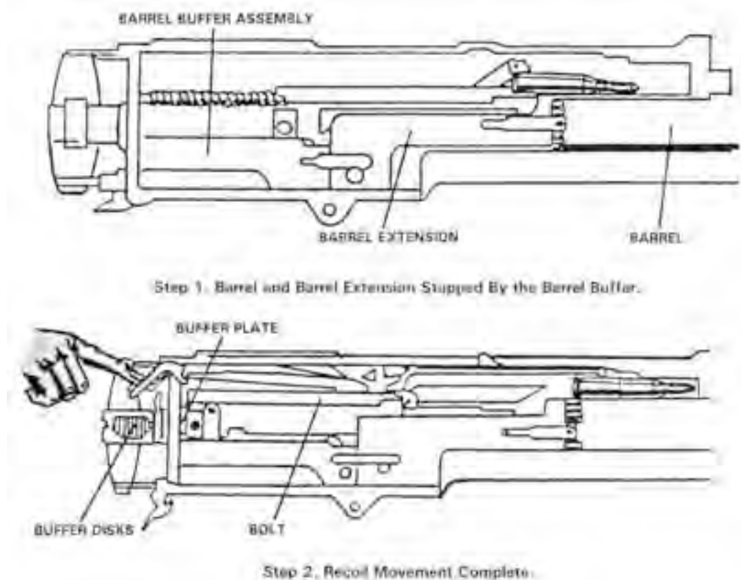
Figure 4-65. Unlocking.
