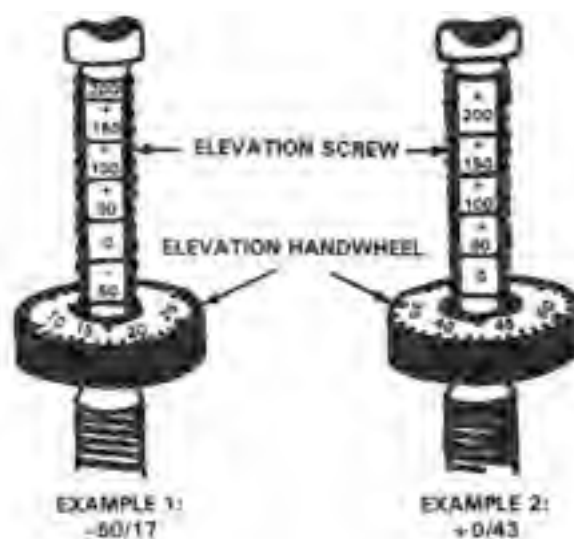
Figure 6-29. Elevation Reading.
