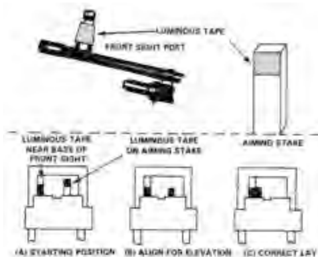
Figure 6-32. Field Expedient—Aiming Stake Method.
