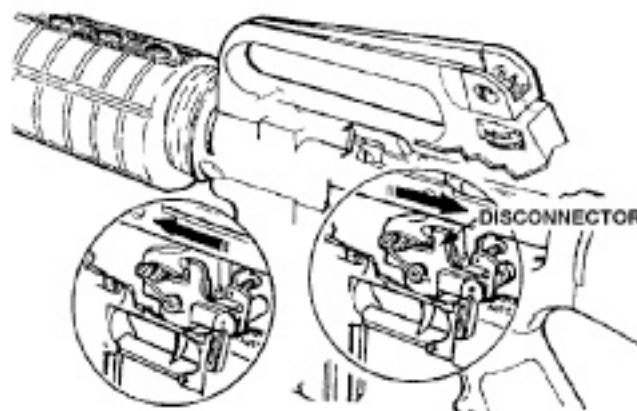
Figure 2-10. Cocking.
