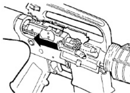
Figure 2-9. Ejecting.
