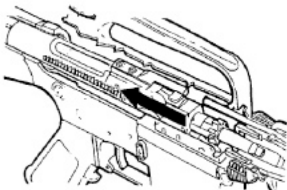
Figure 2-8. Extracting.
