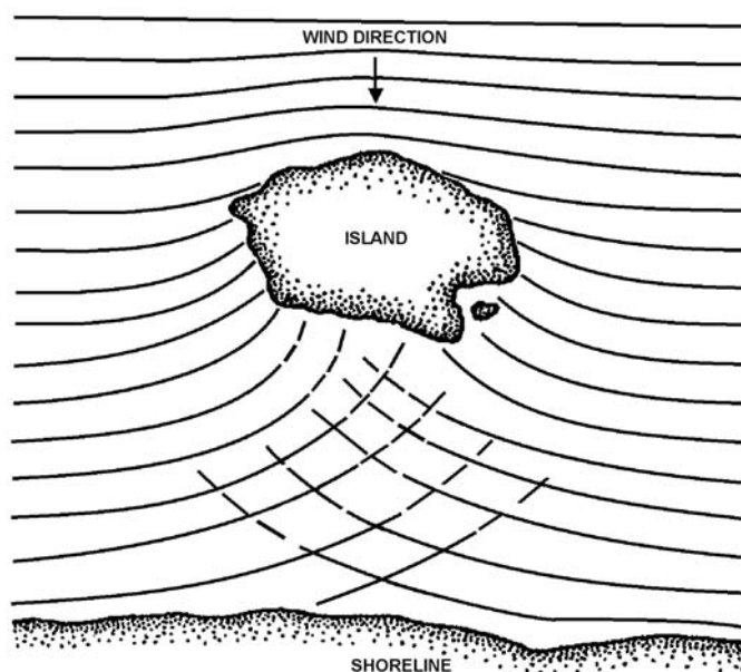
Figure 20-2 Wave Refraction
