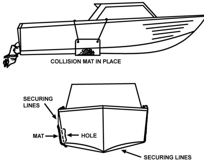
Figure 18-26 Collision Mat
