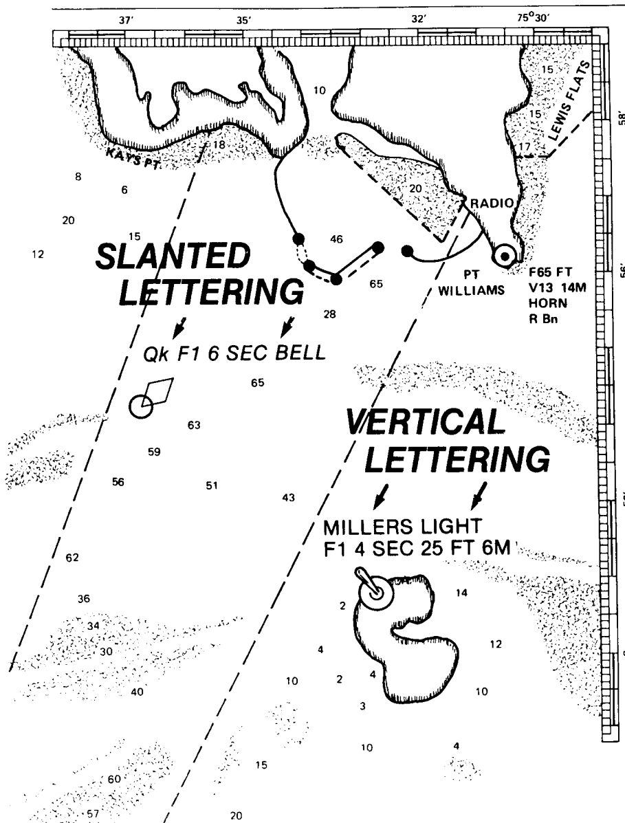
Figure 14-8 Chart Lettering
