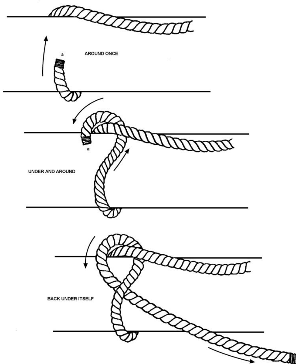
Figure 7-13 Half Hitch
