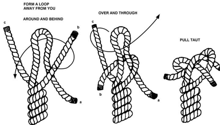
Figure 7-27 Crown Knot
