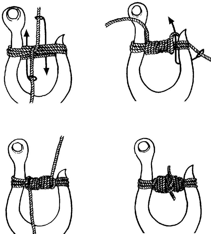
Figure 7-33 Mousing a Hook
