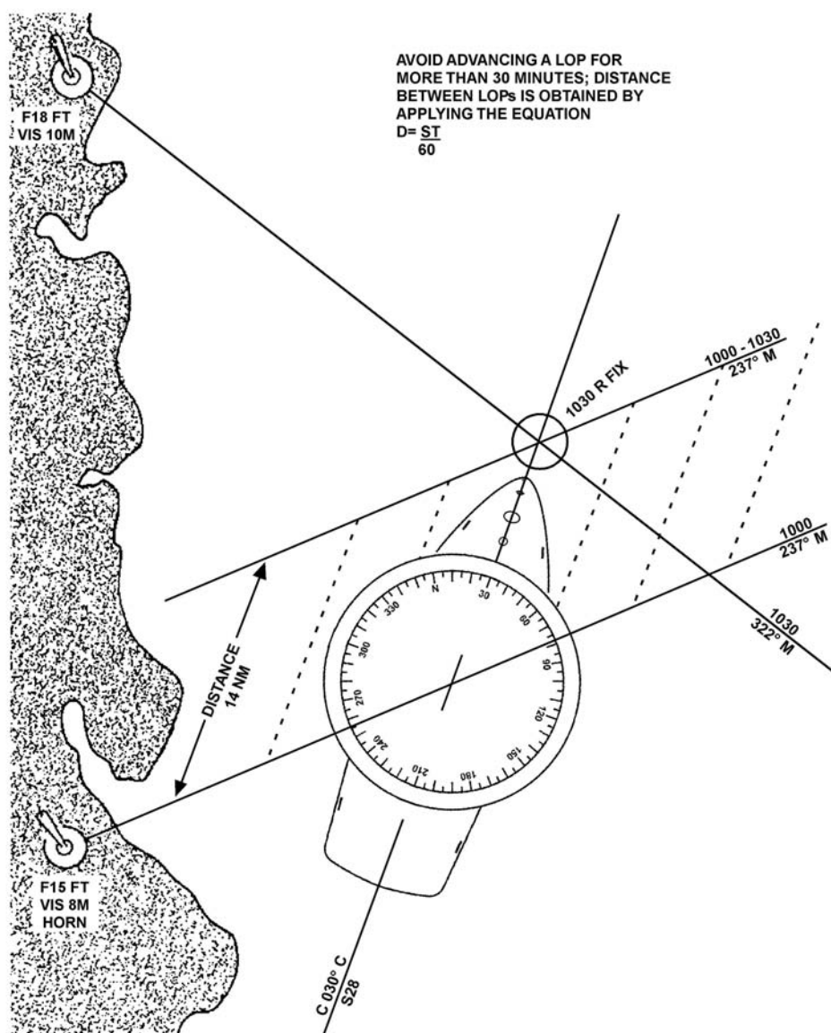
Figure 14-34 Running Fix
