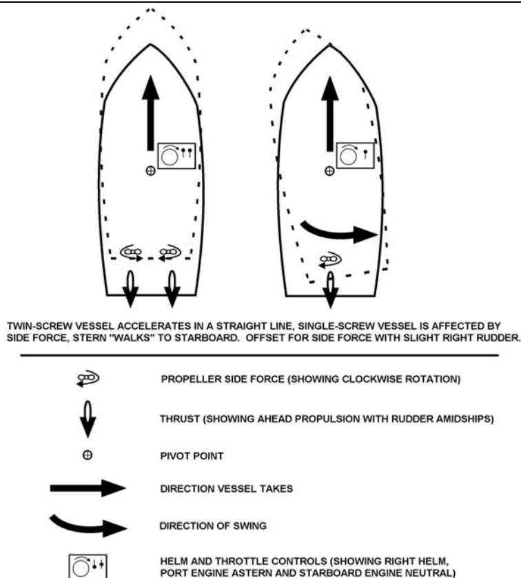
Figure 10-12 Accelerated Ahead
