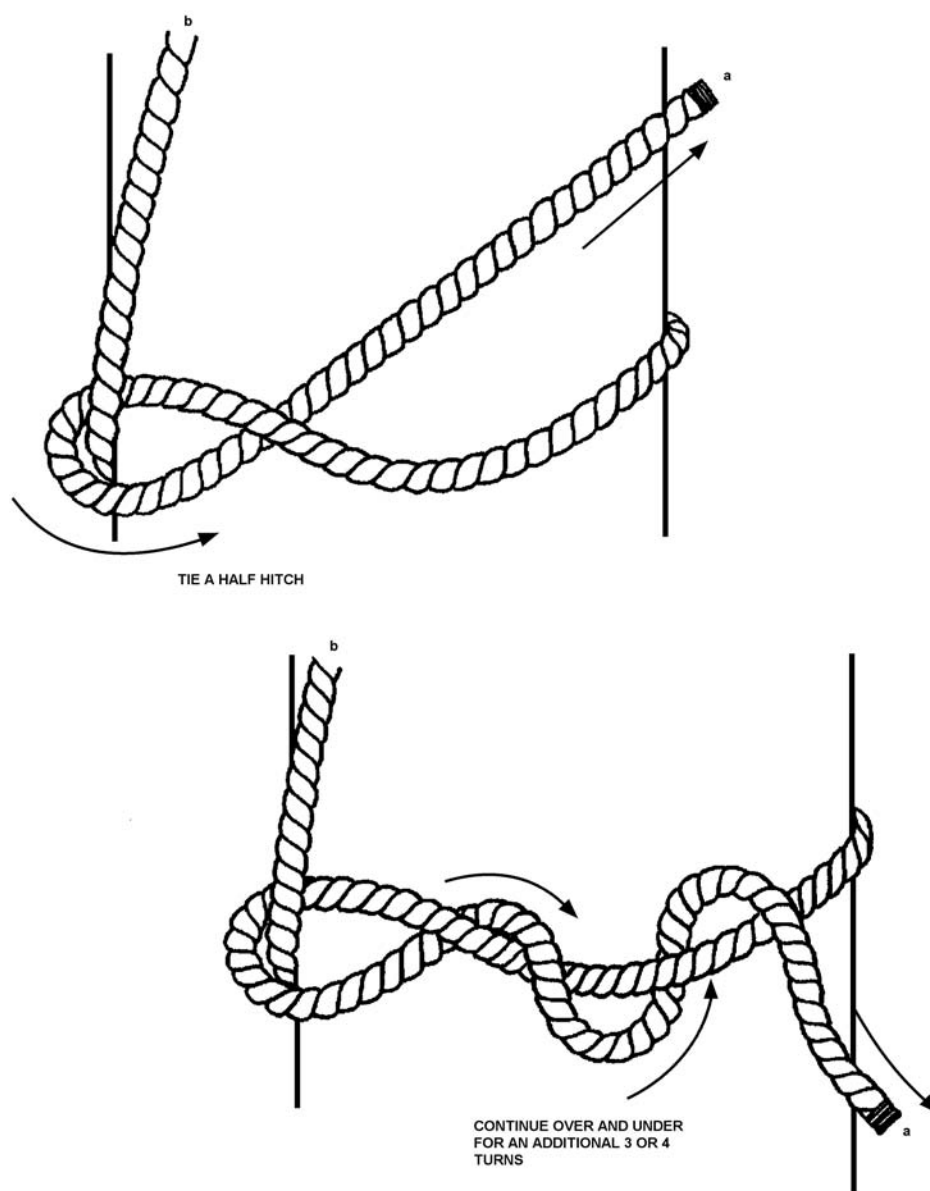
Figure 7-18 Timber Hitch
