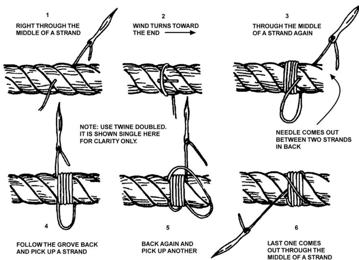
Figure 7-32 Permanent Whipping
