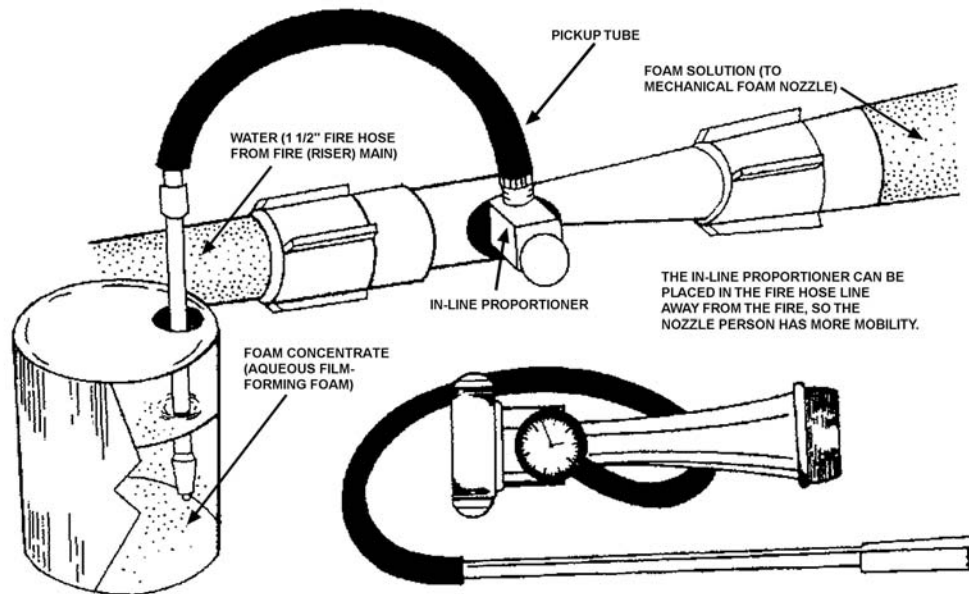
Figure 18-11 In-Line Proportioner
