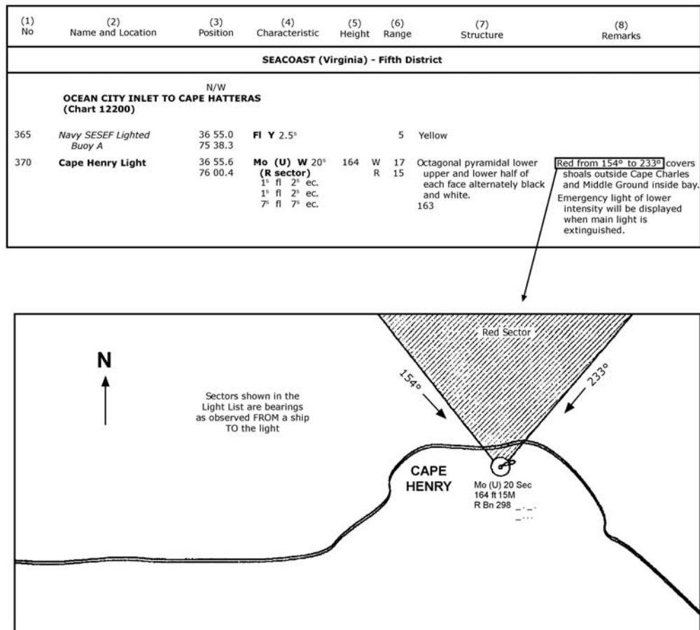
Figure 13-9 Sector Light
