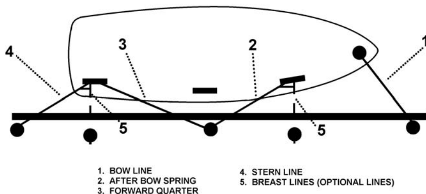
Figure 10-19 Mooring Lines
