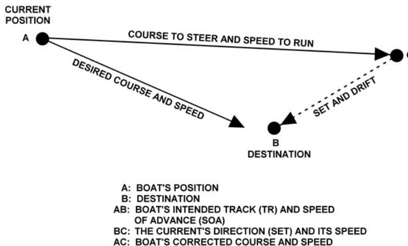
Figure 14-36 Current Triangle
