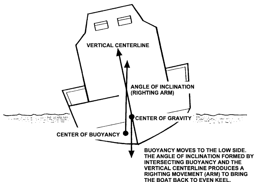
Figure 9-2 Heeling
