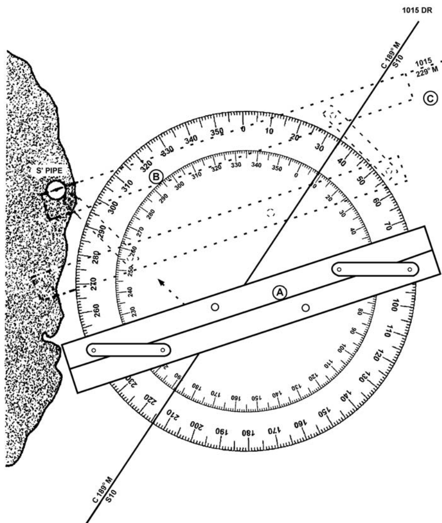
Figure 14-30 Plotting Bearings
