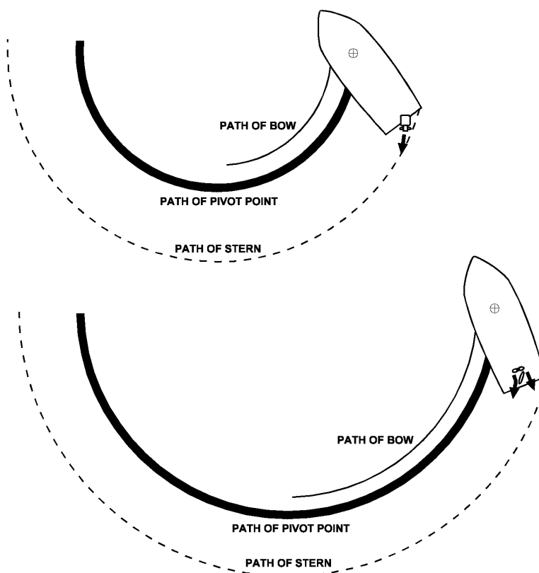
Figure 10-15 Pivot Point, Skid, Kick, Inboard vs. Outboard
