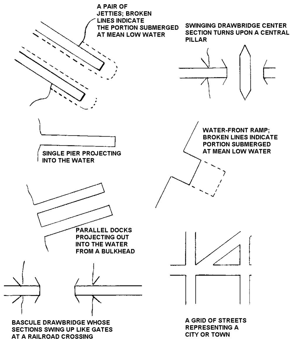
Figure 14-11 Structures
