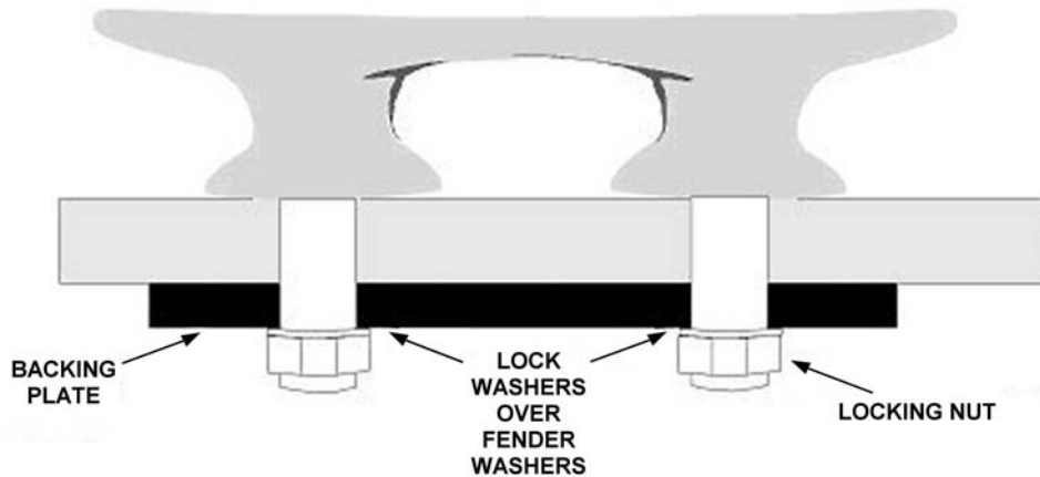
Figure 7-36 Backup Plate
