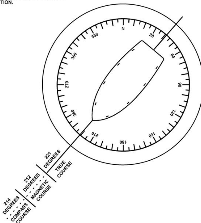
Figure 14-20 Applying Compass Error, Uncorrecting
