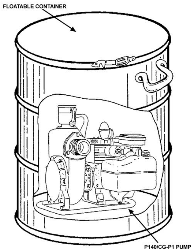
Figure 18-16 Drop Pump
