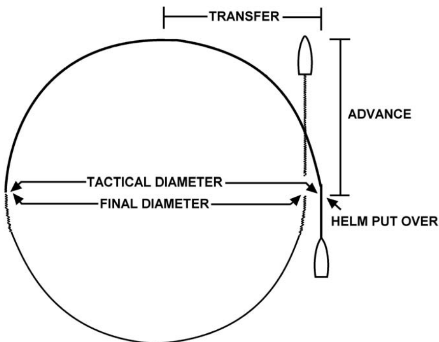
Figure 10-16 Turning Characteristics
