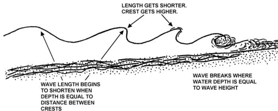
Figure 12-7 Surf
