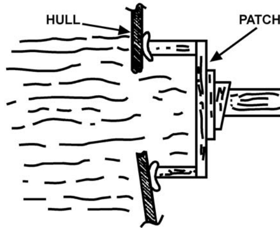
Figure 18-27 Box Patch
