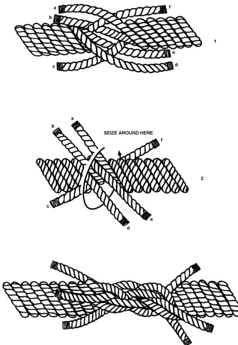
Figure 7-30 Short Splice
