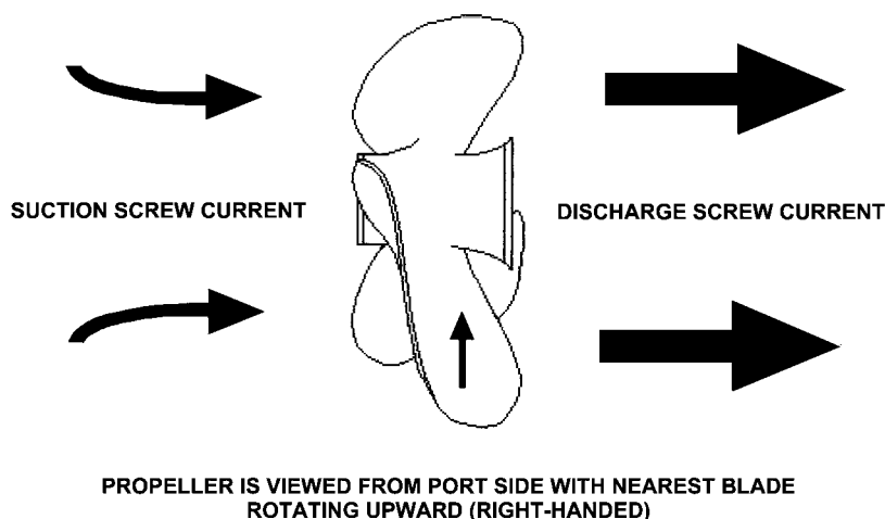
Figure 10-6 Screw Current
