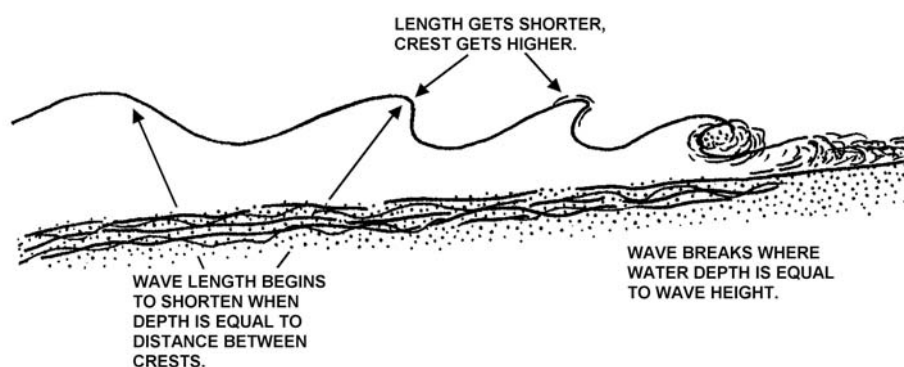
Figure 20-5 Surf
