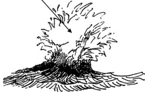
Figure 12-4 Wave Refraction
