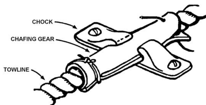
Figure 7-5 Chafing Gear
