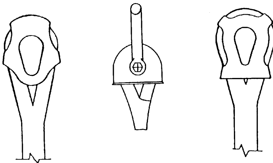
Figure 17-6 Thimbles
