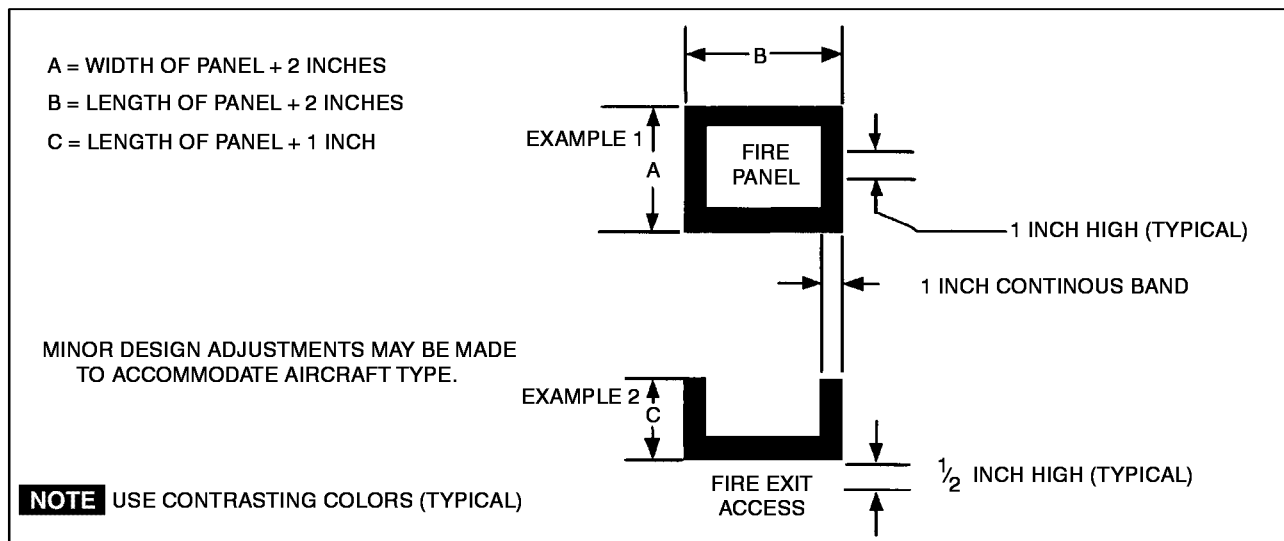
Figure B-9. Markings For Fire Access Panel
