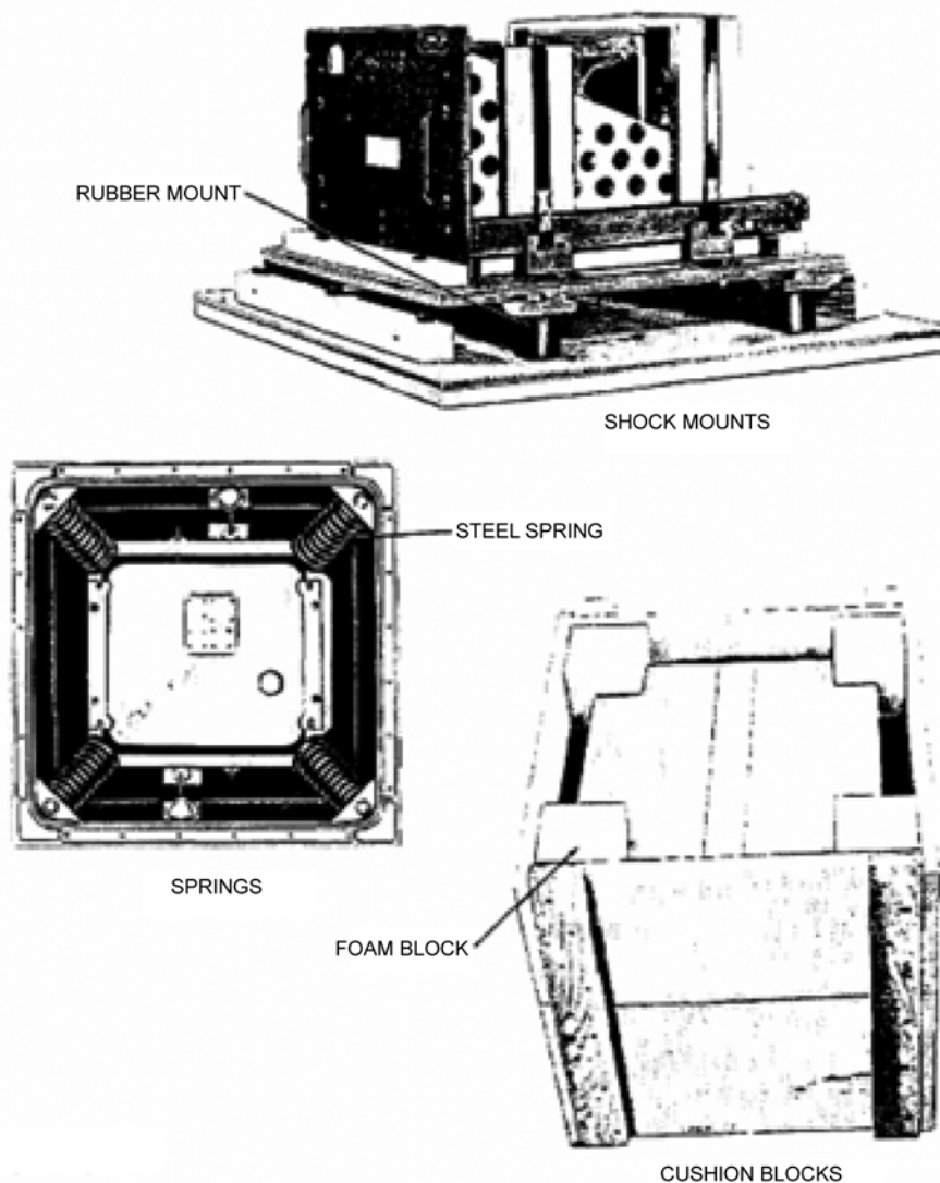
Figure 5-8. Shock Isolators
