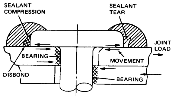
Figure 6-17. Fastener Movement on Oversize Hole
