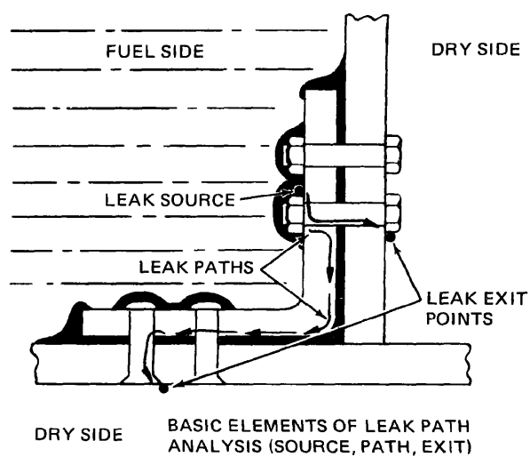
Figure 6-14. Leak Path Analysis
