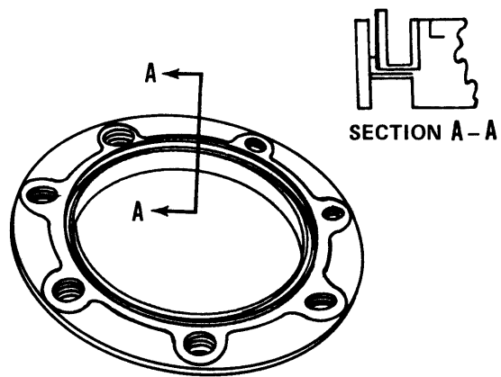
Figure 9-30. Retainer Ring Installation
