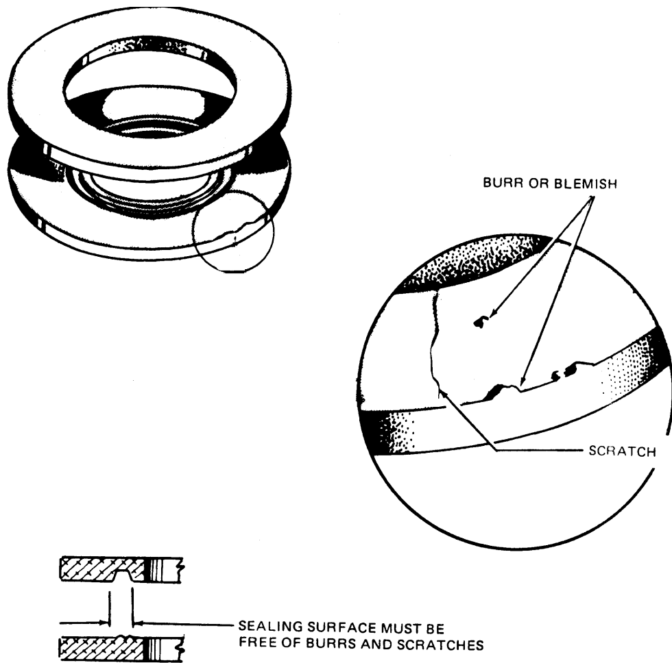
Figure 9-12. O-Ring Fitting Inspection
