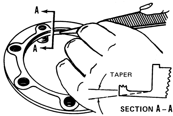
Figure 9-29. Fitting Flange Break
