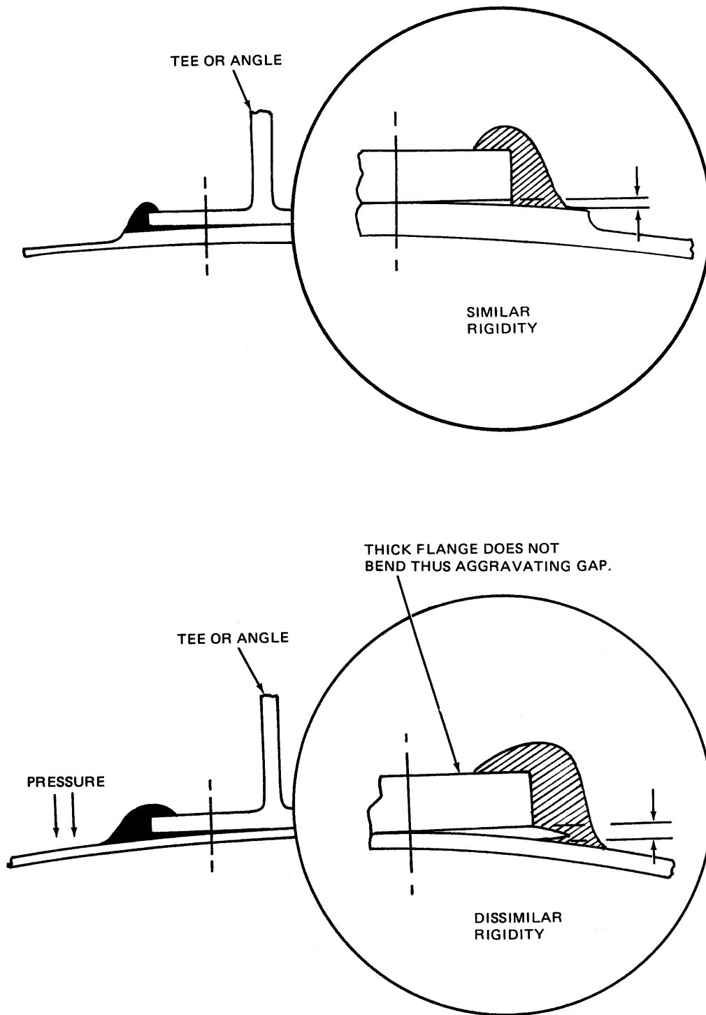
Figure 6-20. Fillet Seal Deflection
