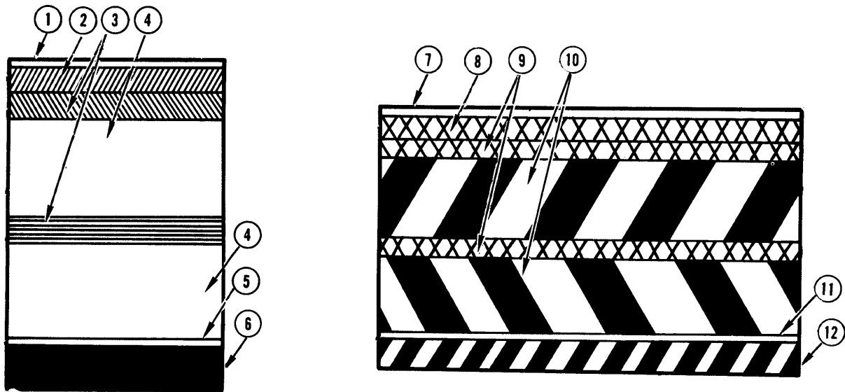
Figure 9-2. Self-Sealing
