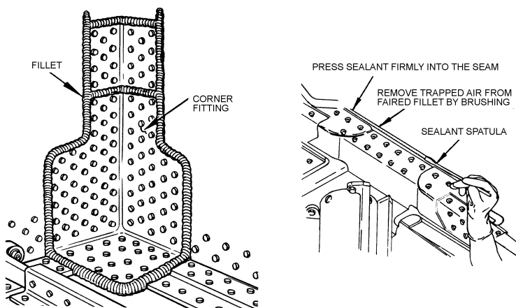
Figure 6-29. Typical Fillet Seals
