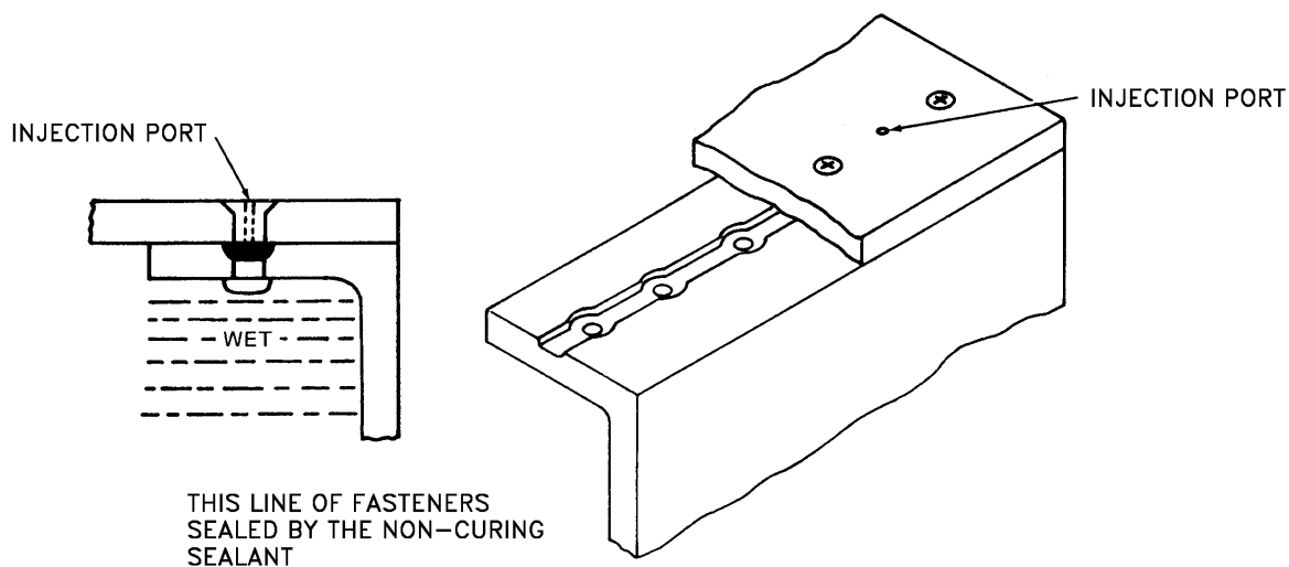
Figure 6-4. Typical Locations of Grooves/Channels (Sheet 2)
