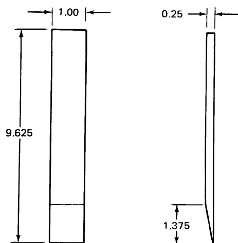
Figure 8-7. Typical Hand Scraper
