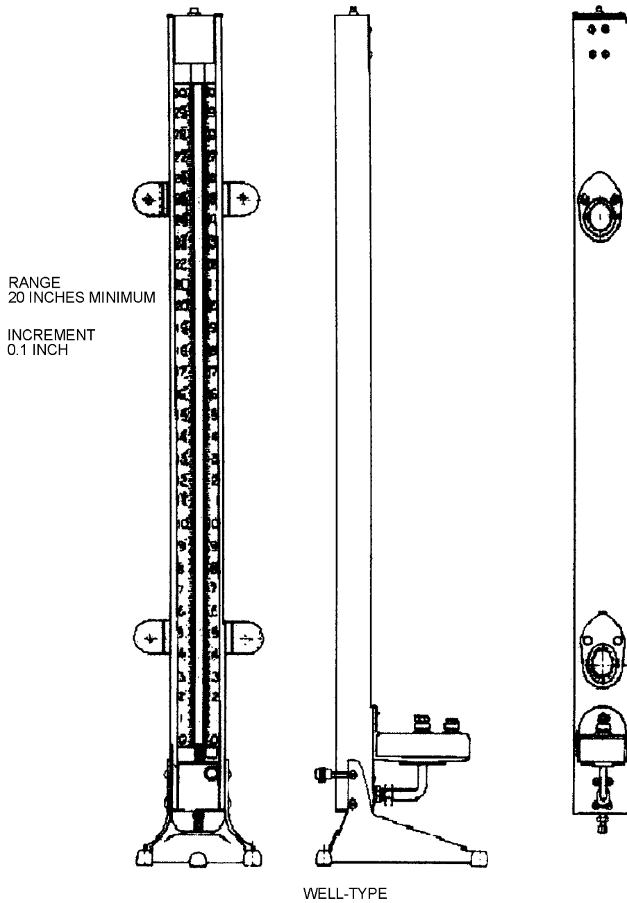
Figure 8-5. Typical Well-Type Manometer
