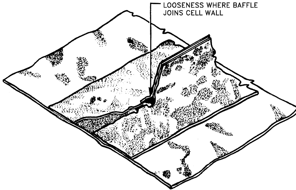
Figure 9-7. Loose Baffles
