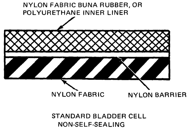
Figure 9-4. Non-Self-Sealing Construction
