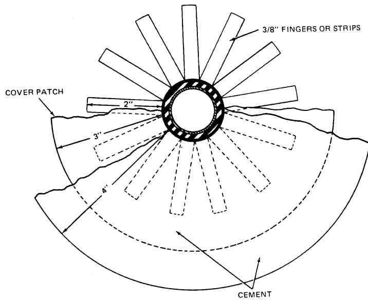
Figure 9-28. Wrap Application
