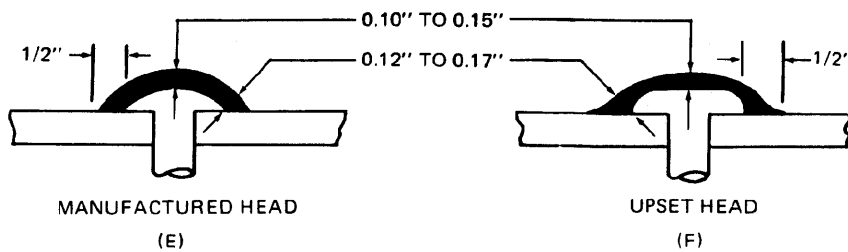
Figure 6-30. Typical Fillet Dimensions
