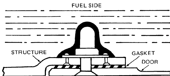
Figure 6-8. Flat Gasket Seal
