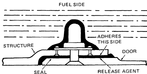
Figure 6-10. Formed-In-Place Seal
