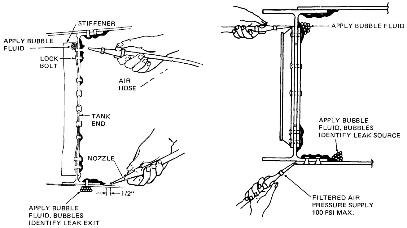
Figure 6-22. Blow Back Method
