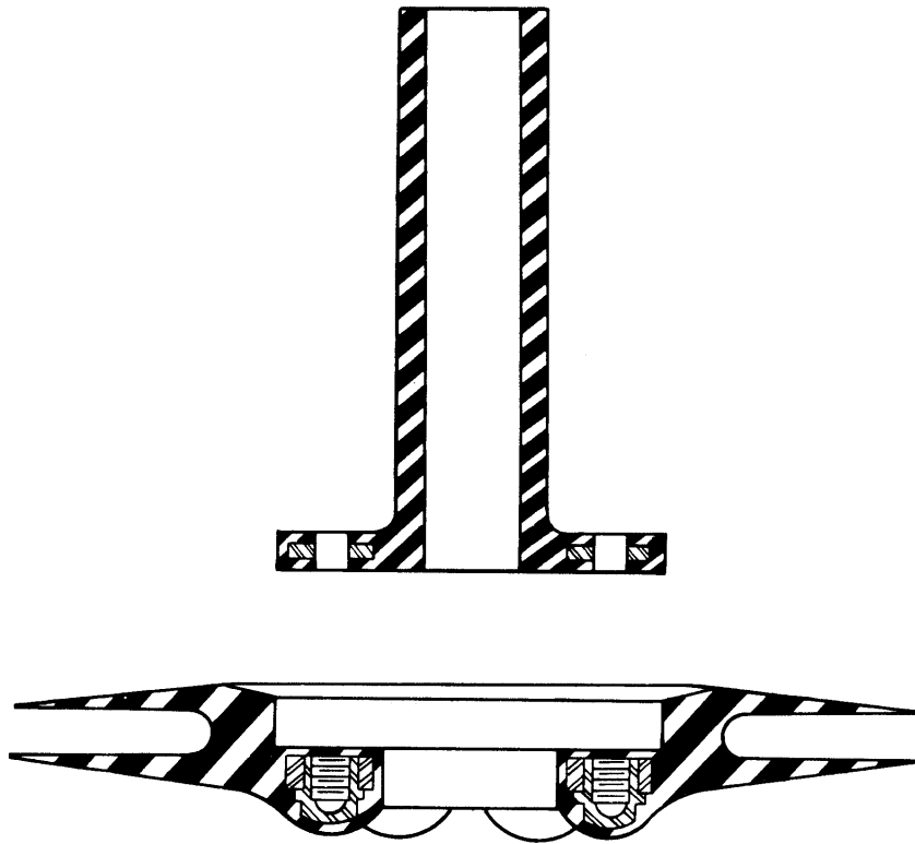
Figure 9-27. Two-Phase Fitting
