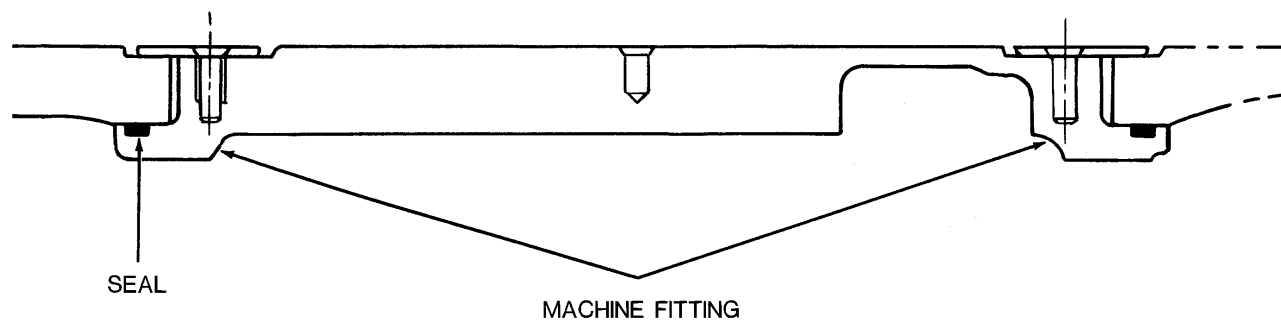
Figure 6-13. Machine Fitted Plug-Type Access Door for Attaching
