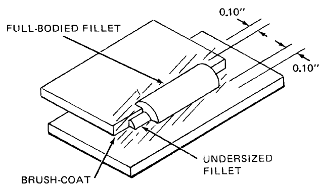
Figure 6-28. Two Bead Fillet
