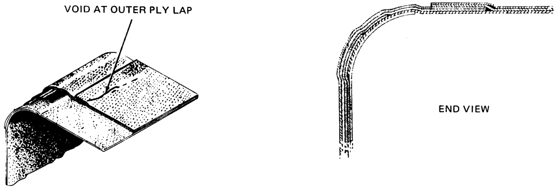
Figure 9-11. Lap Channels
