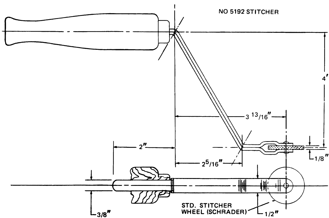
Figure 8-8. Stitcher Horizontal
