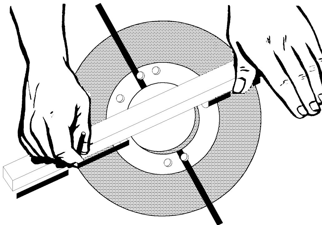
Figure 9-31. Locating Fitting
