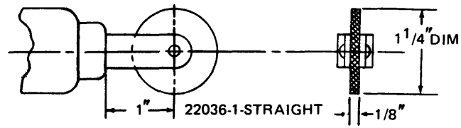
Figure 8-9. Stitcher Roller
