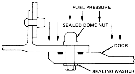
Figure 6-7. Direct Seal Door
