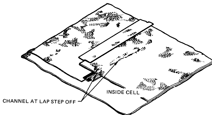
Figure 9-9. Channel at Lap Steps
