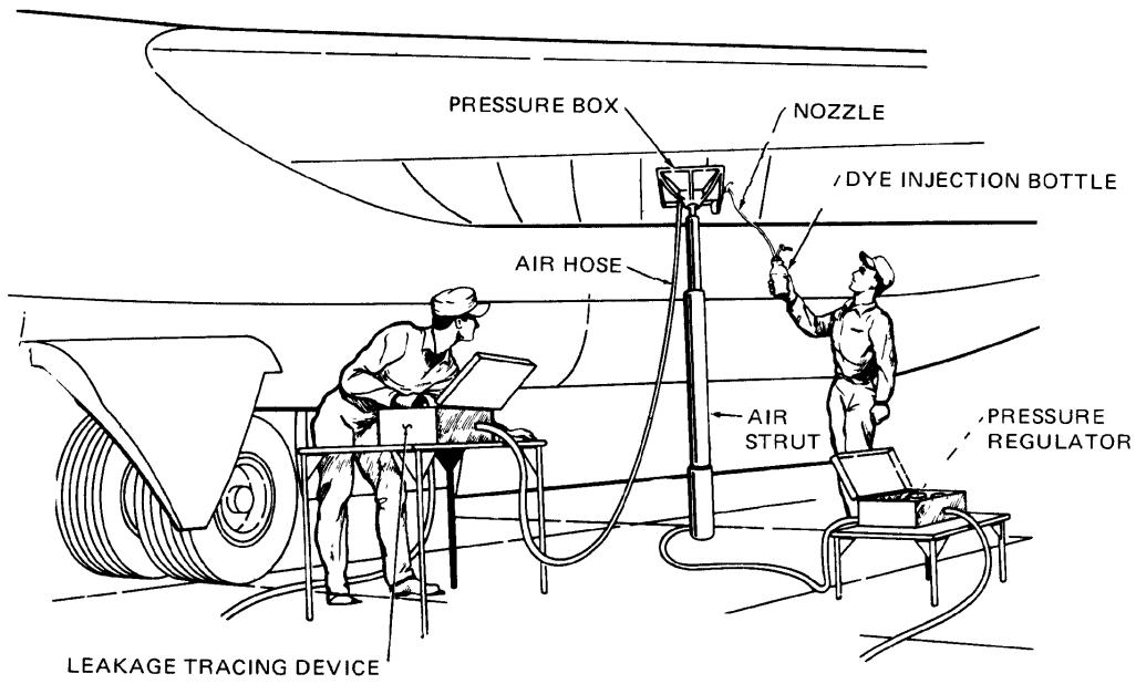
Figure 6-24. Use of Pressure Box for Dye Injection
