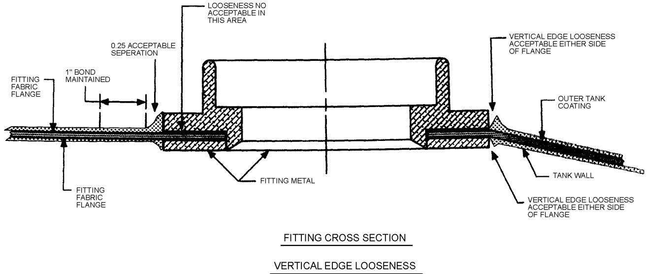
Figure 9-5. Separation of Cell Wall From Fitting Fabric Flange
