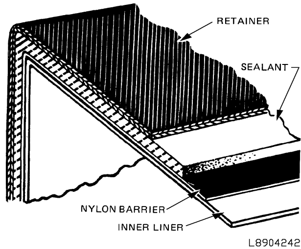
Figure 9-2. Self-Sealing
