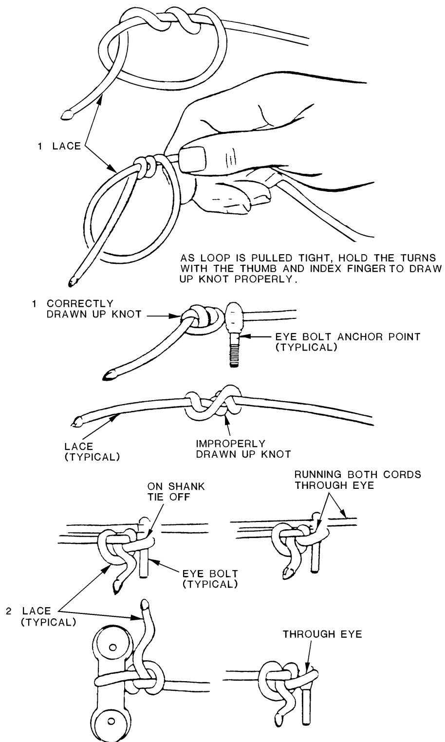
Figure 9-35. Lacing Cord Knots
