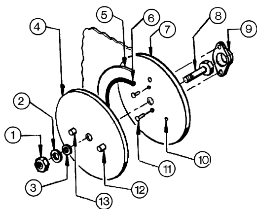
Figure 9-32. Fuel Cell Fitting Leak Test Cover Plate
