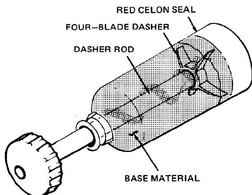
Figure 6-25. Hand Mixing of Sealant Kit
