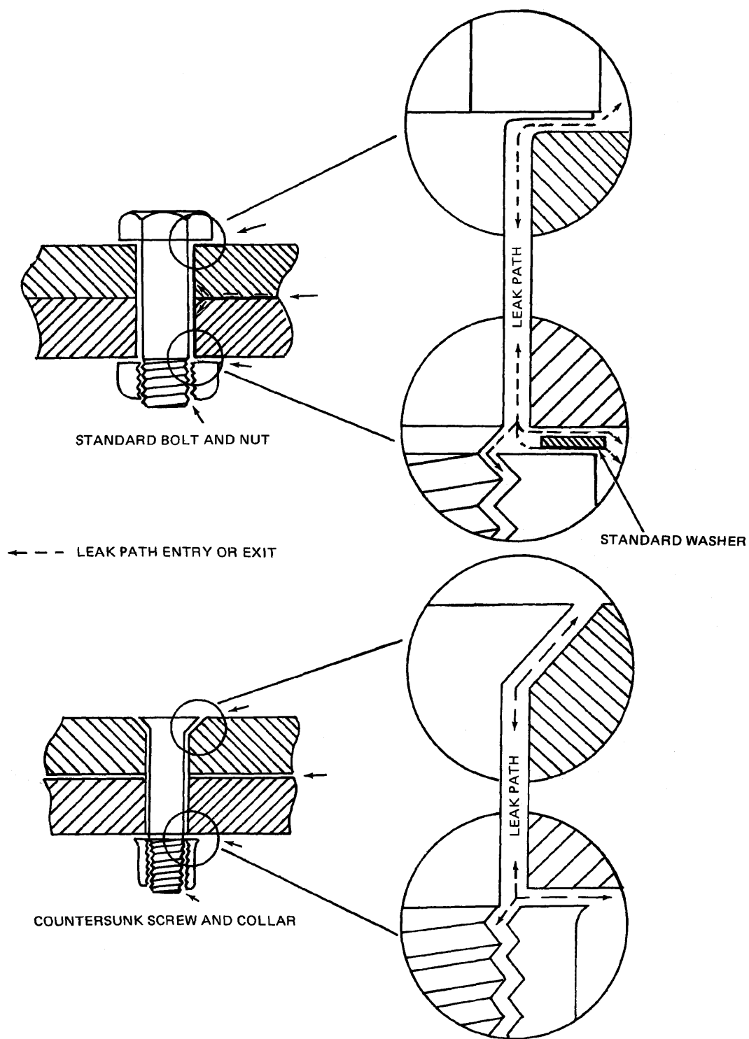
Figure 6-15. Fasteners Leaks
