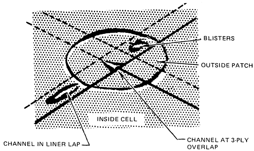
Figure 9-8. Loose Patches
