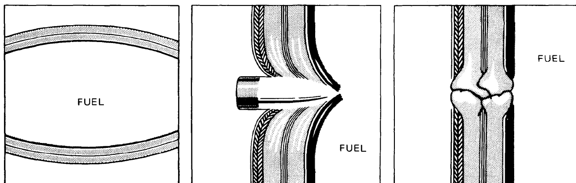
Figure 9-1. Projectile Sealing Action
