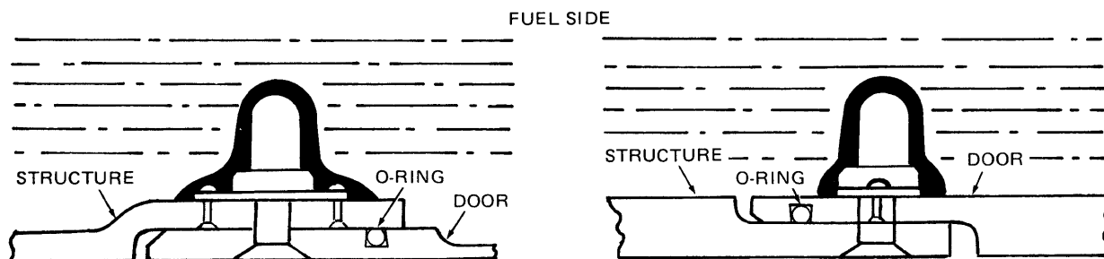
Figure 6-9. O-Ring Seal
