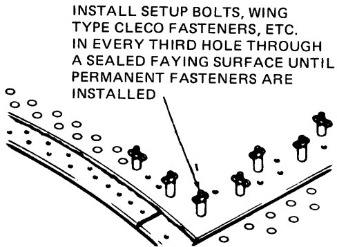
Figure 6-32. Faying Surface Seal Assembly
