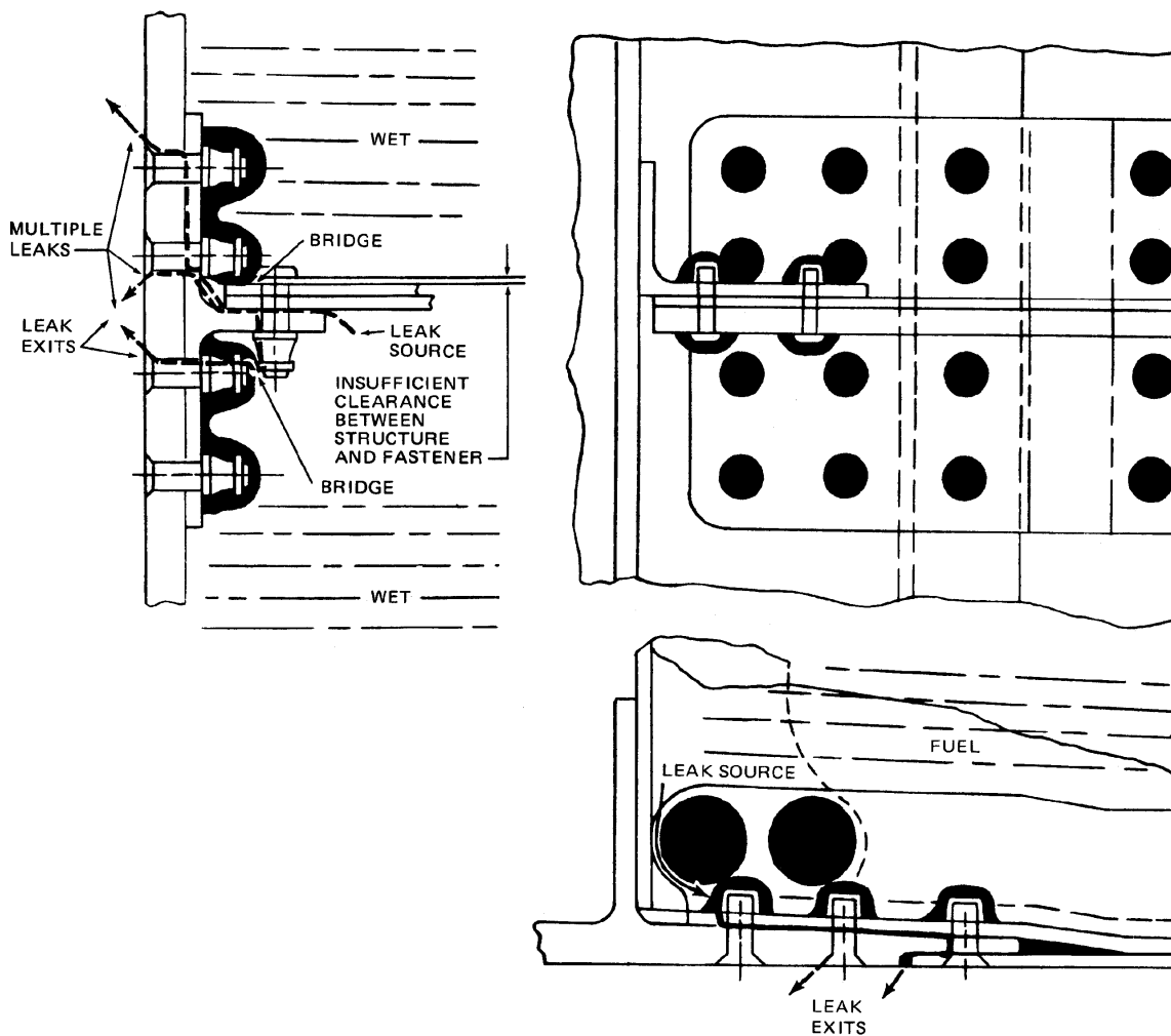
Figure 6-18. Multiple Leak Paths from a Single Leak Source
