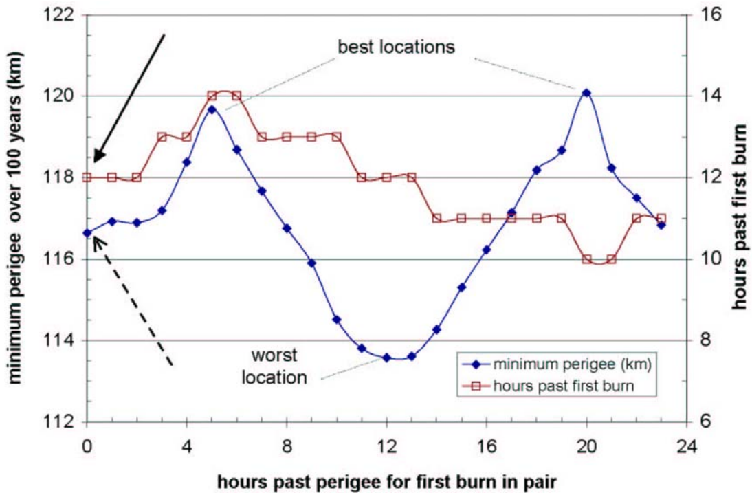
Figure C.4. Optimal locations in orbit for burn pair.
