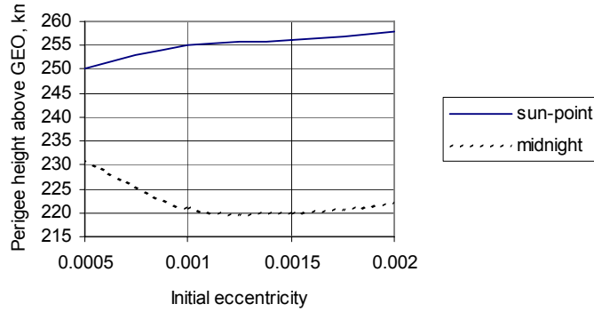
Figure B.7. Minimum perigee height above GEO vs. initial eccentricity.
