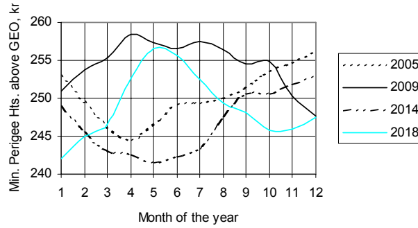
Figure B.5. Minimum perigee height vs. month of the year.
