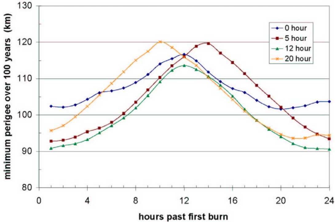
Figure C.5. Individual sample cases from Figure 10.4.
