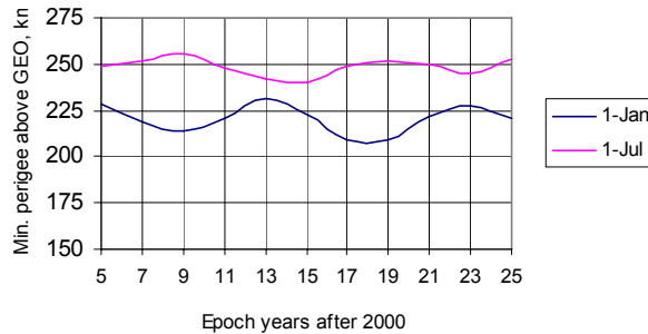
Figure B.4. Minimum perigee height vs. epoch.
