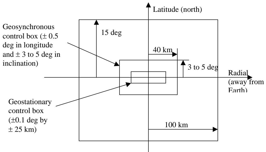
Figure 4.2. Cross section of the geosynchronous ring (not to scale).
