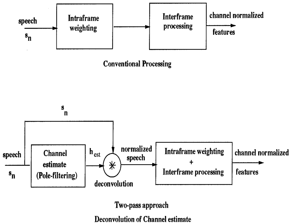
Figure 4.26: Combining inter-frame and intra-frame processing.
