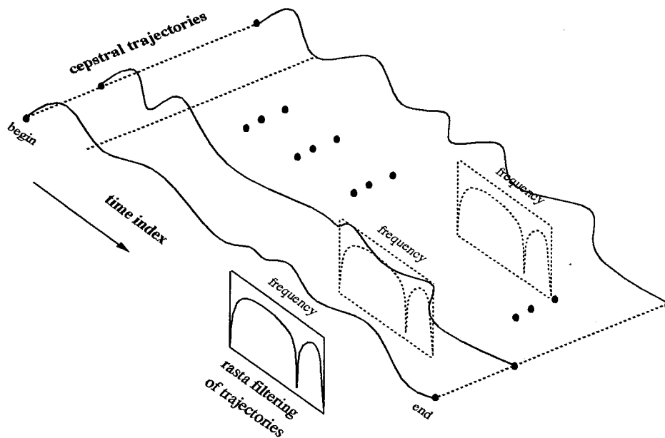
Figure 3.7: RASTA processing of cepstral trajectories.
