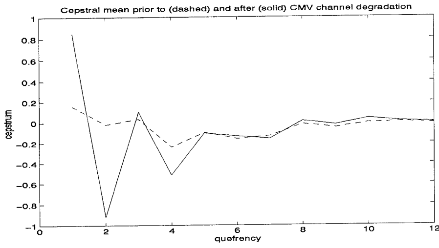
Figure 9.1: Comparison of cepstral mean of a speech utterance prior to and after channel degradation.
