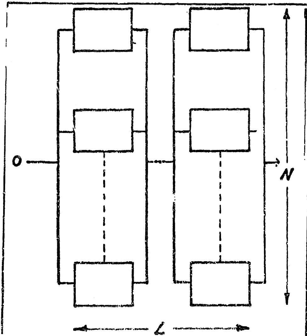
Figure 2.1. Full on Redundancy (Single Unit Necessary For Survival)
