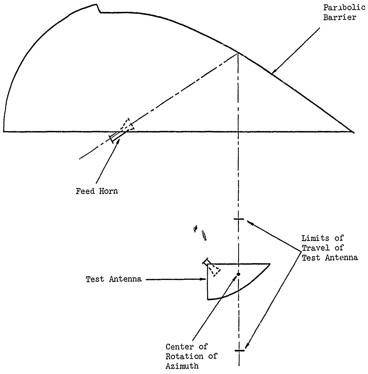
Figure 13. Plan View of the Two-Dimensional Compact Antenna Range.
