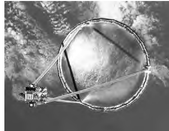
Figure 22-2. Spartan 207 inflatable antenna. (NASA photo)
