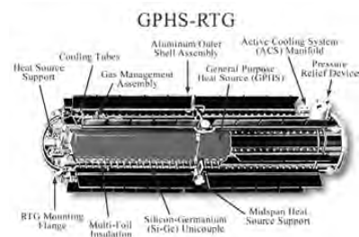
Figure 22-8. Radioisotope thermoelectric generator. (NASA graphic)
