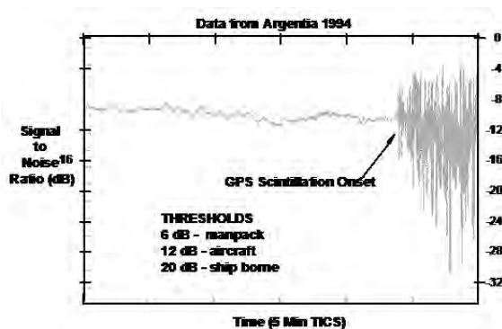
Figure 7-7. Scintillation effect on GPS signal. (Reprinted from Air University, Space Primer , unpublished book, 2003, 6-9.)
