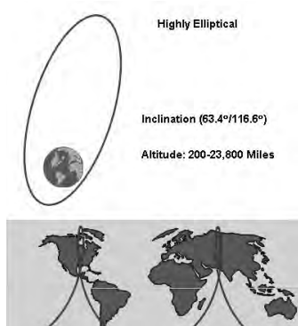
Figure 6-6. Molniya orbit. (Adapted from Air University, Space Primer , unpublished book, 2003, 8-18.)
