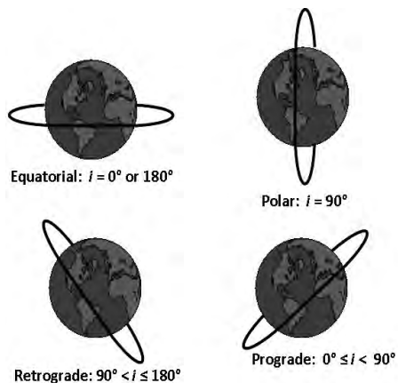
Figure 6-17. Orbital inclination types. (Created by ACSC)
