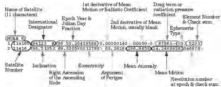
Figure 6-21. TLE set format. (Reprinted from NASA, "Definition of Two-Line Element Set Coordinate System," Human Space Flight Web site, http://spaceflight.nasa.gov/realdata/sightings/SSApplications/Post/JavaSSOP/SSOP_Help/tle_def.html [accessed 18 April 2008]).
