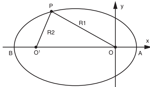
Figure 6-7. Kepler's first law. (Created by ACSC)
