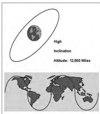
Figure 6-3. Semisynchronous orbit. (Adapted from Air University, Space Primer , unpublished book, 2003, 8-18.)
