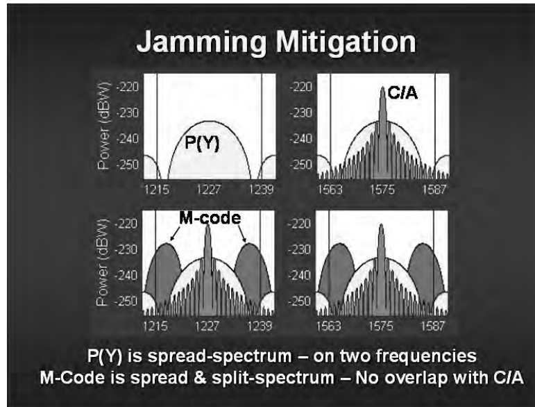
Figure 16-7. GPS signal structure. (NSSI graphic prepared by the author)
