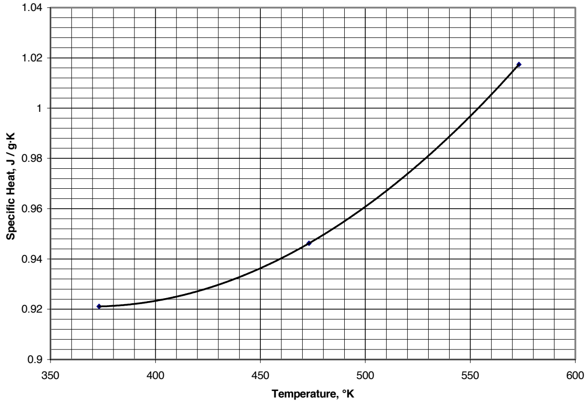
Figure 3.2.2.0(a). Effect of temperature on specific heat of 2224A-T351.
