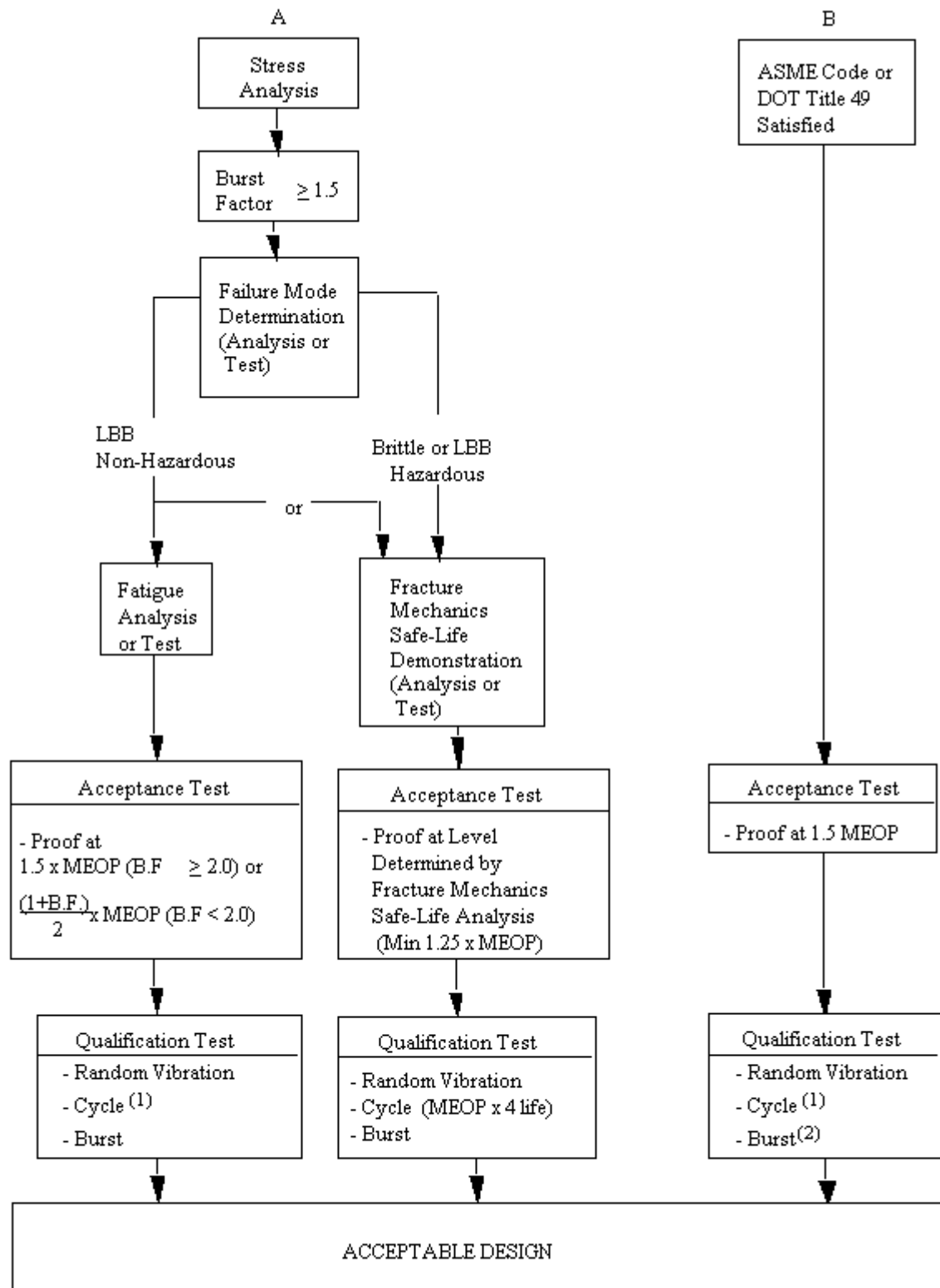
Figure 12.1. Pressure Vessel Design Verification Approach.
