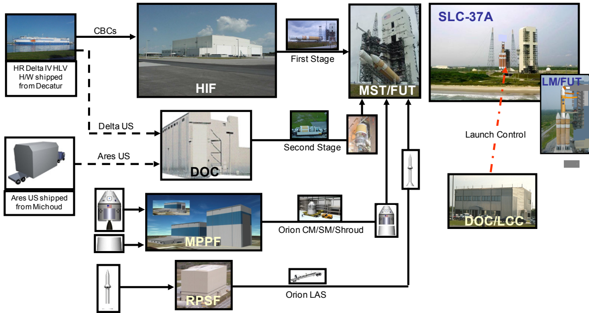
Figure 8. Option A: HR Delta IV H/Orion launch from a new SLC-37A complex.
