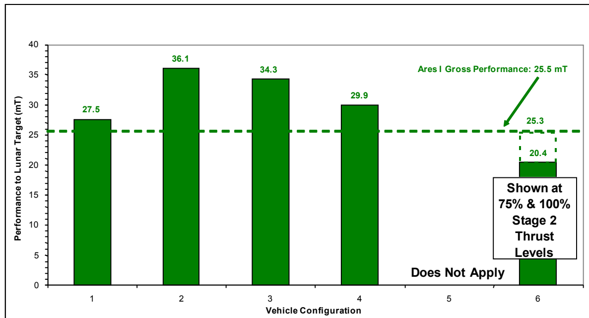
Figure 5. HR Delta IV H lift performance to lunar requirement.
