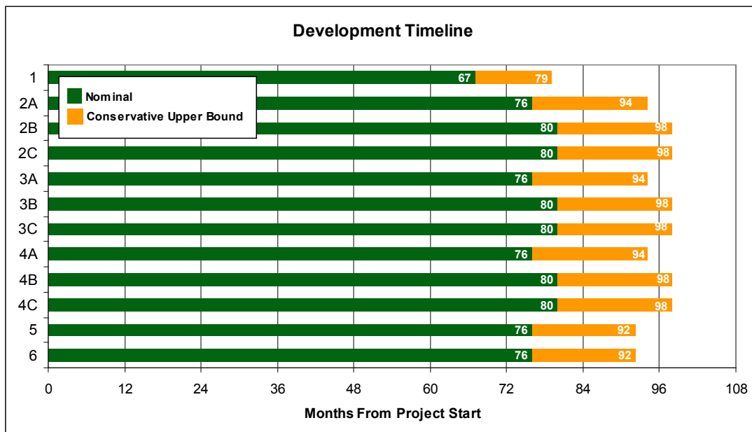
Figure 14. HR Delta IV H development time estimates.
