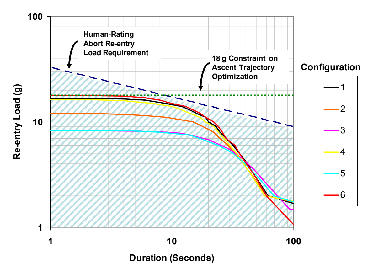
Figure 3. Abort re-entry g-load requirement compared to HR Delta IV H maximum re-entry loading.
