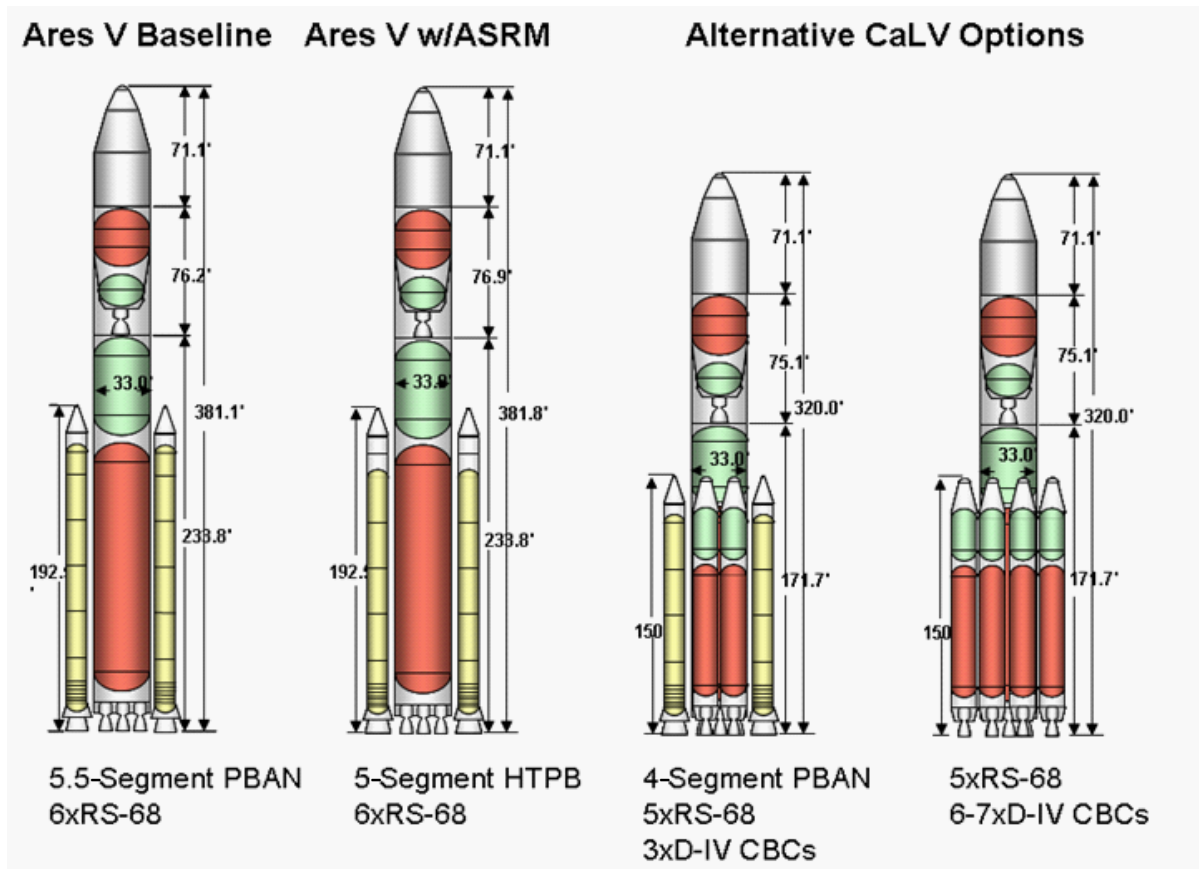
Figure 10. Ares V options and alternative CaLV options.
