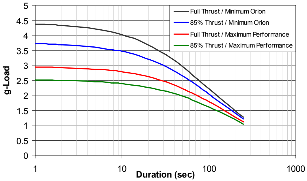
Figure 6. Orion ascent g-loading for configuration 3.
