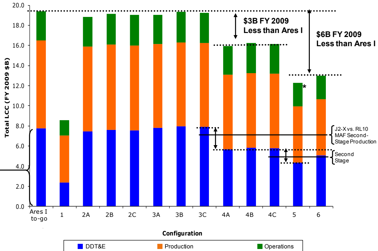
Figure 13. Lifecycle costs for HR Delta IV H compared to Ares I (at 21 percent confidence level without carrying costs).
