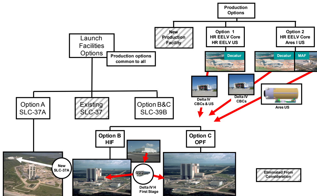
Figure 7. Ground infrastructure options examined.
