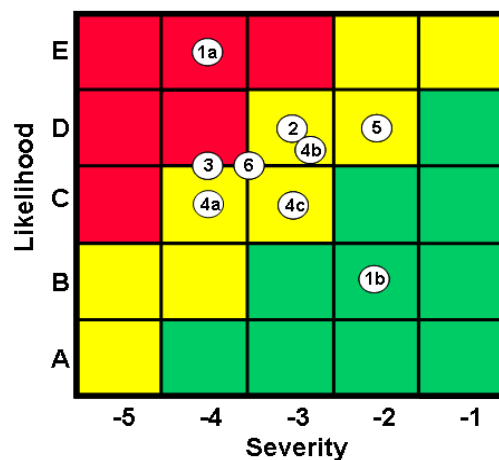
Figure 12. Preliminary HR Delta IV H NSS risk assessment matrix.
