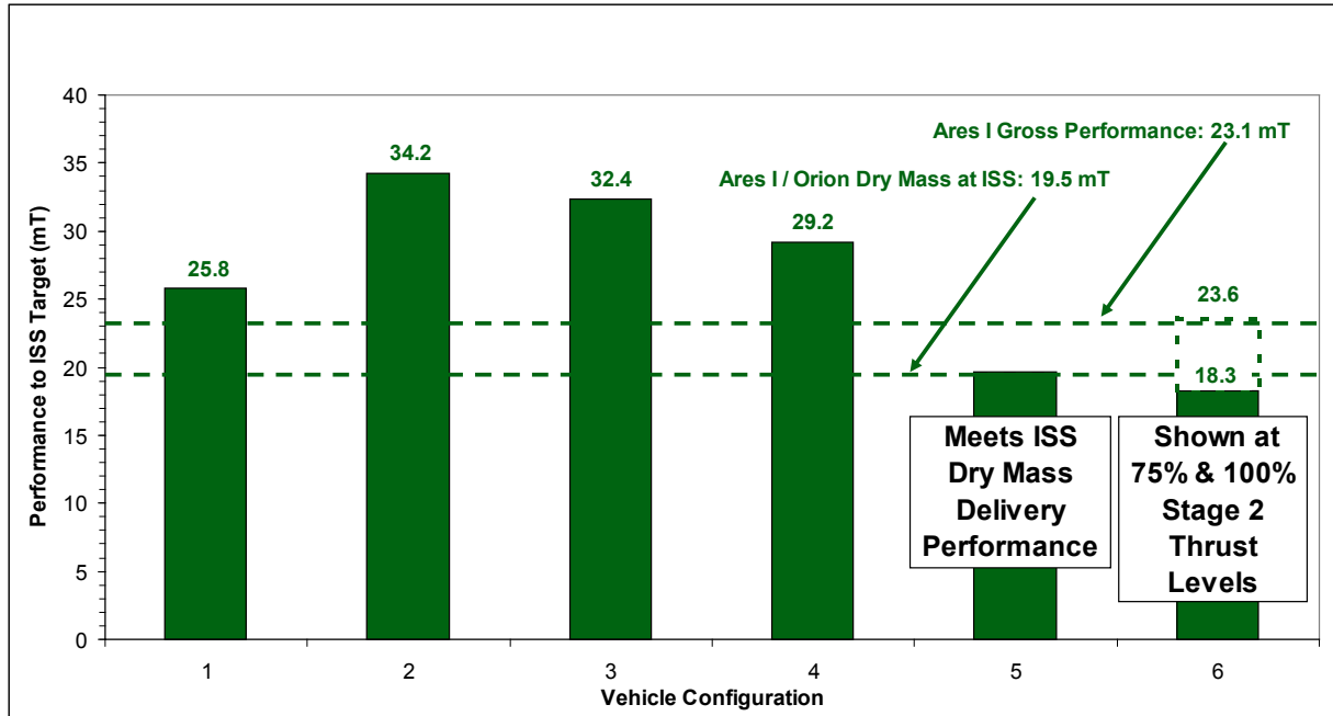
Figure 4. HR Delta IV H lift performance to ISS requirement.
