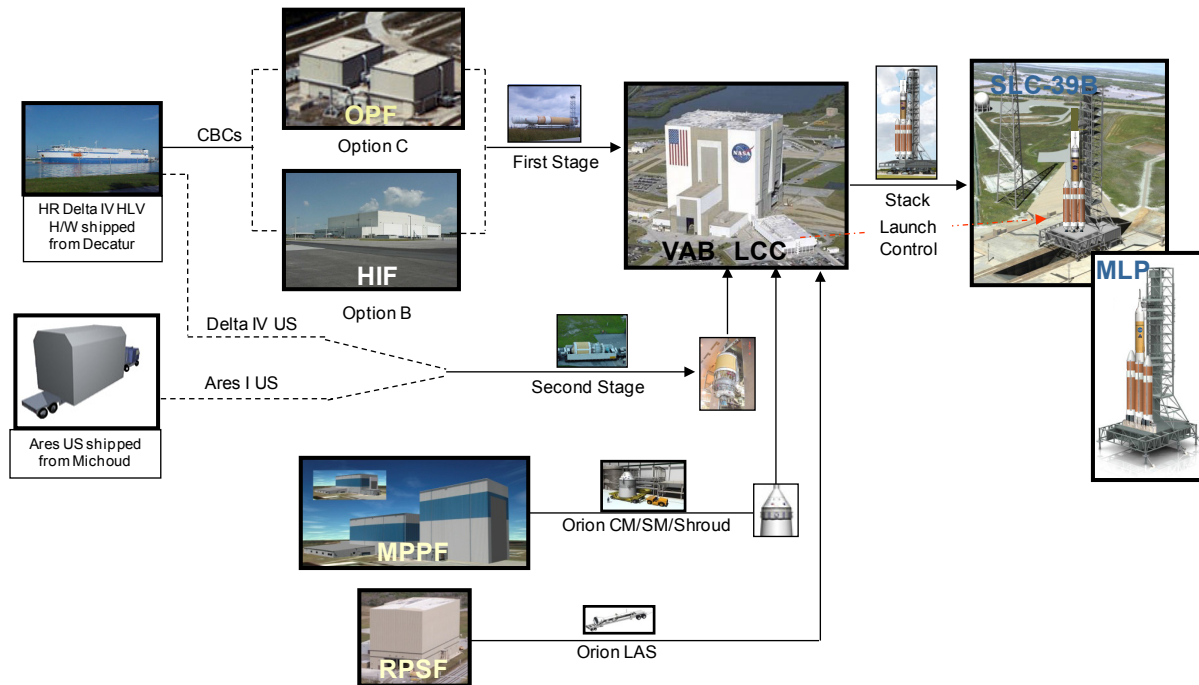
Figure 9. Options B and C for HR Delta IV H launch processing infrastructure.
