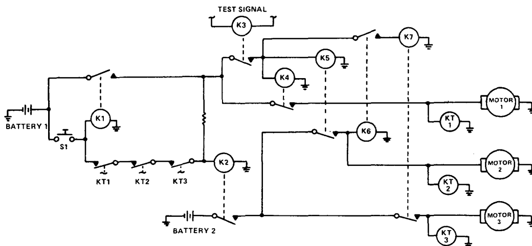
Figure IX-1. Power Distribution Box Fault Tree Example
