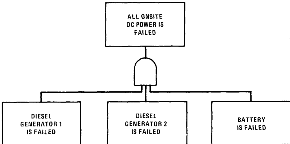
Figure IV-6. Specific Example of an AND-Gate
