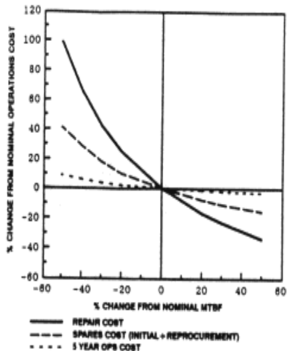
Figure B-11 — Effect of MTBF on Operations Cost.
