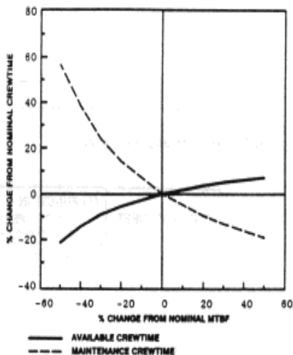
Figure B-12 — Effect of MTBF on Crew Time.
