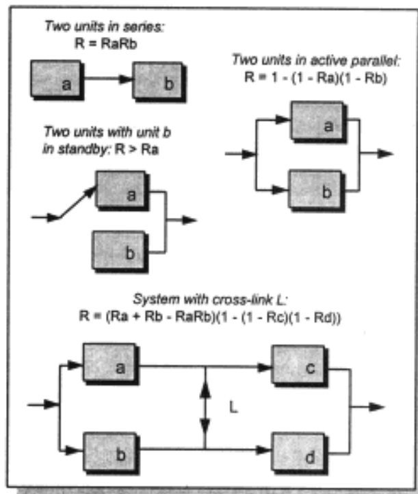
Figure 29 — Basic Reliability Block Diagrams.
