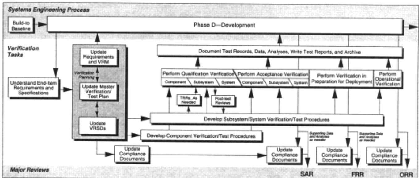
Figure 32b — Verification Process Flow (Phase D).
