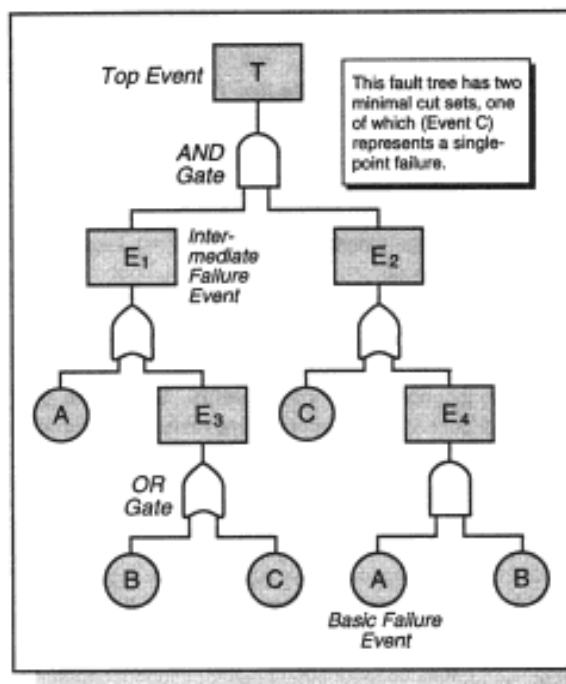
Figure 30 — A Simple Fault Tree.
