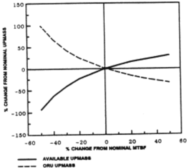
Figure B-13 — Effect of MTBF on Upmass.
