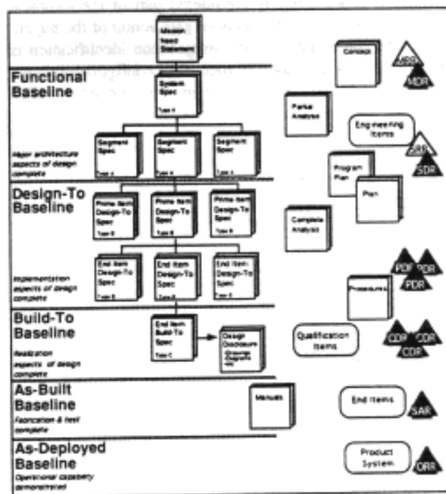
Figure 17 — Evolution of the Technical Baseline.
