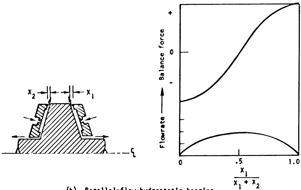
(b) Parallel-flow hydrostatic bearing
