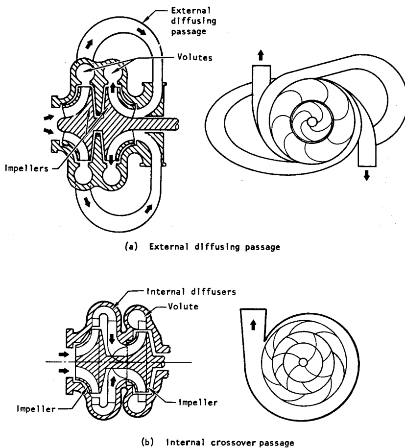
Figure 11. — Basic types of interstage flow passages.
