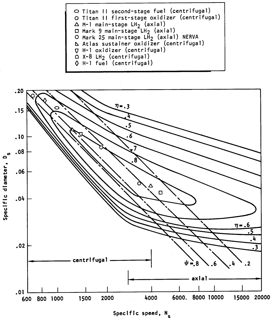
Figure 3. — Representative N_s - D_s diagram for centrifugal and axial flow turbopumps.
