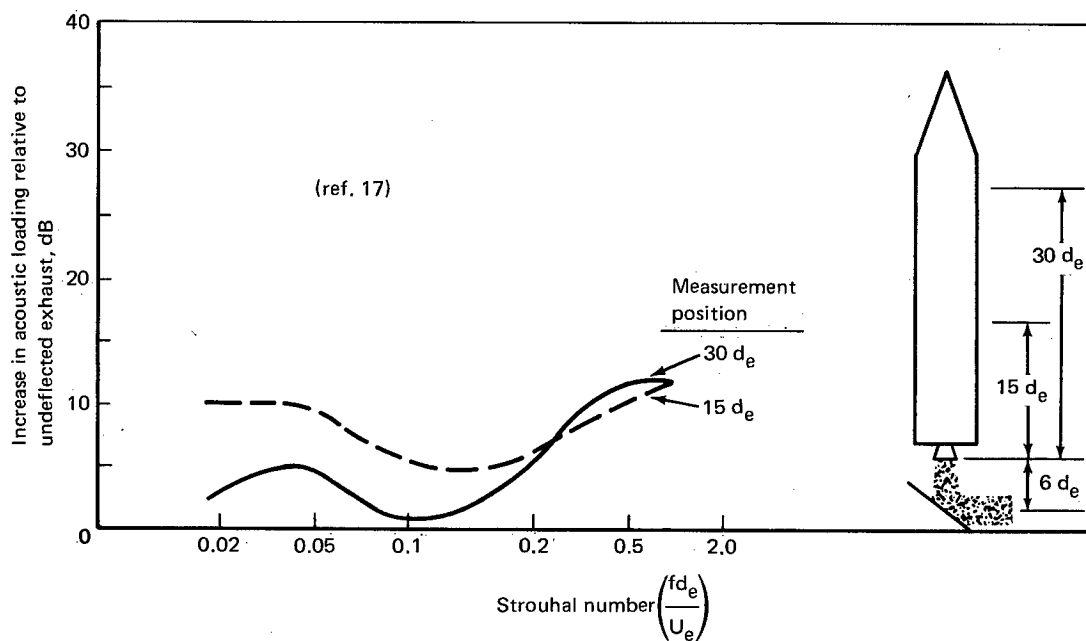
Figure 15. — Examples of the increase in noise level as a result of deflecting the exhaust flow.
