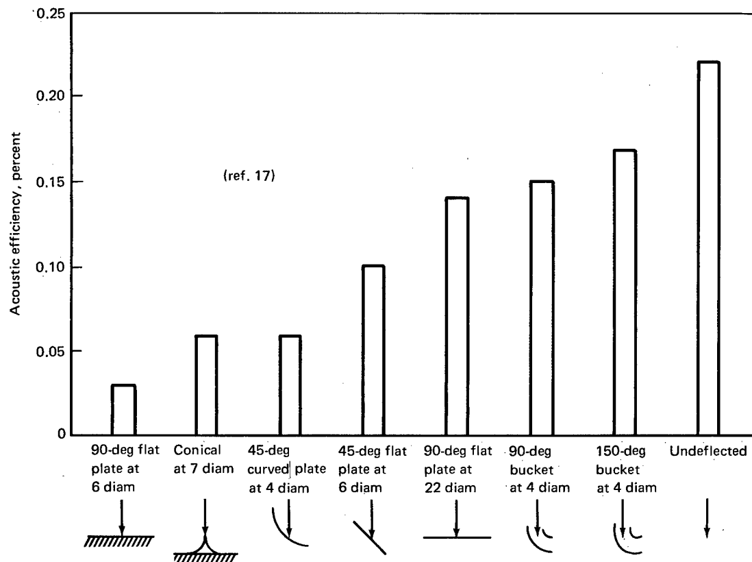
Figure 4. — Acoustic efficiency of various deflected rockets.
