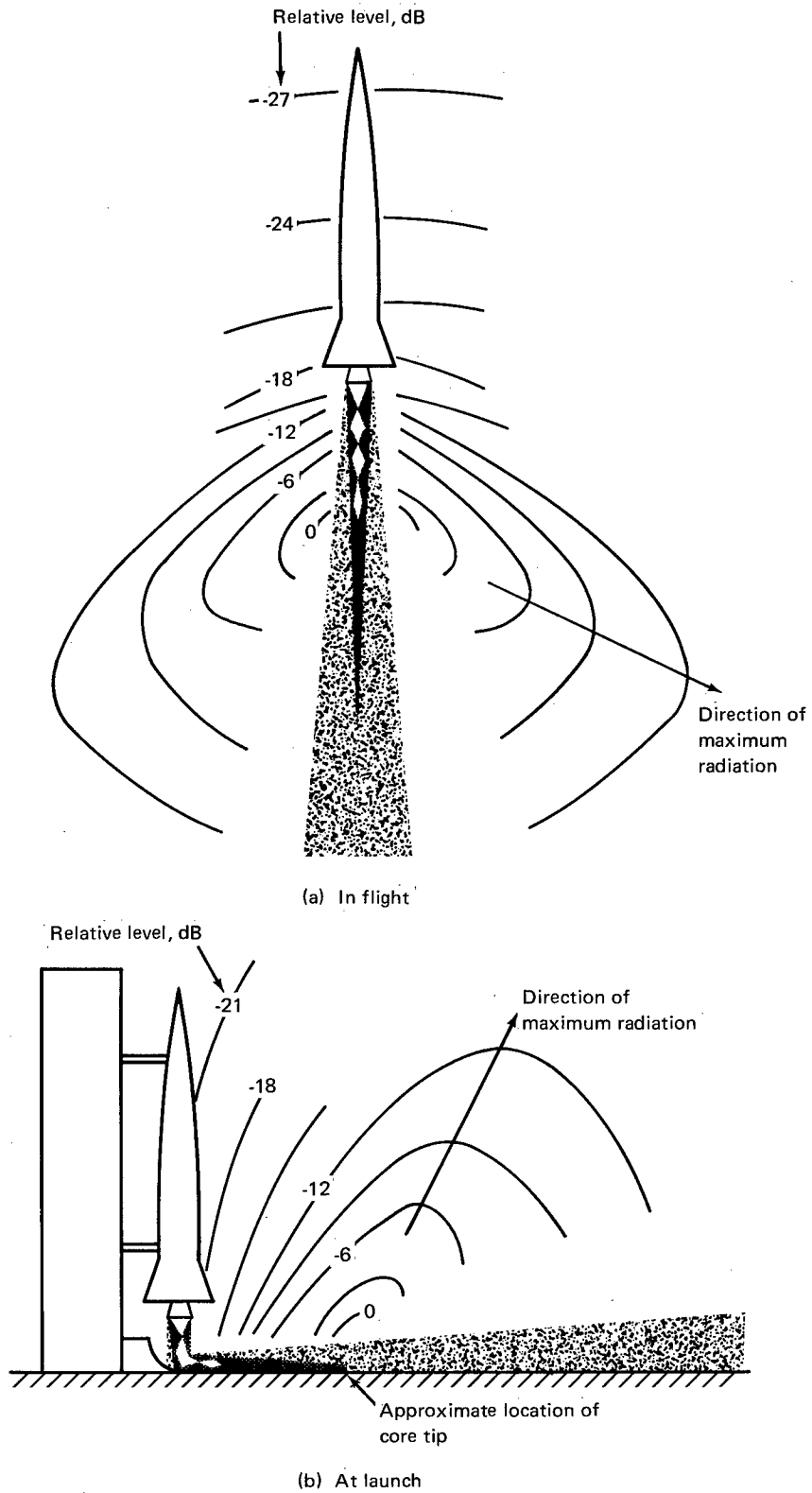
Figure 1. — Sketch of the rocket flow and contour of equal overall sound-pressure level for flight and launch cases.
