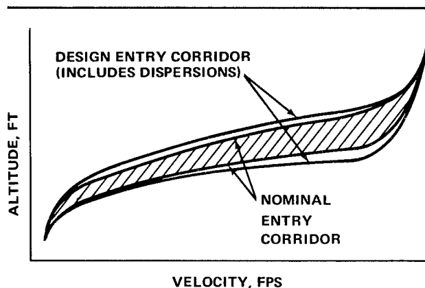
FIGURE 5-2 DESIGN ENTRY CORRIDOR
