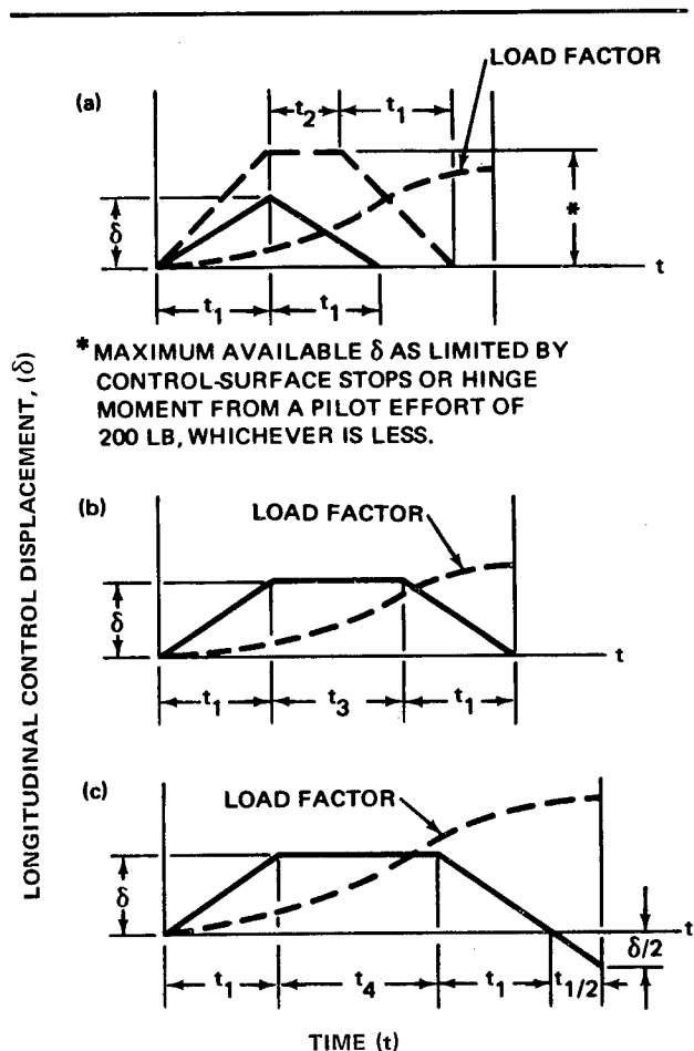
FIGURE 5-5 LONGITUDINAL CONTROL DISPLACEMENT-TIME DIAGRAM
