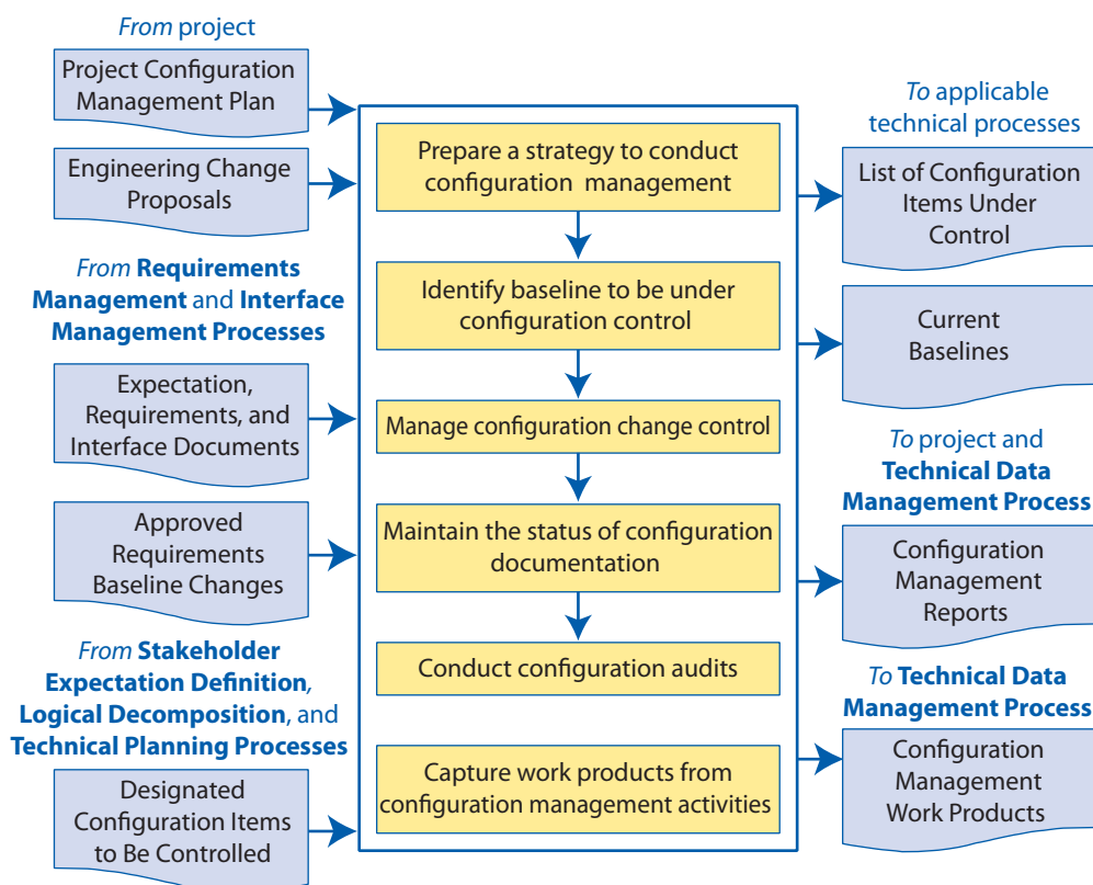
Figure 6.5-1 CM Process
