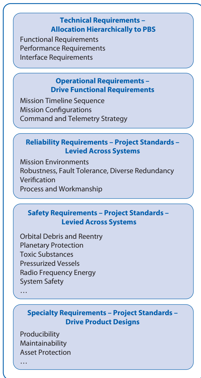
Figure 4.2-2 Characteristics of functional, operational, reliability, safety, and specialty requirements
