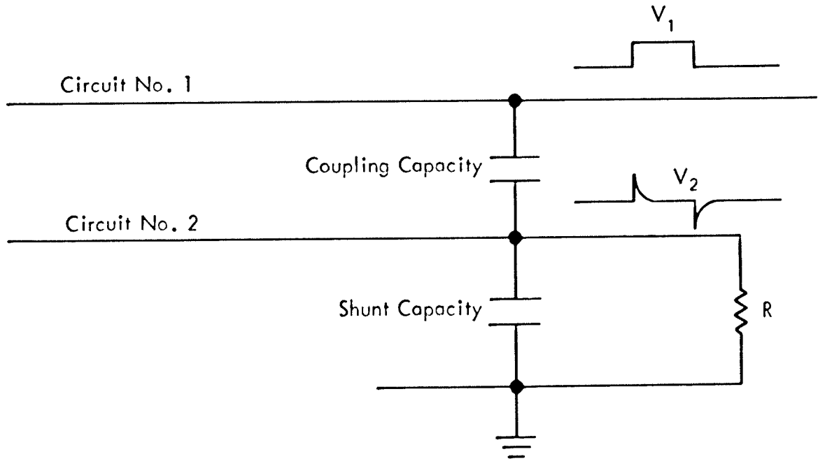
Figure 4. - Capacitive coupling.
