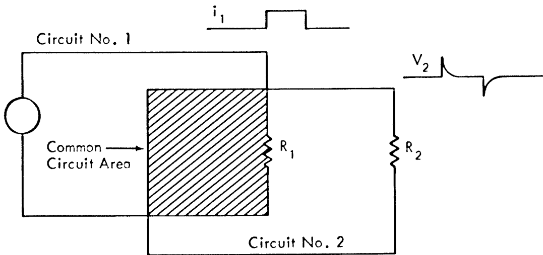
Figure 5. - Inductive coupling.
