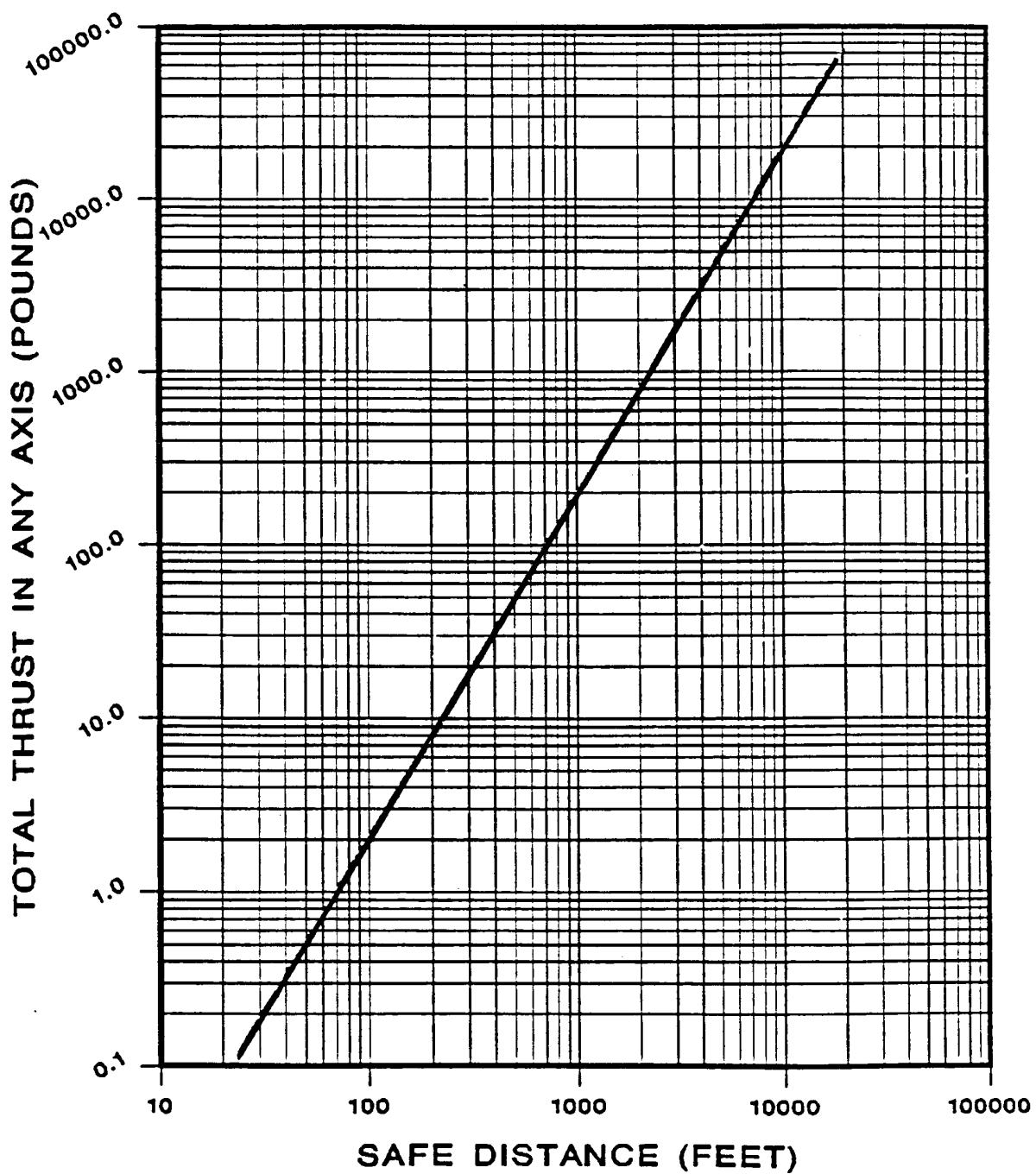
Figure 1.- Safe distance for firing liquid propulsion thrusters.
