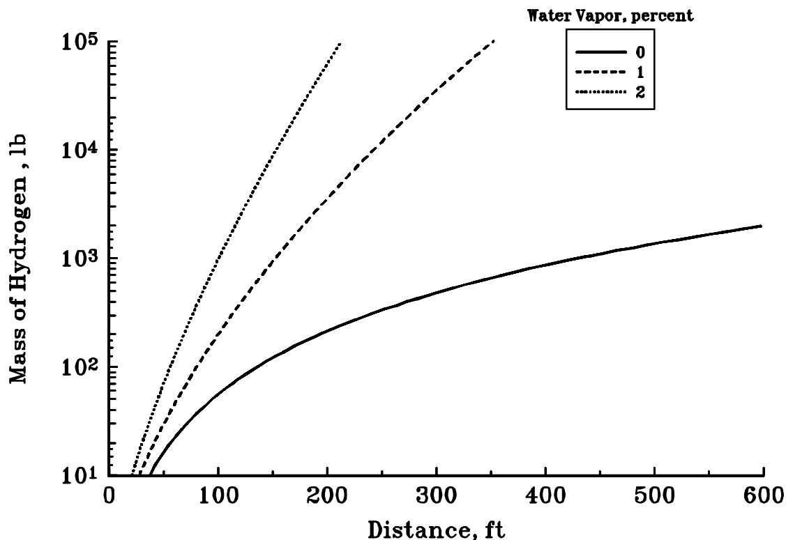
Figure A2.6 Variation in Distance from a Hydrogen Fire for a Thermal Radiation Exposure of 2 \text{ cal/cm}^2 for an Exposure Duration of 10 s
