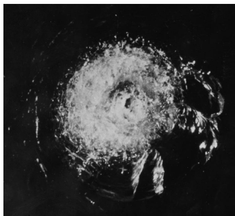
Figure 2. Shuttle window pit caused by impact with a paint chip.
