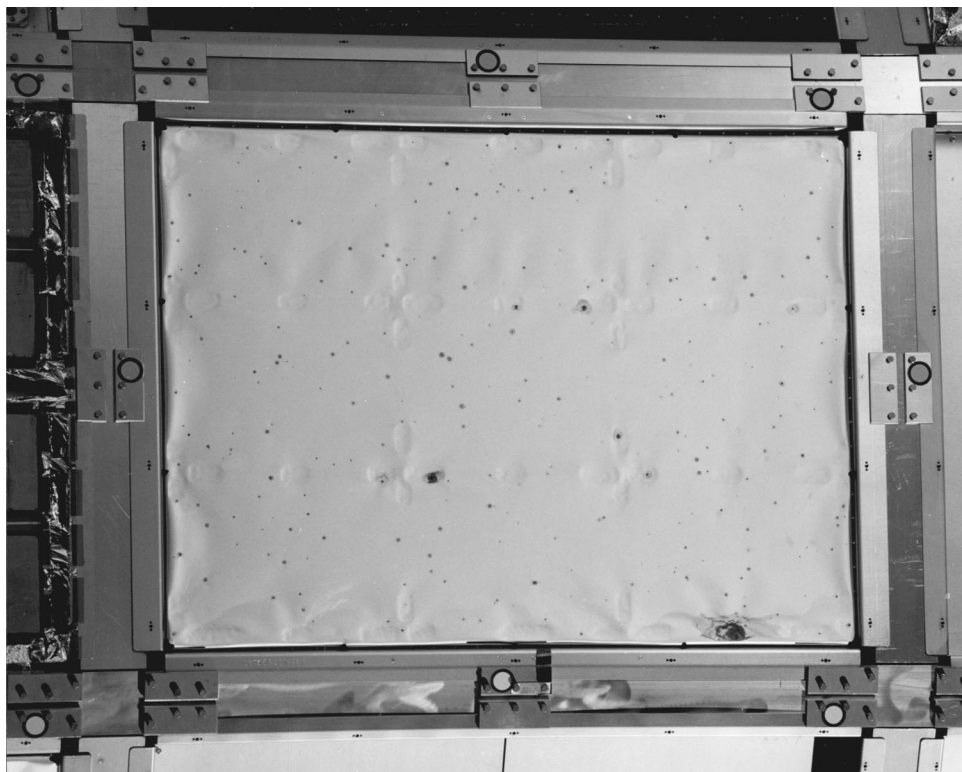
Figure 5. Orbital debris impact damage to silver Teflon™ blanket on LDEF.
