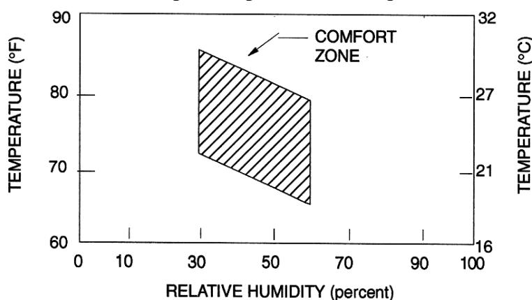
Figure 6-1: Comfort Zone Chart Temperature Requirements
