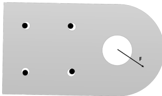
Figure 21b—Rigid Body Response for Lug with Clearance Holes
