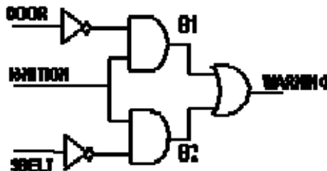
Figure B-4: Warning Buzzer Example
