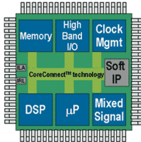
Figure C-12: Reconfigurable SoC
