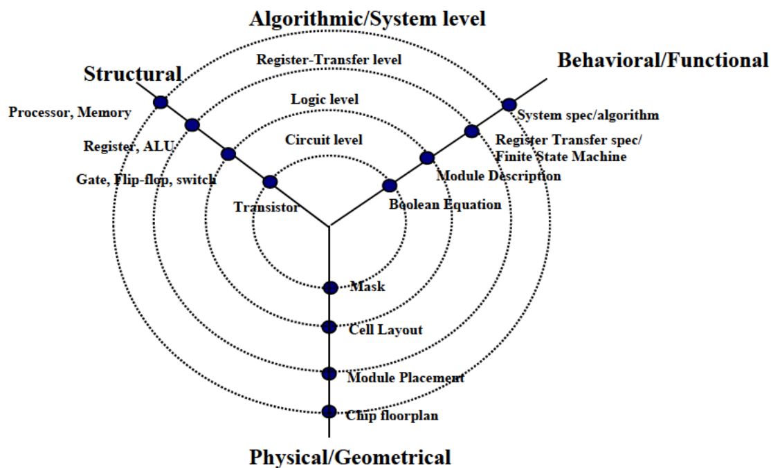
Figure 4: Complex Electronics Design Views
