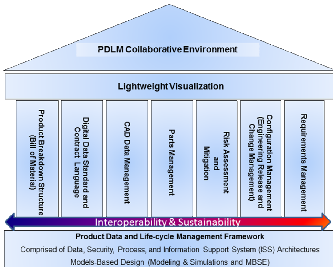
Figure 2—PDLM Framework
