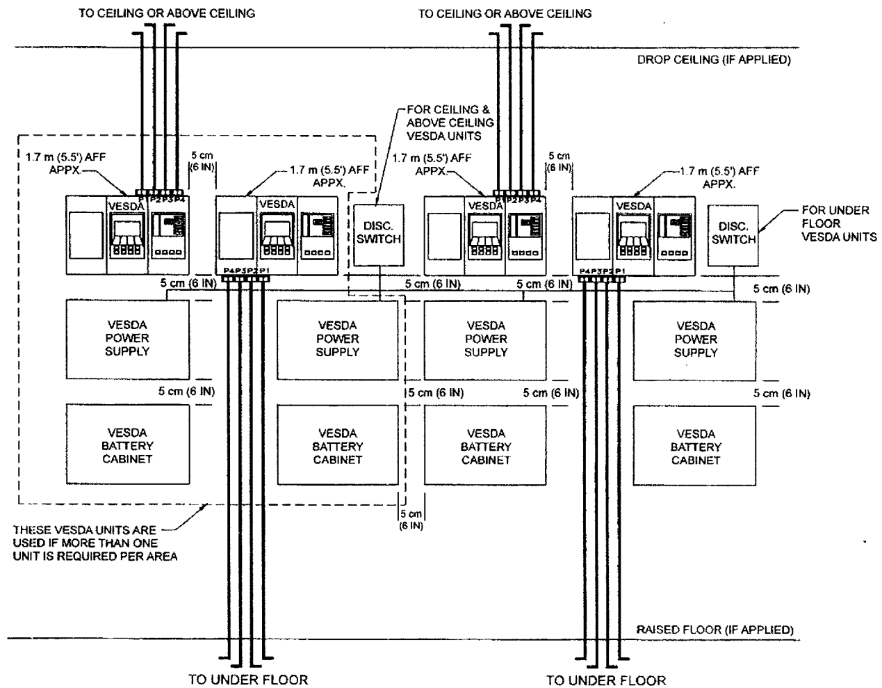
TYPICAL MOUNTING OF VESDA CABINETS
