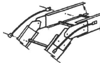
D. Cable Tray Sections Vertical Adjustable Splice Plate
