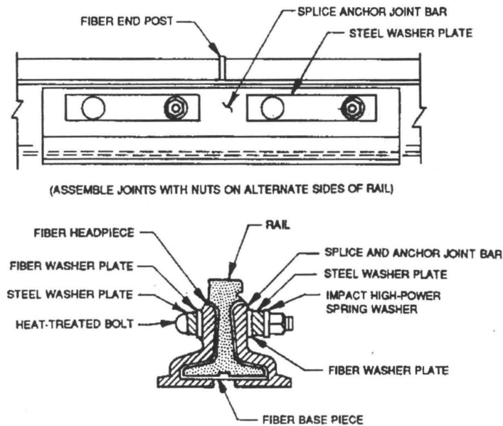
5(a) SIDE AND SECTION VIEWS OF A TYPICAL INSULATED JOINT
