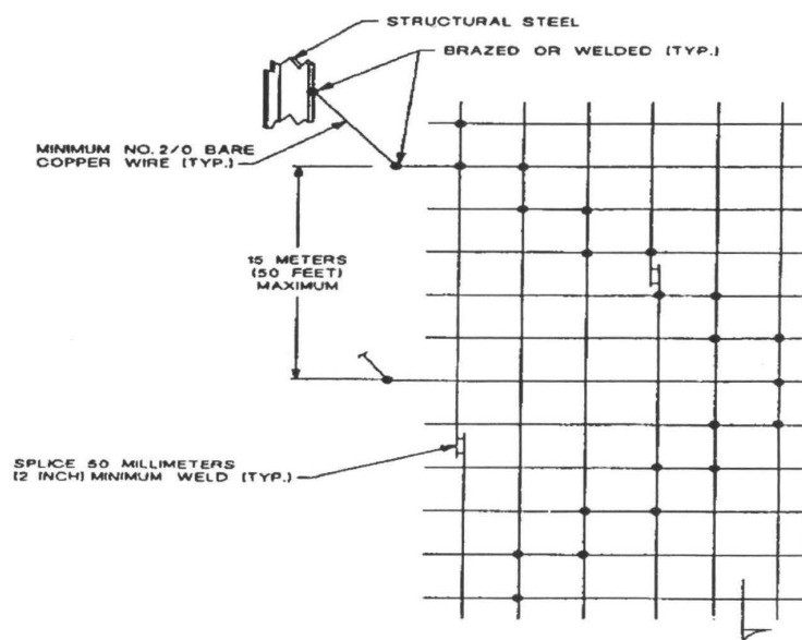
Figure 7. Bonding and Grounding of Reinforced Concrete
