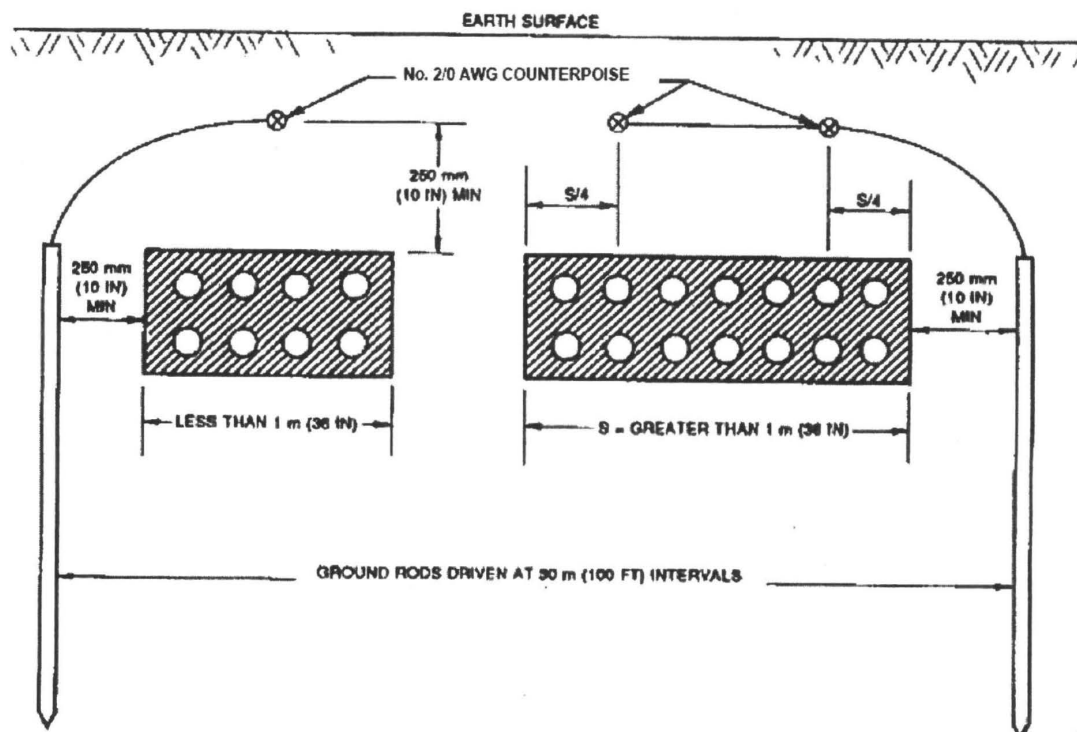
Figure 13. Lightning Protection for Underground Duct Banks
