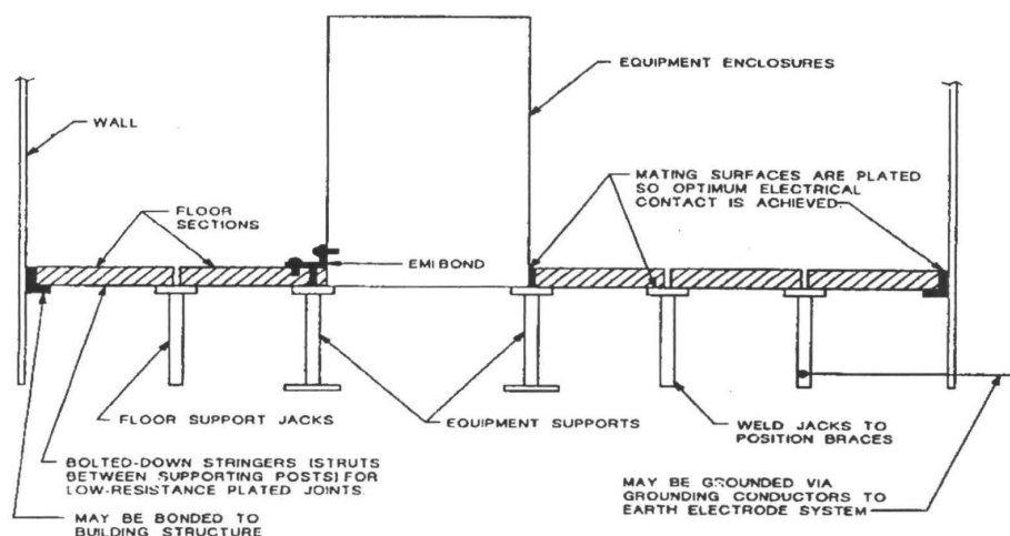
Figure 2. Grounded Raised Floor
