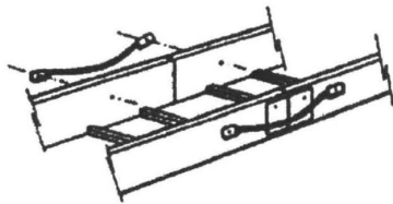
A. Expansion Splice Plates
