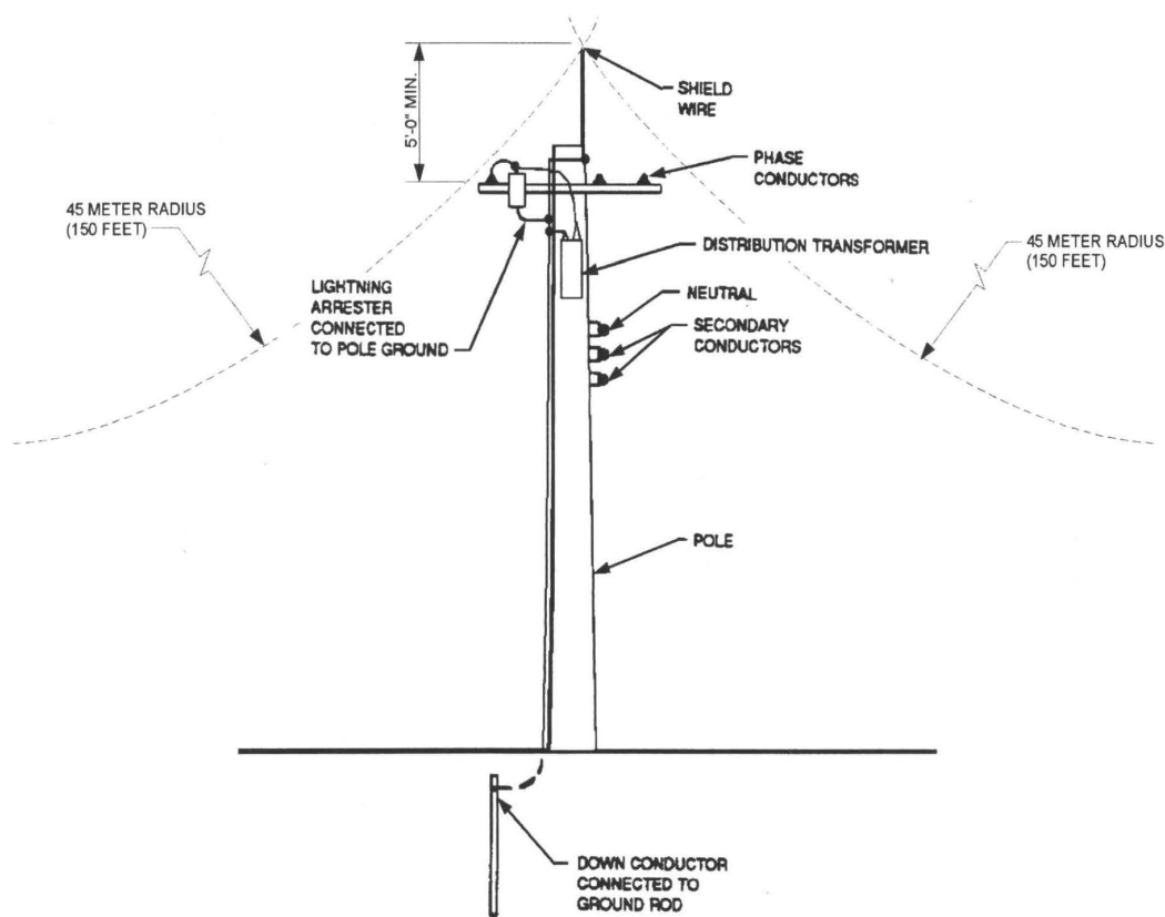
Figure 12. Shield Wire and Lightning Arrester Typical Installation
