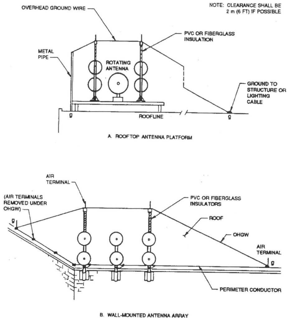
Figure 8. Rooftop Antenna Lightning Protection
