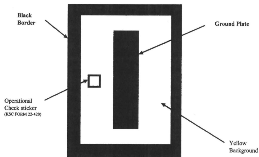
Figure 4. Ground Plate Marking
