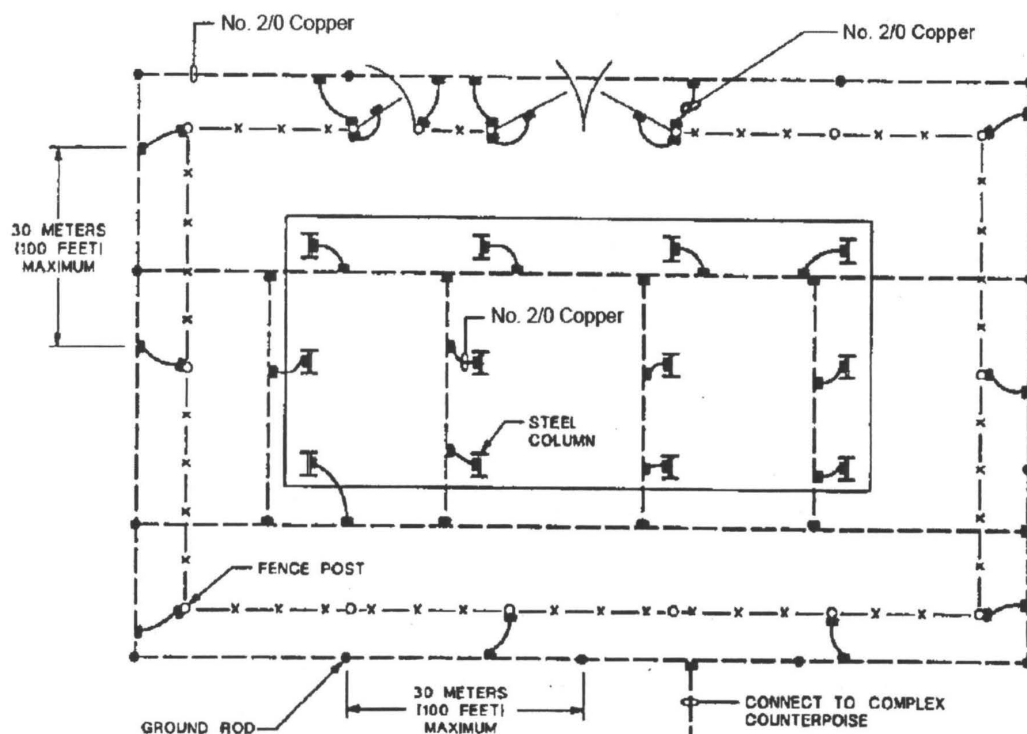
Figure 5. Connection of Substation Fence and Structural Steel
