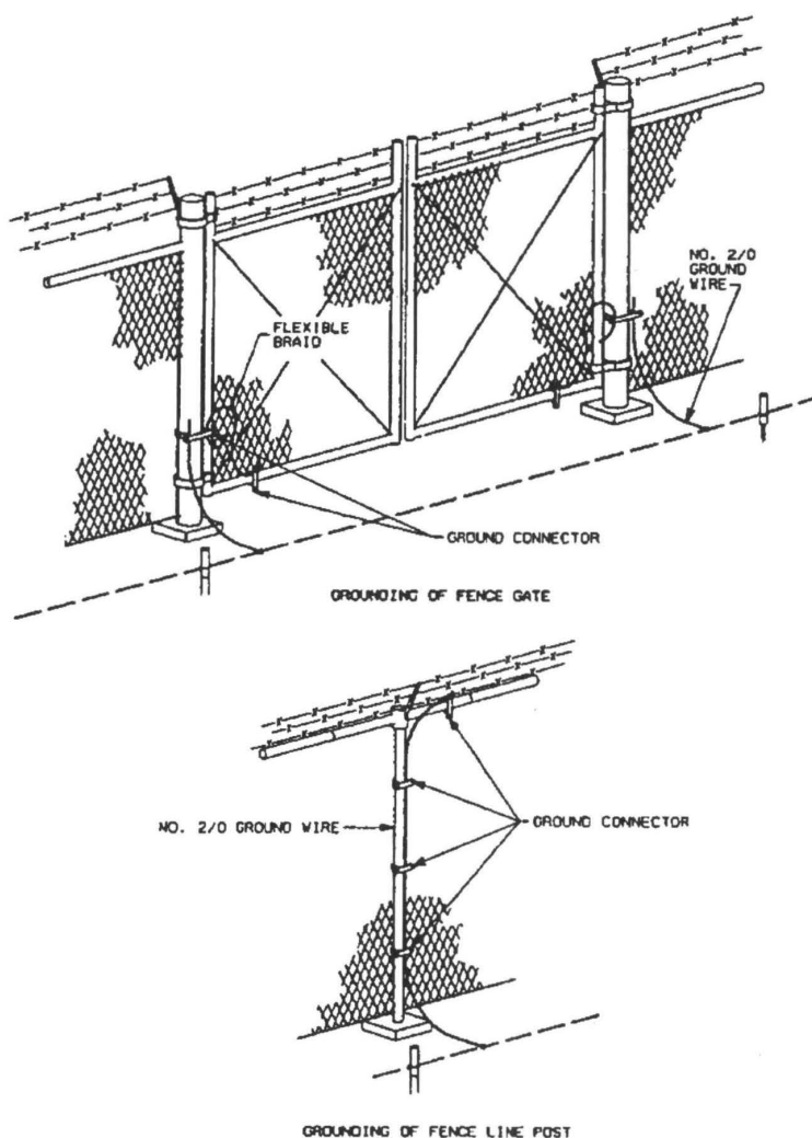
Figure 6. Substation Fence Detail
