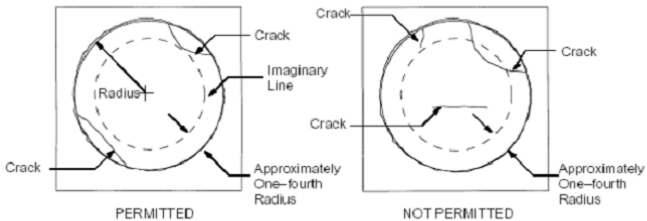
Figure 19. Cracks on the Endface of an Optical Fiber
