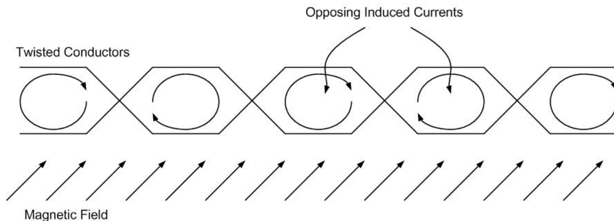
Figure 4. Twisted Conductor
