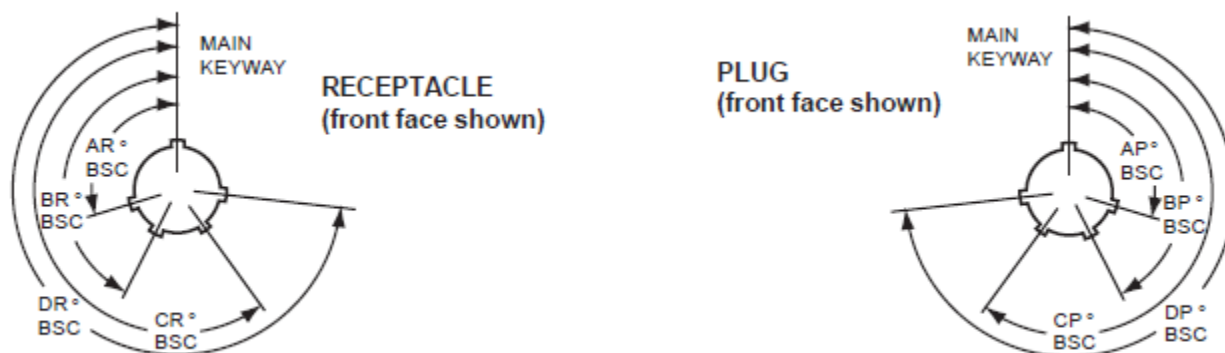
Figure 9. 38999 Polarization Angles
