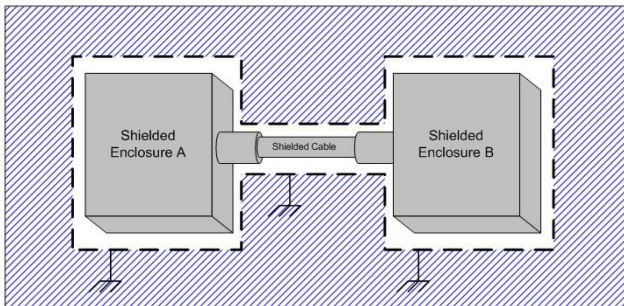
Figure 3. Shielded “Barbell”
