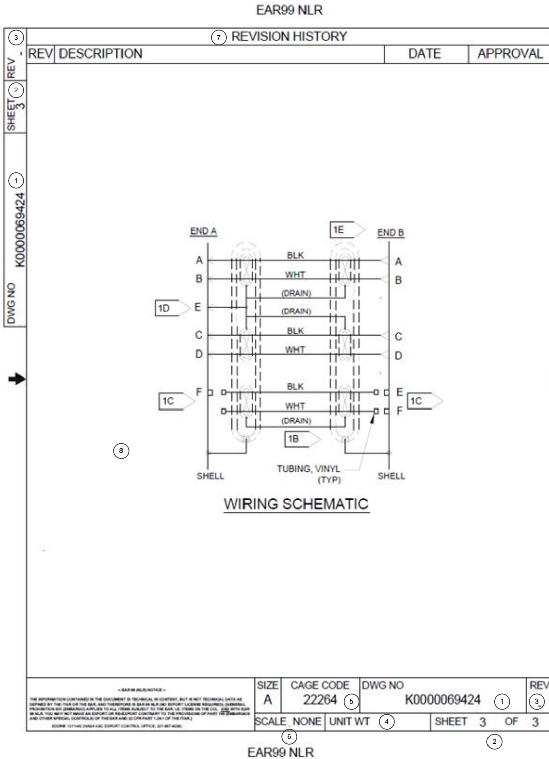
Figure 14. Cable Subassembly Drawing – Continuous/Last Page
