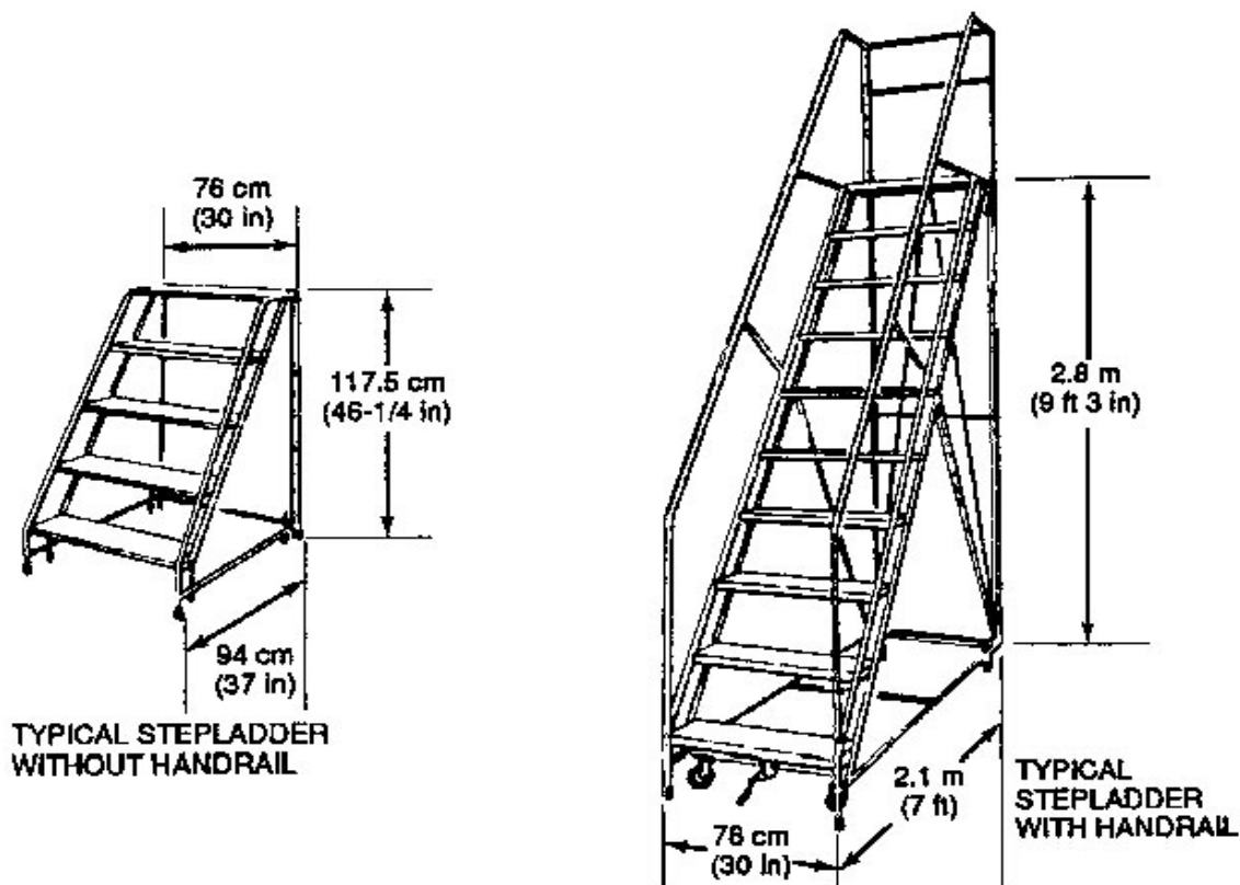
Figure 3-25. Typical Access Stepladders With and Without Handrails
