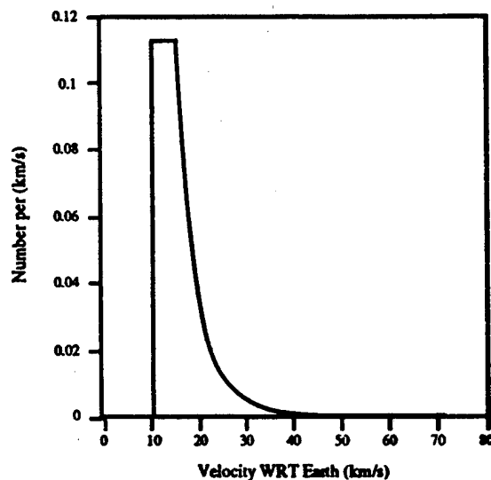
Figure 7-1. Normalized meteoroid velocity distribution from equation (7-3).
