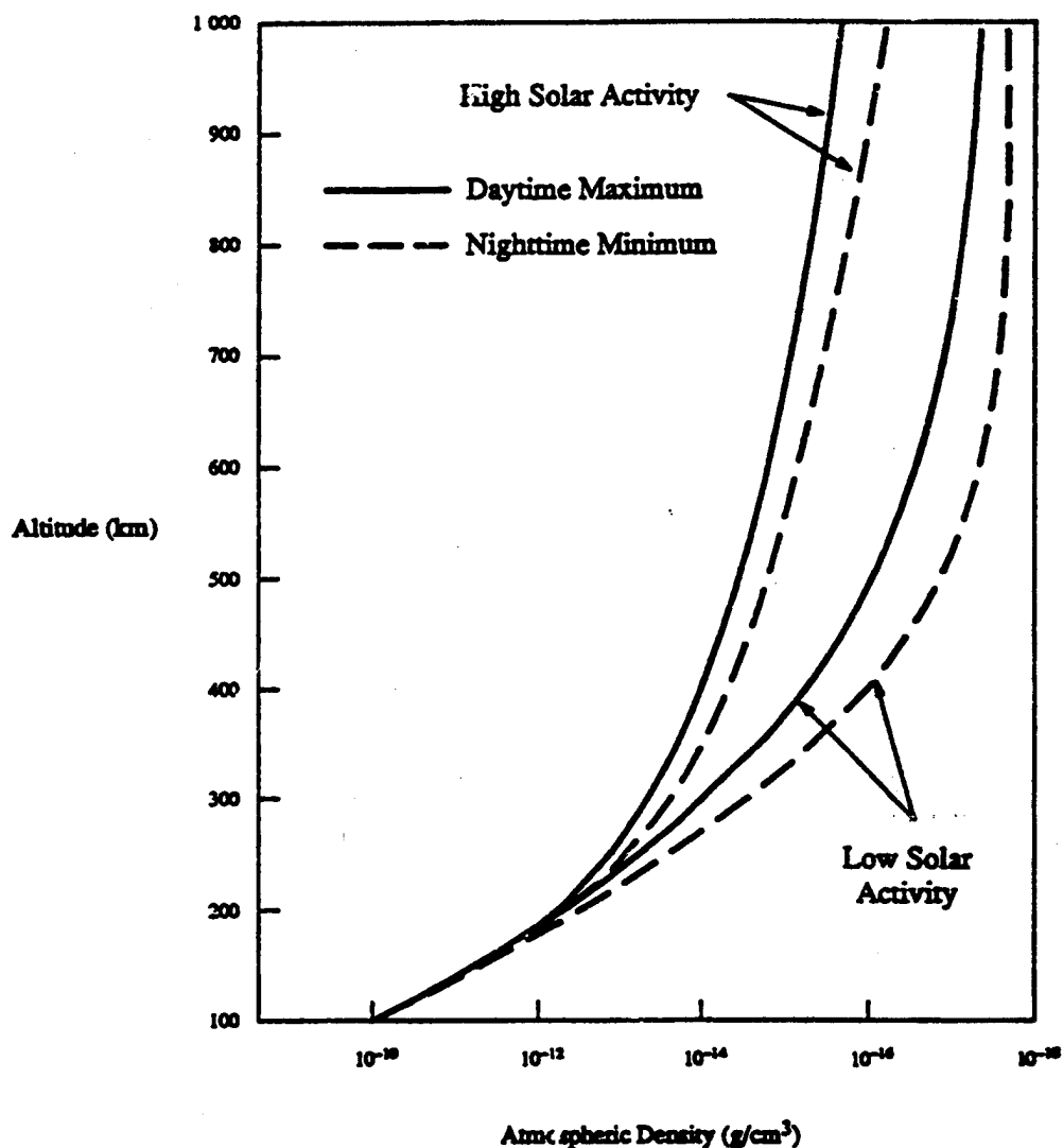
Figure 3-2. Typical atmospheric mass density profiles at high and low solar activity. (For information only; not for design use.)
