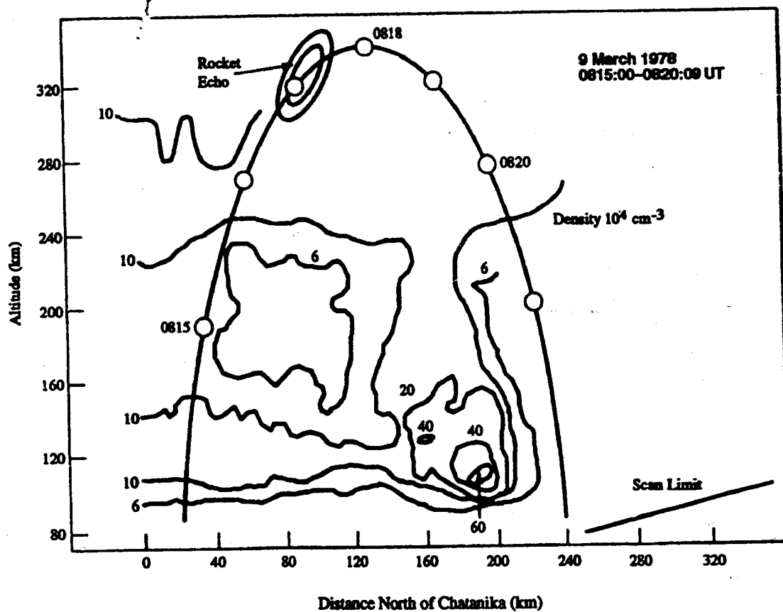
Figure 4-5. Ionospheric electron density in an aurora ( \times 10^4 n_e/cm^3 ). 14
