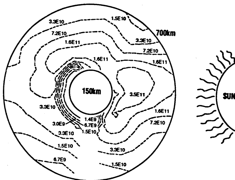
Figure 4-3. Noon-midnight cross section view of plasma density ( m^{-3} ) as a function of altitude from 150 to 700 km for June 21 and solar minimum conditions ( F_{10.7} = 70 , contours in the 0^\circ and 180^\circ longitude plane, IRI90 results with default options selected).
