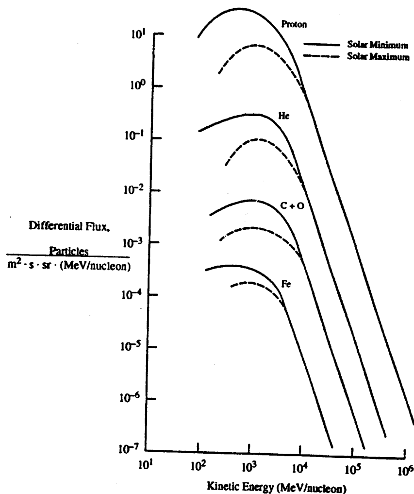
Figure 5-6. Characteristics of GCRs. Differential energy spectra for GCRs outside the magnetosphere at maximum and minimum solar activity (as defined by sunspot number).
