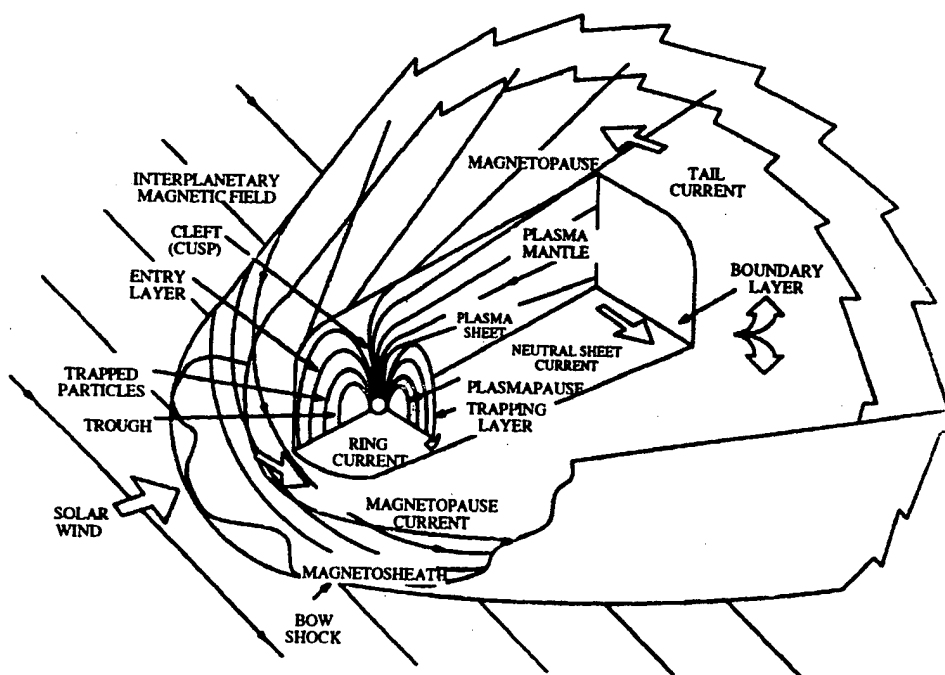
Figure 2-1. Schematic view of terrestrial space. 4
