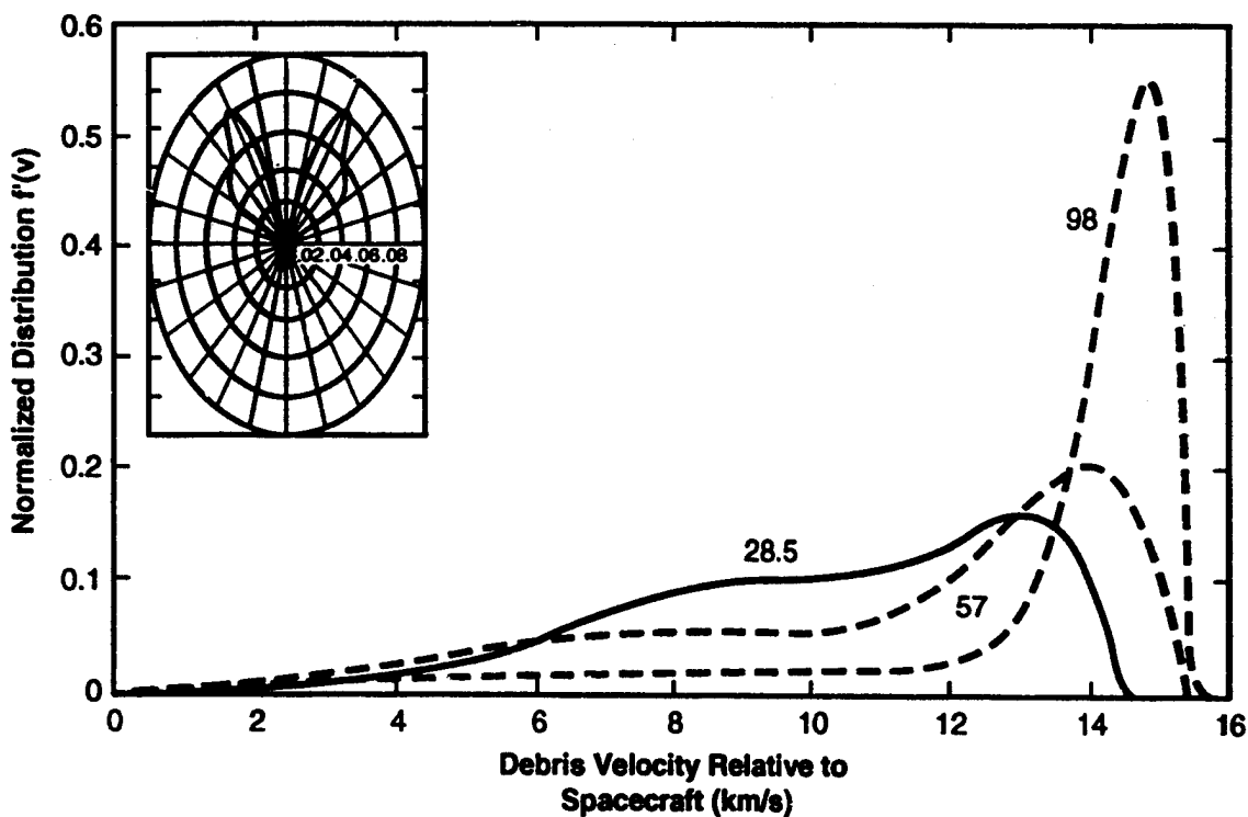
Figure 7-3. Normalized collision velocity distribution as function of the debris velocity for a spacecraft with orbital inclinations of 28.5°, 57°, and 98°.
