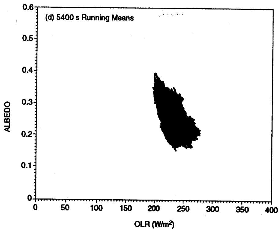
Figure 9-8. Albedo-OLR correlated pairs for 90° inclination orbits (page 2 of 2).
