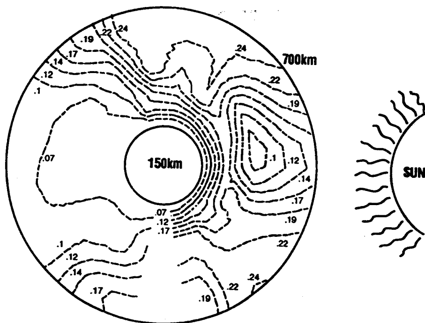
Figure 4-4. Noon-midnight cross section view of electron energy (eV) as a function of altitude from 150 to 700 km for June 21 and solar minimum conditions ( F_{10.7} = 70 , contours in the 0^\circ and 180^\circ longitude plane, IRI90 results with default options selected).
