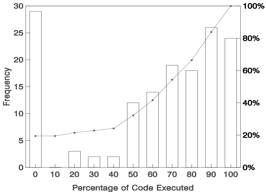
Figure 1 - Distribution of test case coverage.
