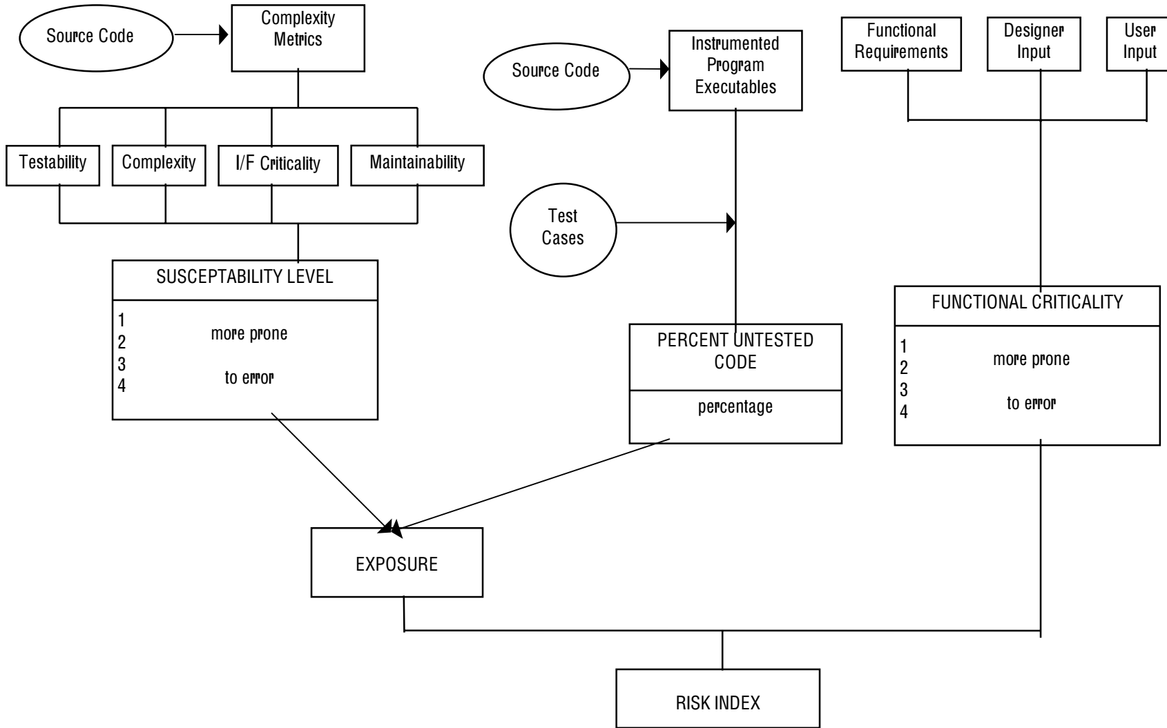
Figure 2 - Derivation of the risk index.
