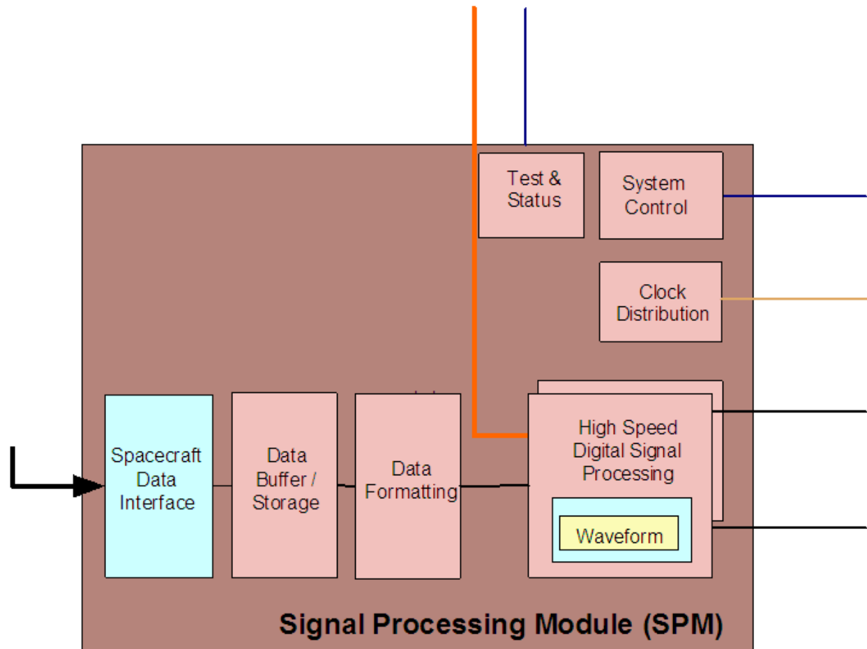
Figure 5-4 SPM Architecture Details
