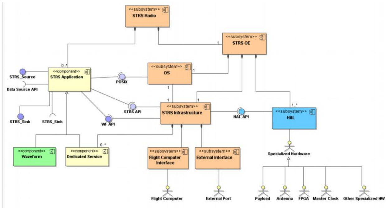
Figure 8-2 STRS Layered Structure in UML
