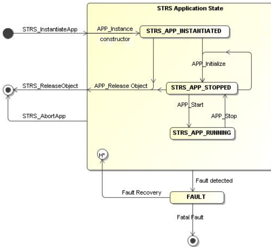
Figure 8-7 STRS Application State Diagram
