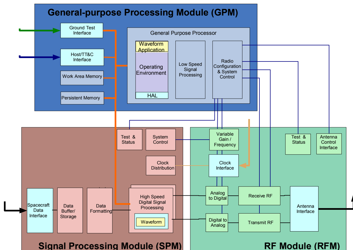
Figure 5-2 STRS Hardware Architecture Implementation
