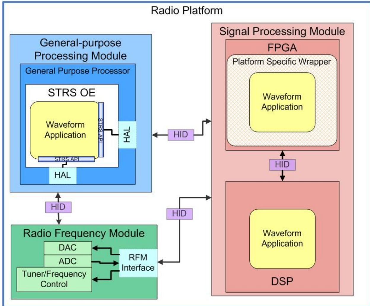
Figure 7-1 High-level Software & Firmware Waveform Applications Interfaces
