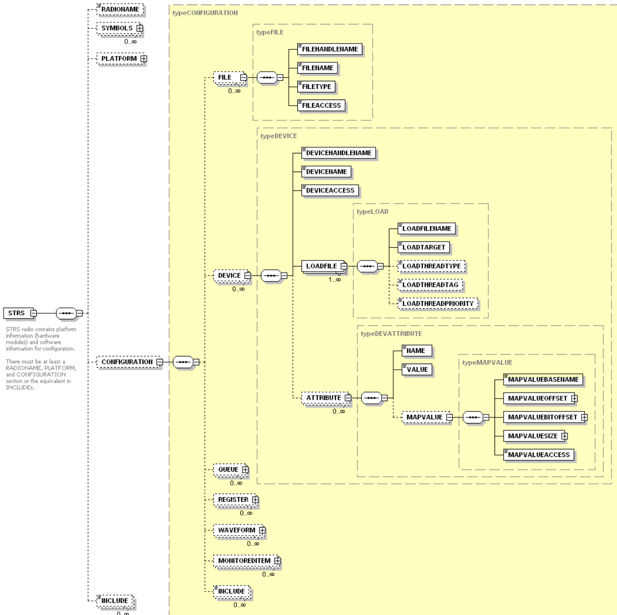
Figure 11-2 Example of software portion of STRS Platform Configuration File
