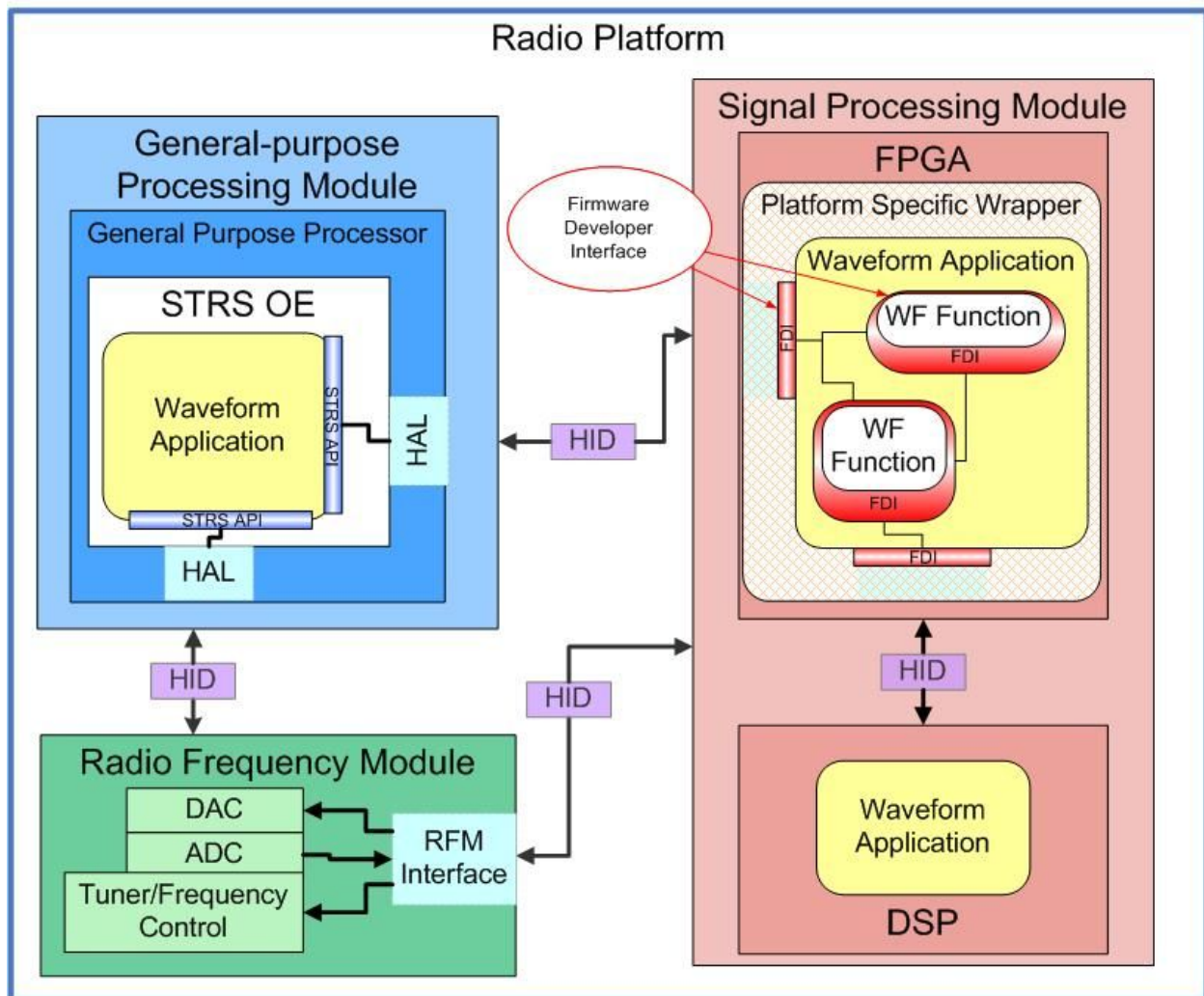
Figure 7-2 Proposed Firmware Architecture Extension
