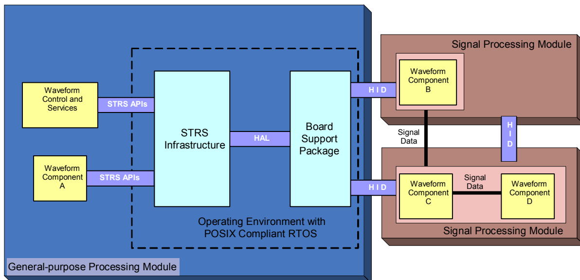
Figure 6-1 Waveform Component Instantiation
