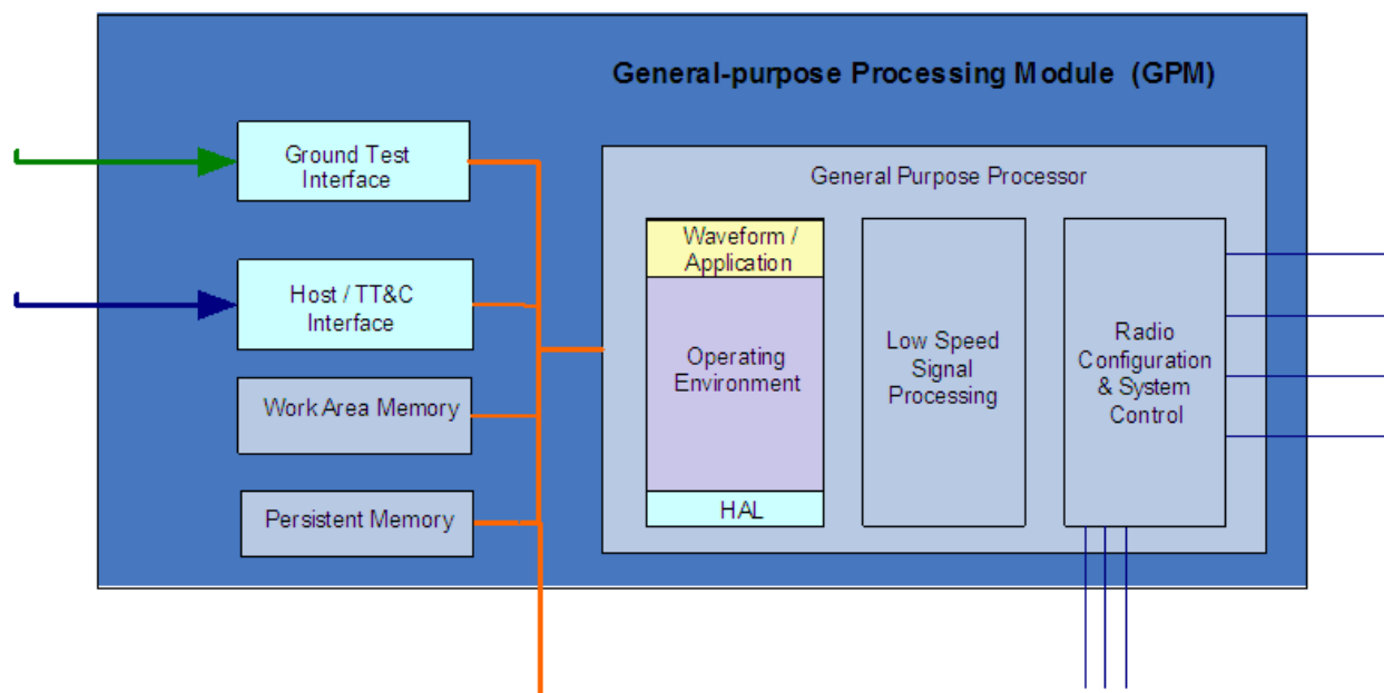
Figure 5-3 GPM Architecture Details
