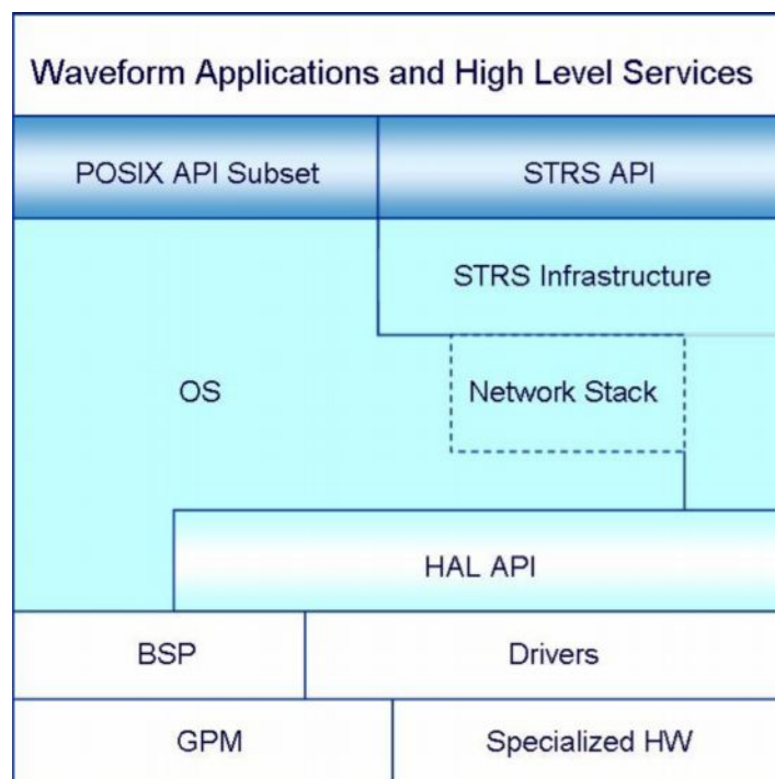
Figure 8-1 STRS Software Execution Model
