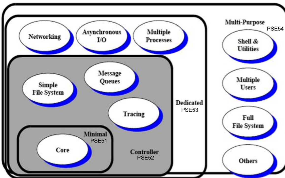
Figure 8-8 Profile Building Blocks
