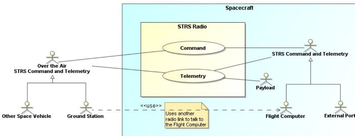
Figure 9-1 Command and Telemetry Interfaces
