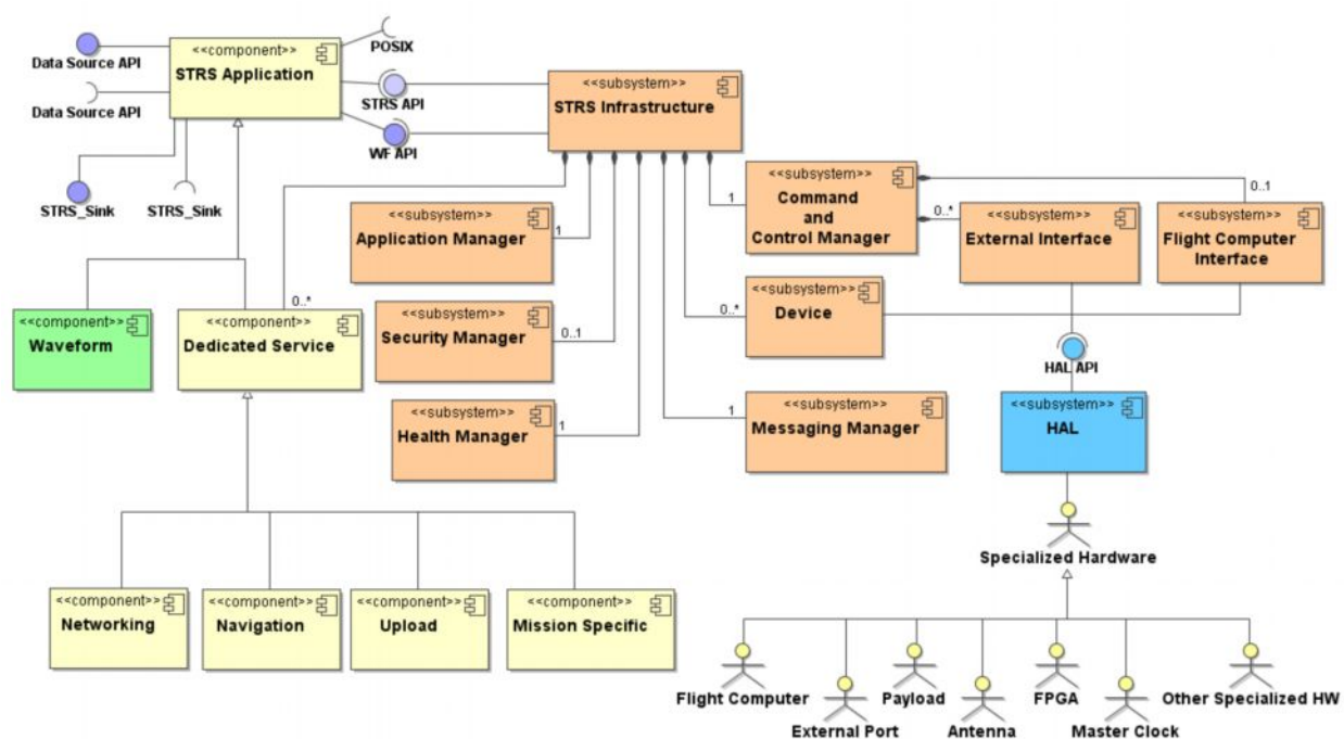
Figure 8-5 STRS infrastructure
