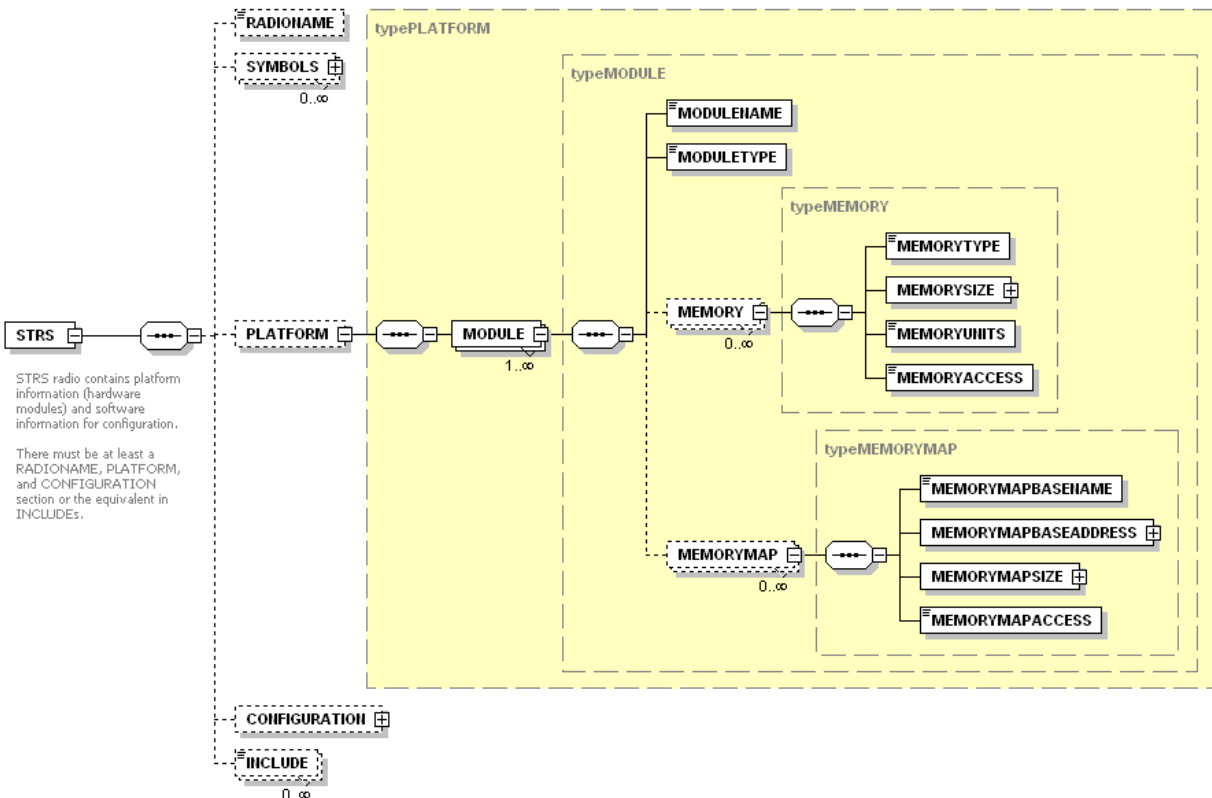
Figure 11-1 Example of hardware portion of STRS Platform Configuration File
