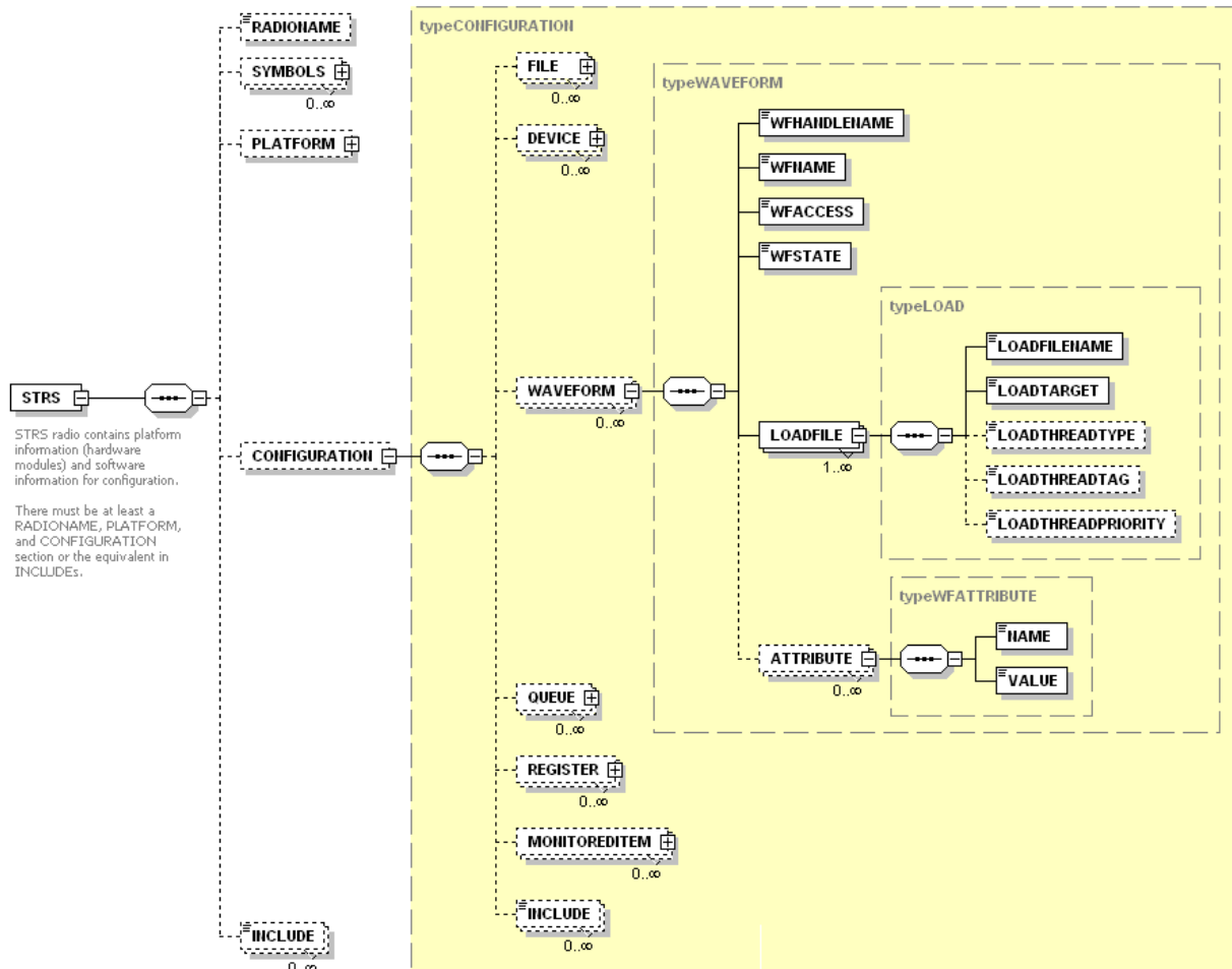
Figure 11-3 Example of STRS WF Configuration File
