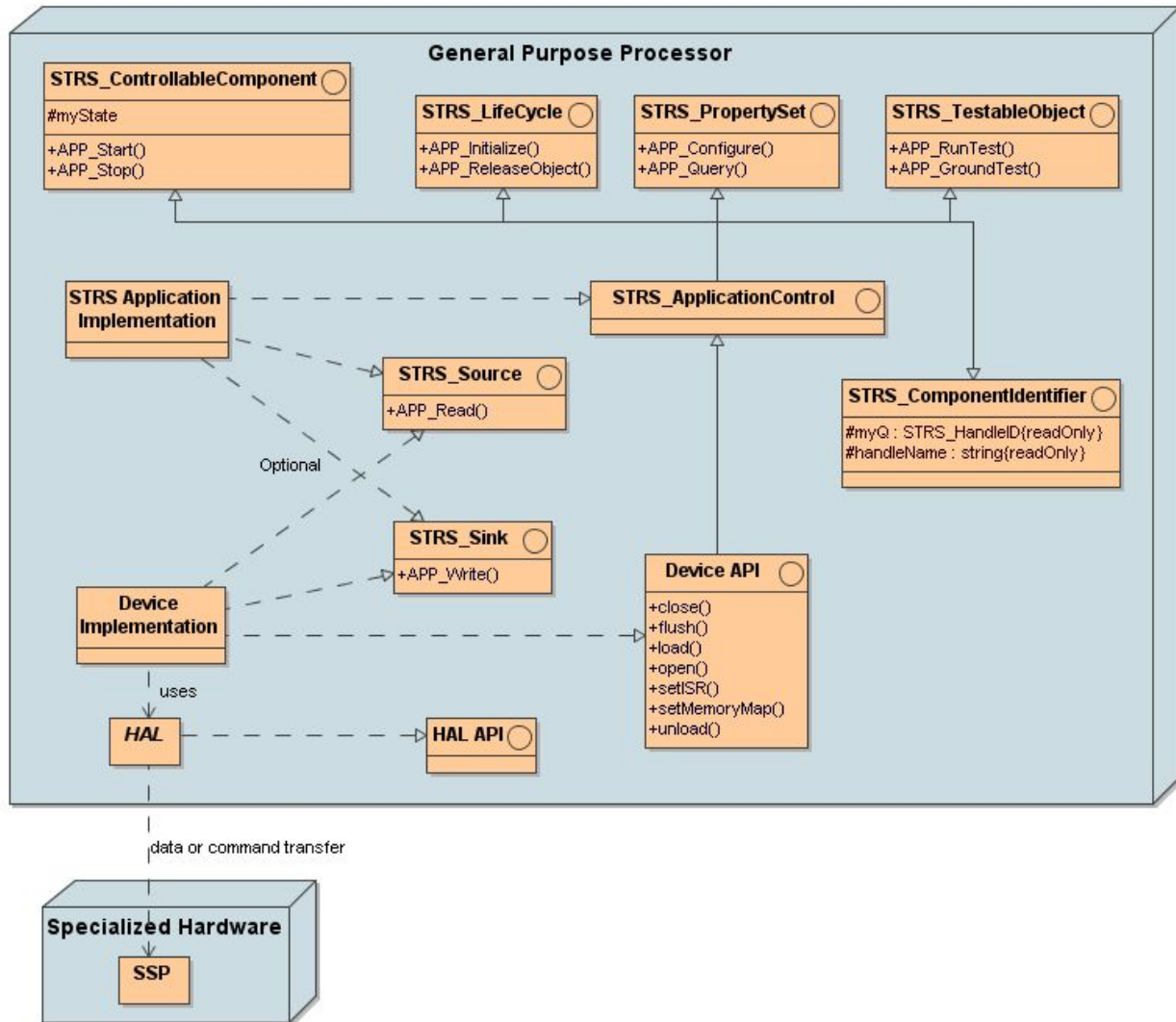
Figure 8-6 STRS Application/Device Structure
