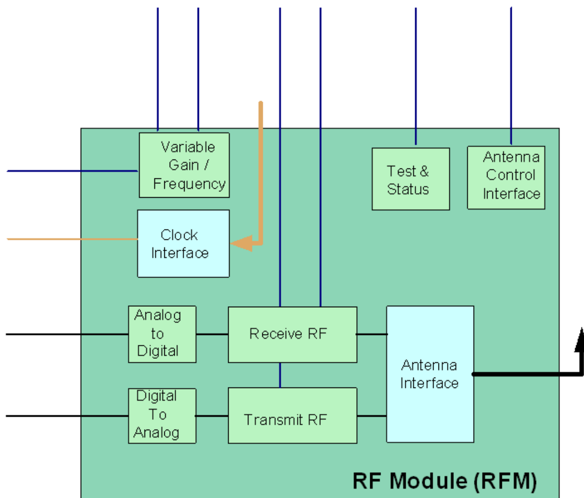
Figure 5-5 RFM Architecture Details
