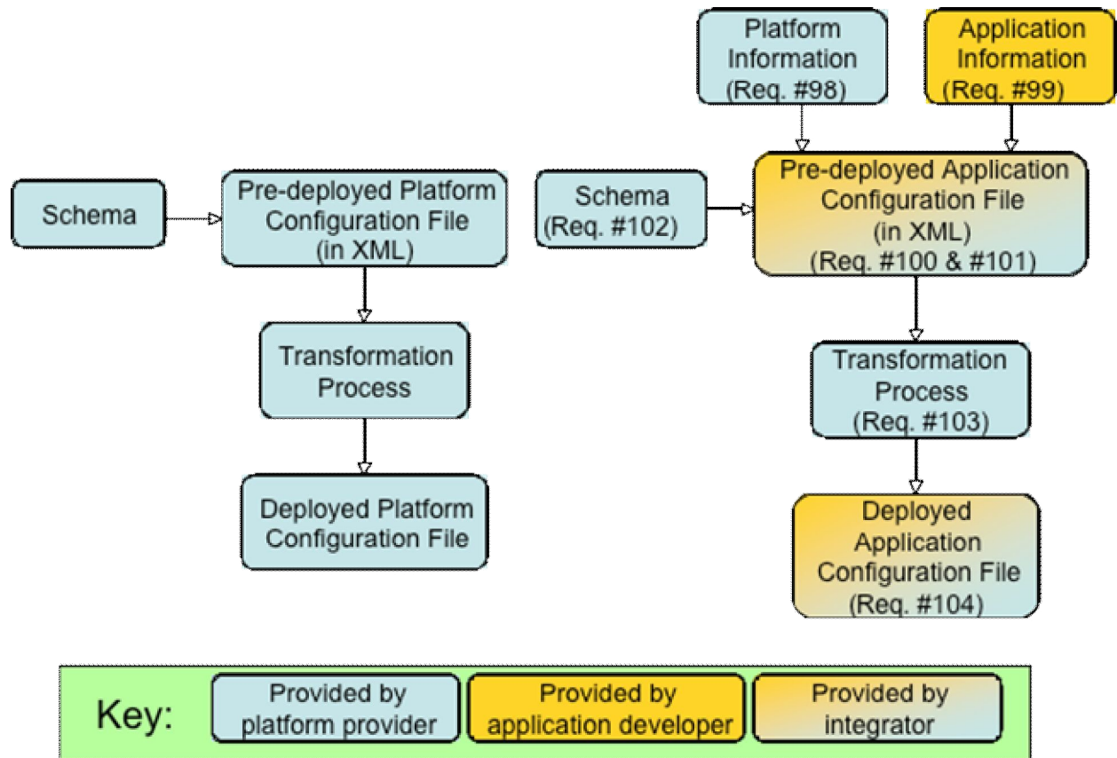
Figure 10-2 Configuration File Development Process
