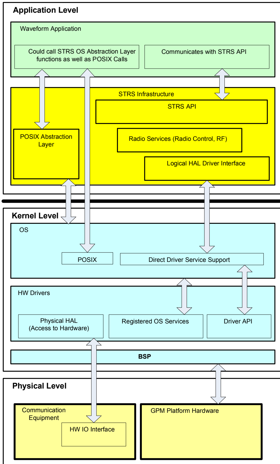
Figure 8-3 STRS Operating Environment
