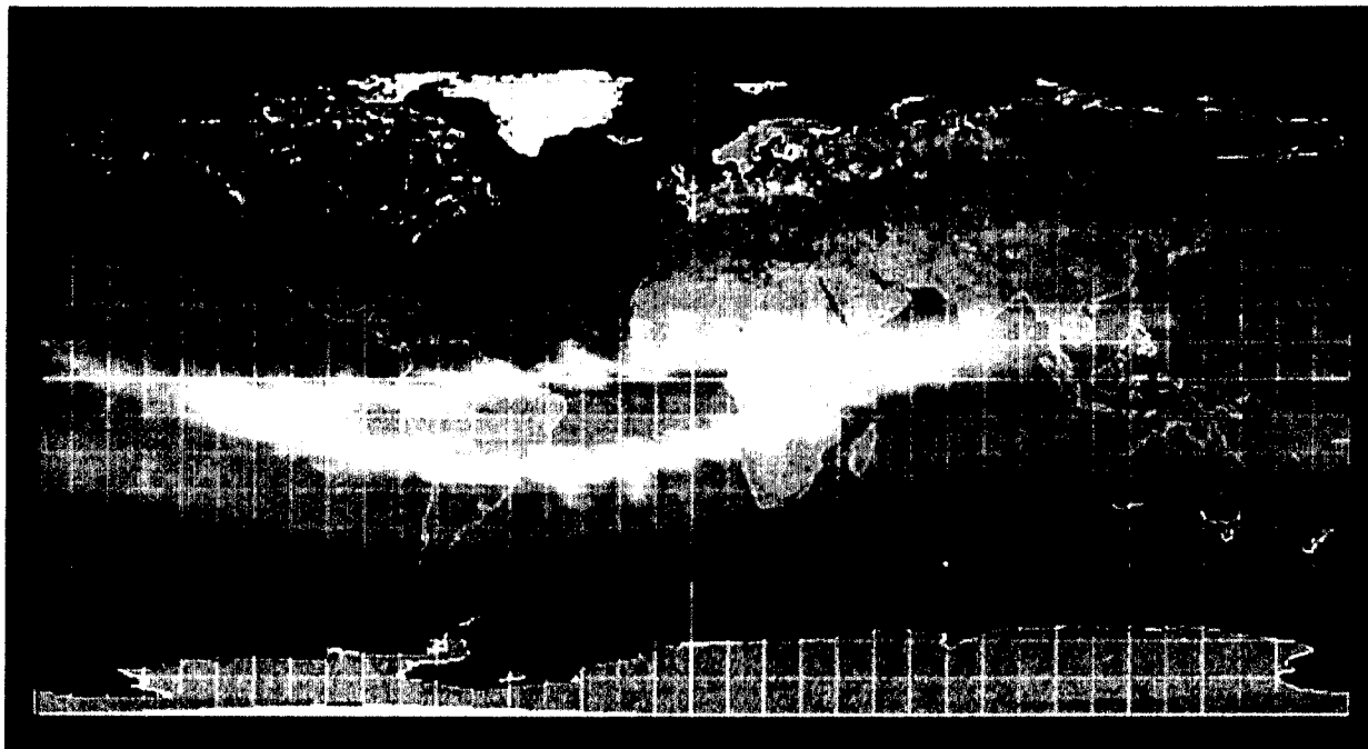
Figure 5. Contour plot of the trapped proton environment overlaying a map of the Earth. 2 Proton density increases from blue to green to yellow to red. Contours highlight the South Atlantic Anomaly (SAA) where the radiation particle population is high due to the offset nature of the Earth's magnetic field.
