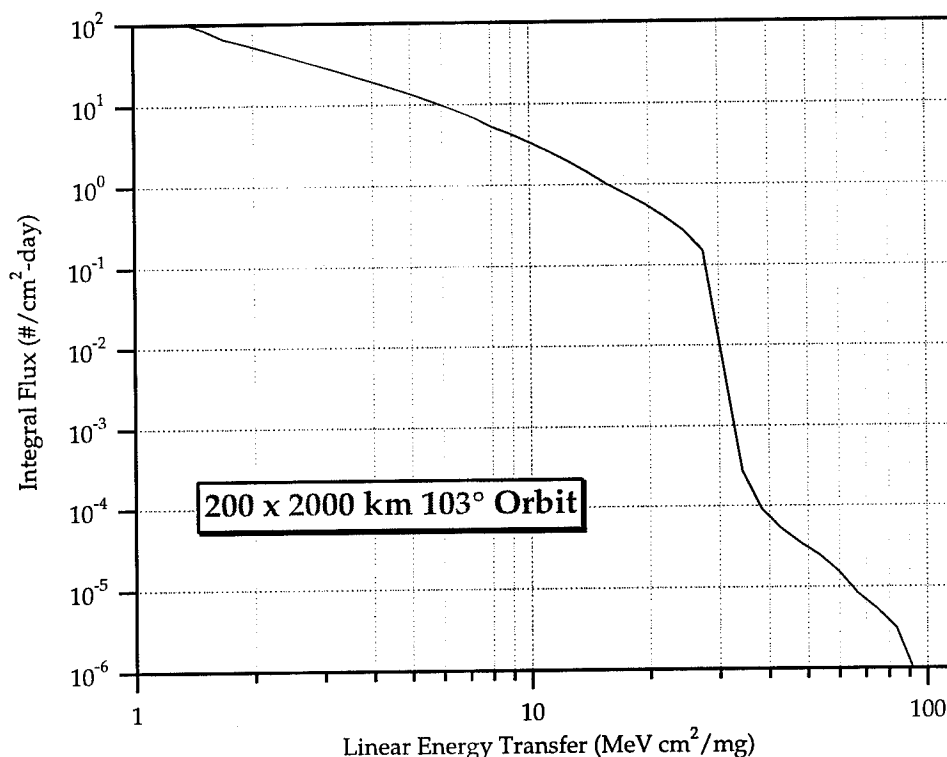
Figure 10. Single event effects (SEE) producing environment for a polar orbit. An important feature is the rapid reduction in the environment for LET greater than approximately 28.
