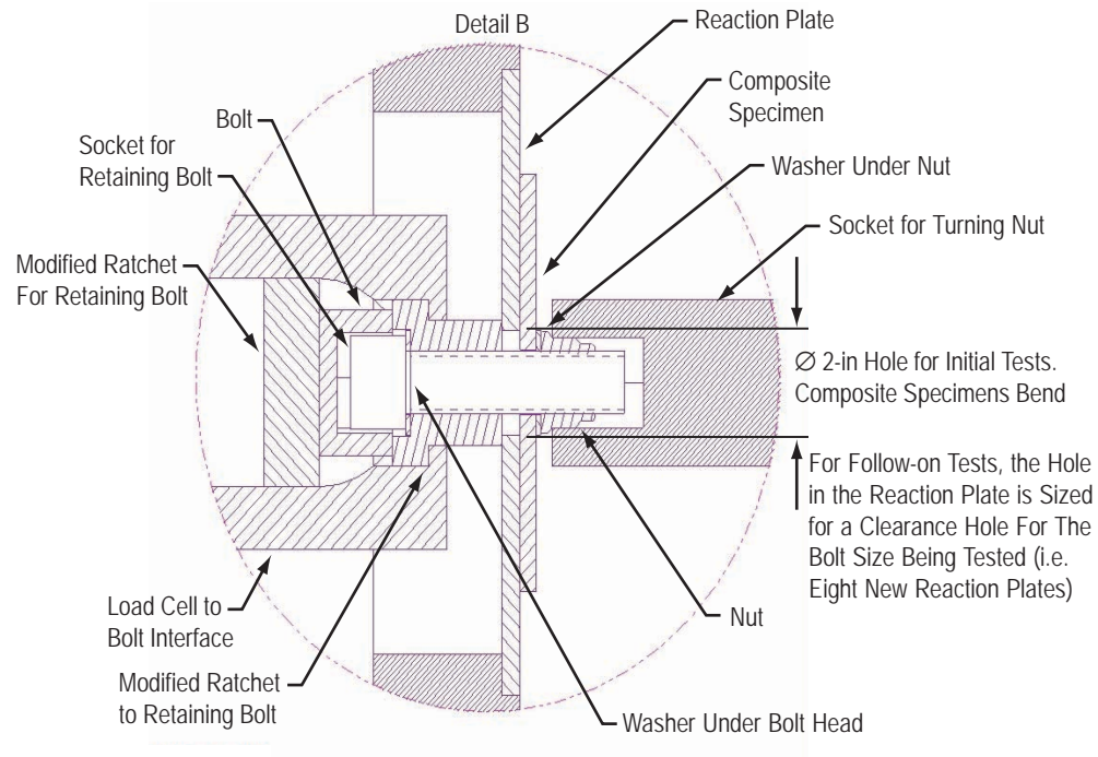
Figure 6. Details of specific test components.
