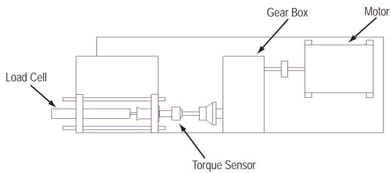
Figure 3. Top view of torque versus tension machine.
