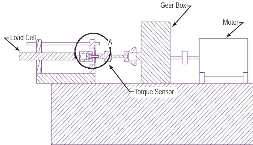
Figure 4. Torque versus tension cross section.
