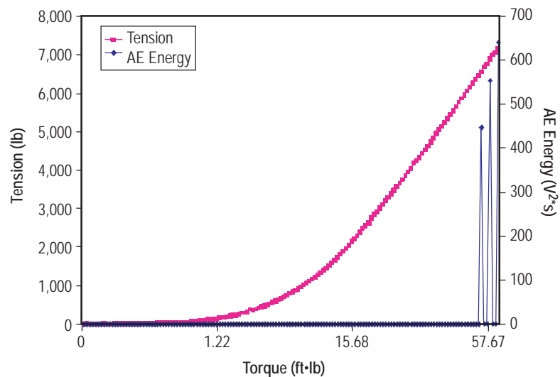
Figure 10. Torque versus tension and torque versus acoustic emissions energy follow-on test with 1/2-in bolt, IM7/8552 material, 0.185-in thick.
