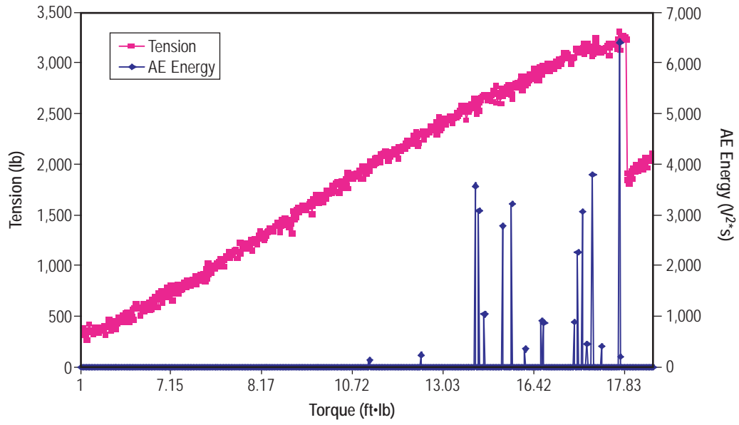
Figure 7. Torque versus tension and torque versus acoustic emissions energy—specimen 33.
