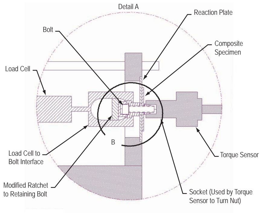
Figure 5. Detailed view of test setup.
