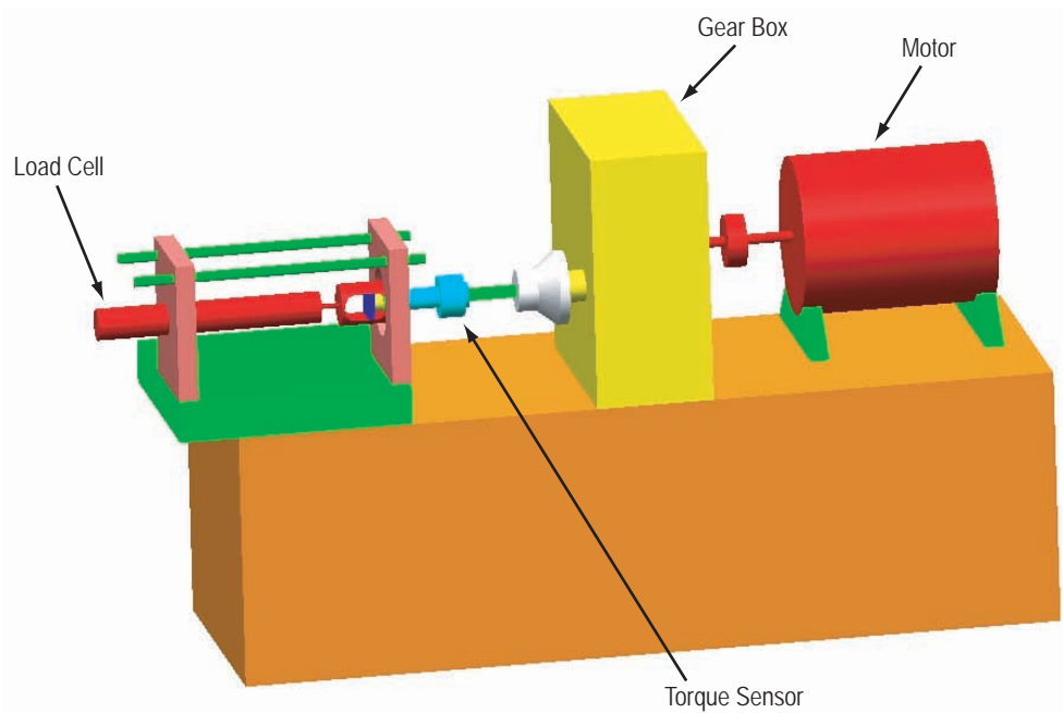
Figure 2. Torque versus tension machine configuration.
