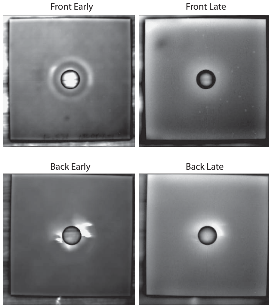
Figure 8. Thermal images of test specimen.
