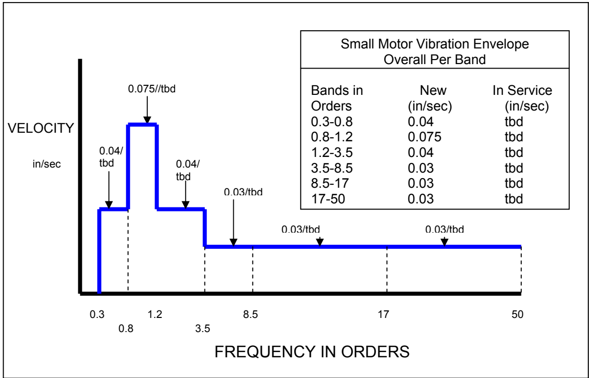
Figure 2-9: Small Motor Vibration Envelope Overall Per Band
