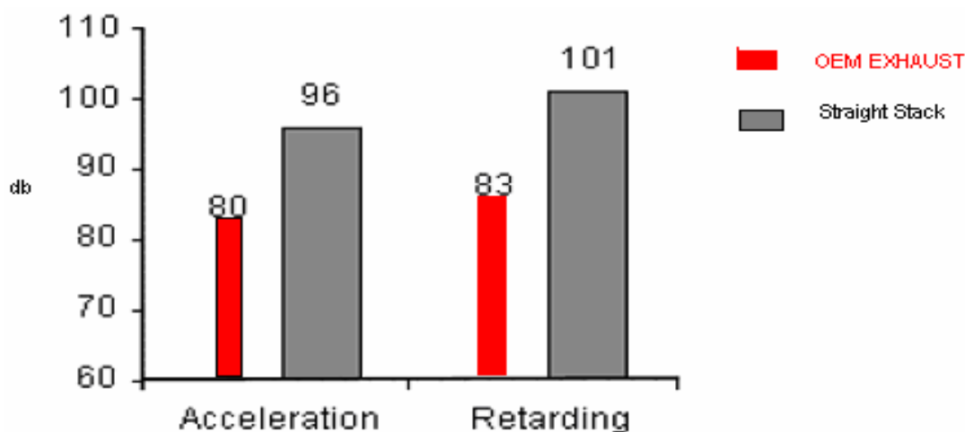
Figure 2-5: Acceptable Noise Levels
