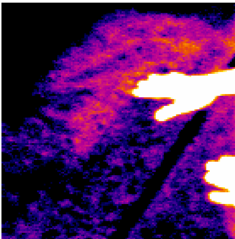
Figure 2-14: Infrared Image of Moisture Under Roof 8
