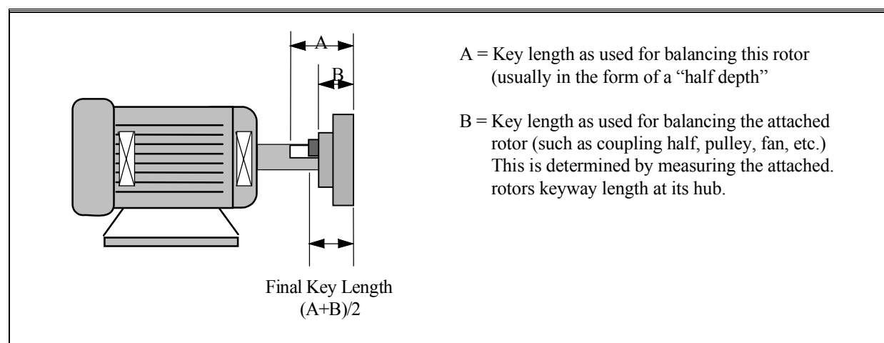
Figure B-1: Balance Test Key Dimension
