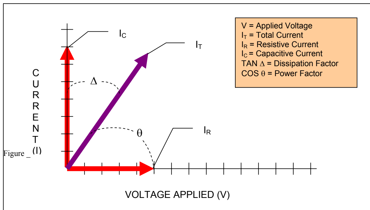
Figure B-11: Phase Relationships
