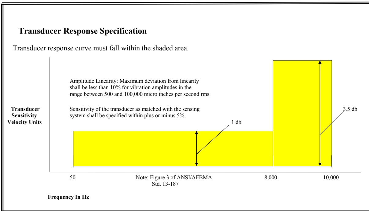
Figure 2-1: Transducer Response
