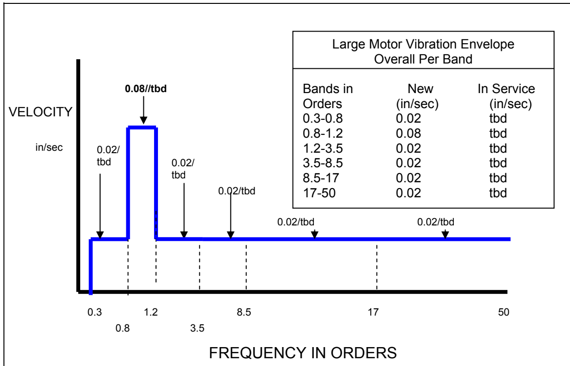
Figure 2-10: Large Motor Vibration Envelope Overall Per Band
