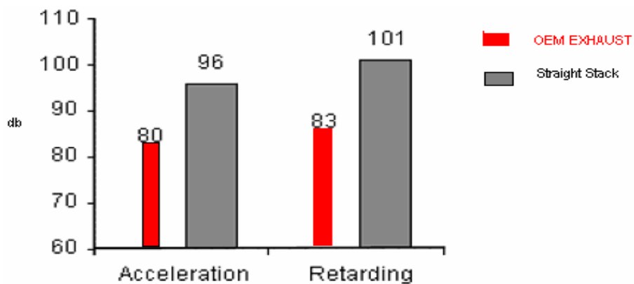
Figure 2-4: Acceptable Noise Levels
