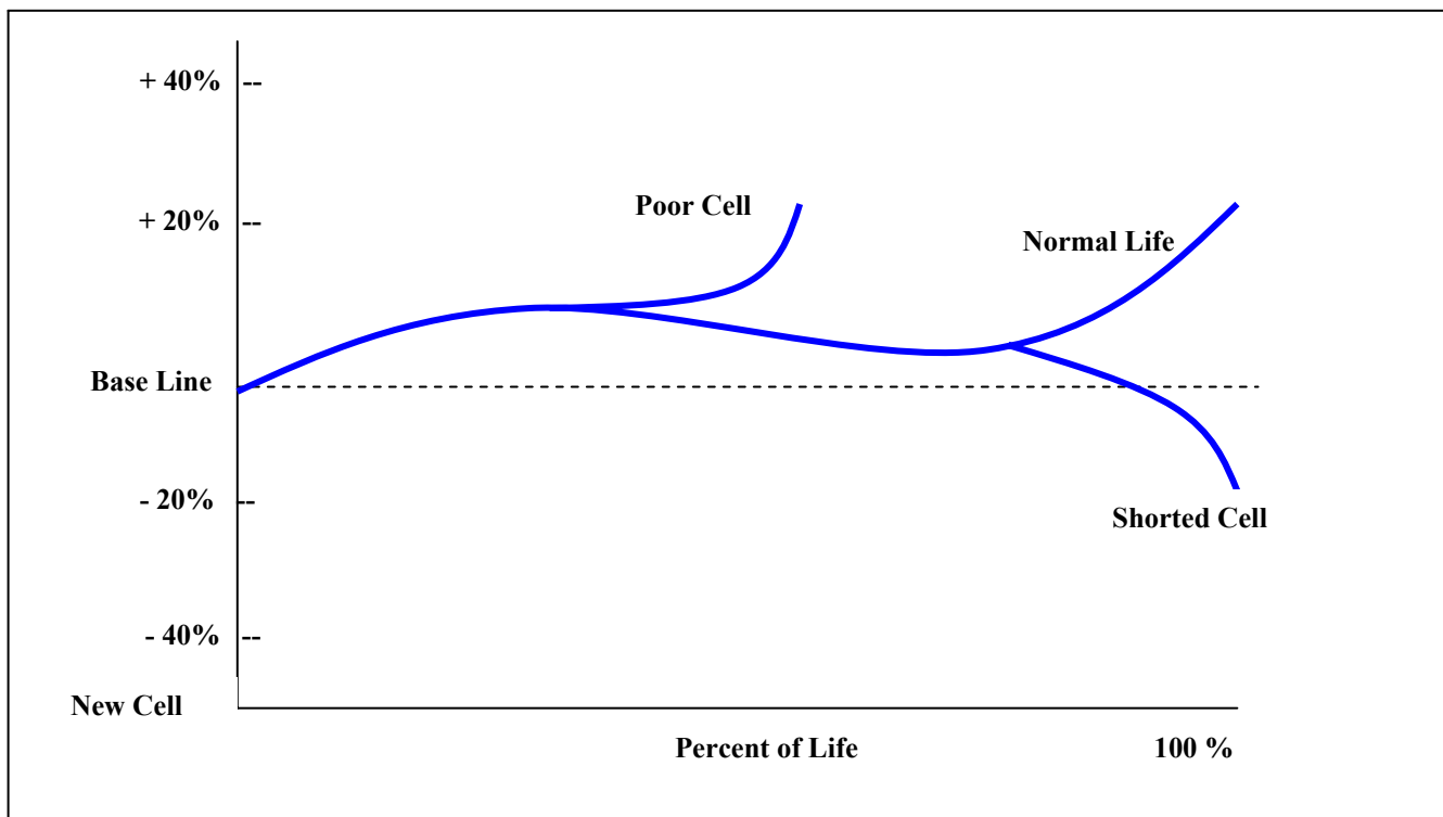
Figure B-16: Typical Battery Impedance Versus Age
