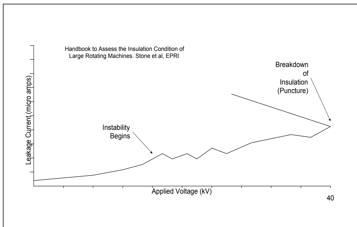
Figure B-19: Hi-Pot Testing Example
