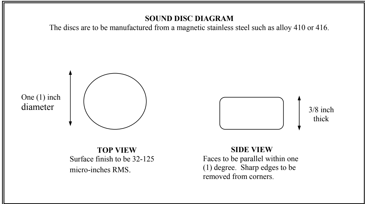
Figure B-5: Sound Disc Diagram
