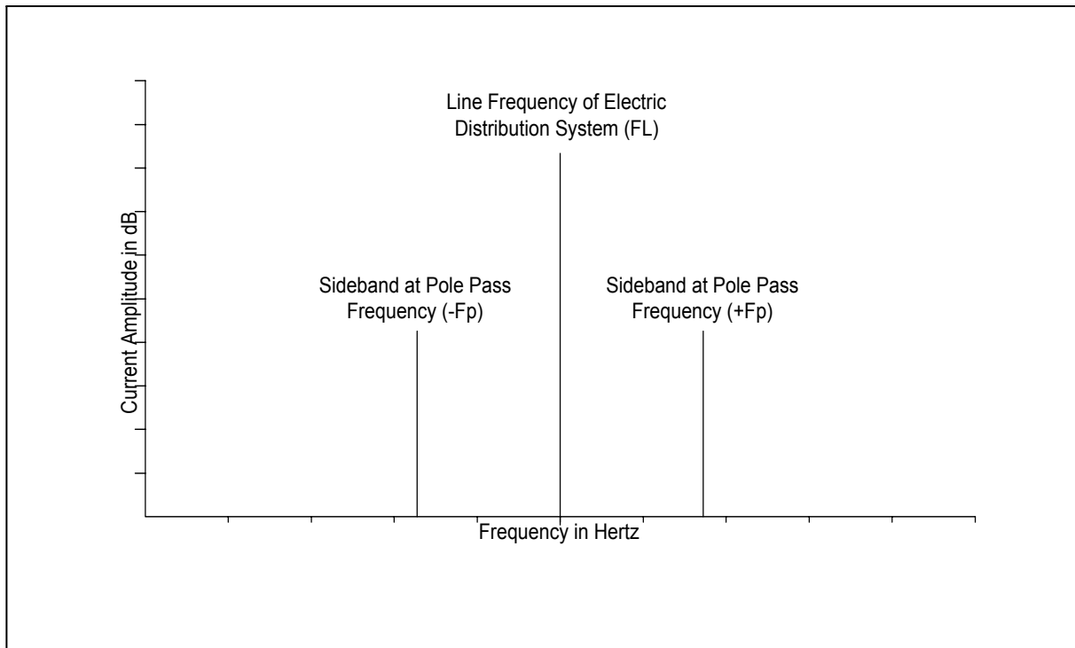
Figure B-17: Simplified Motor Current Signature
