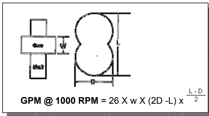
Figure 2-12: Figuring Gear Pump G.P.M.
