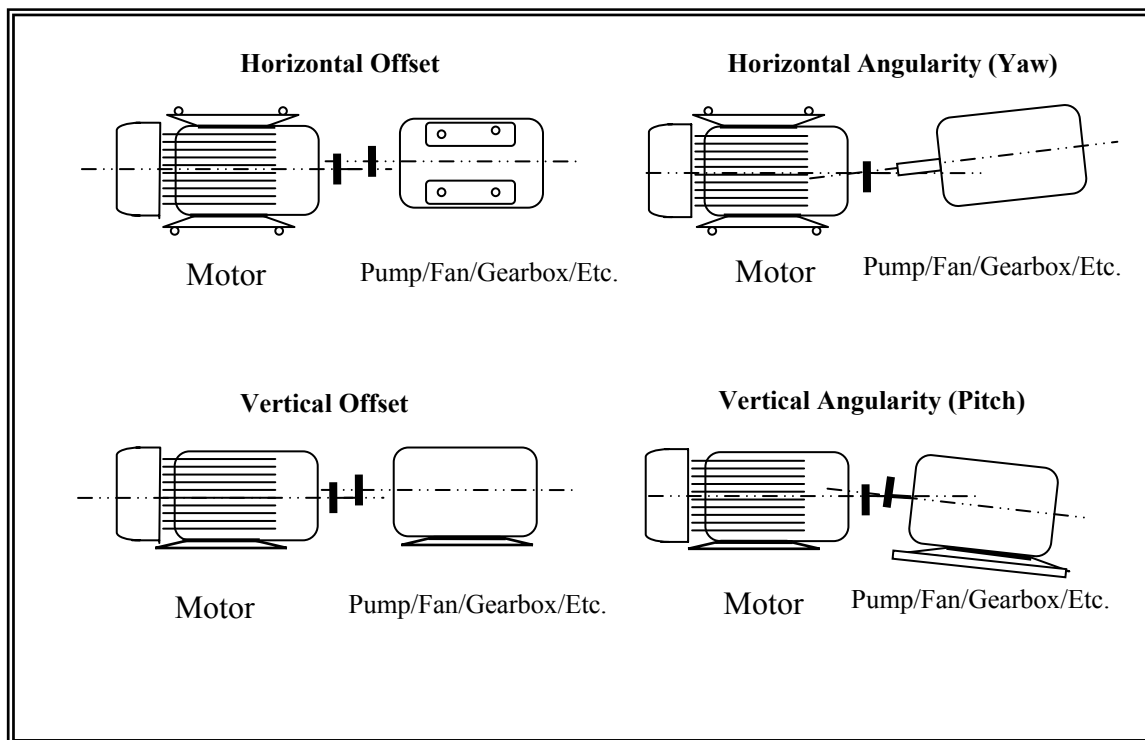
Figure B-2: Offset and Angular Misalignment
