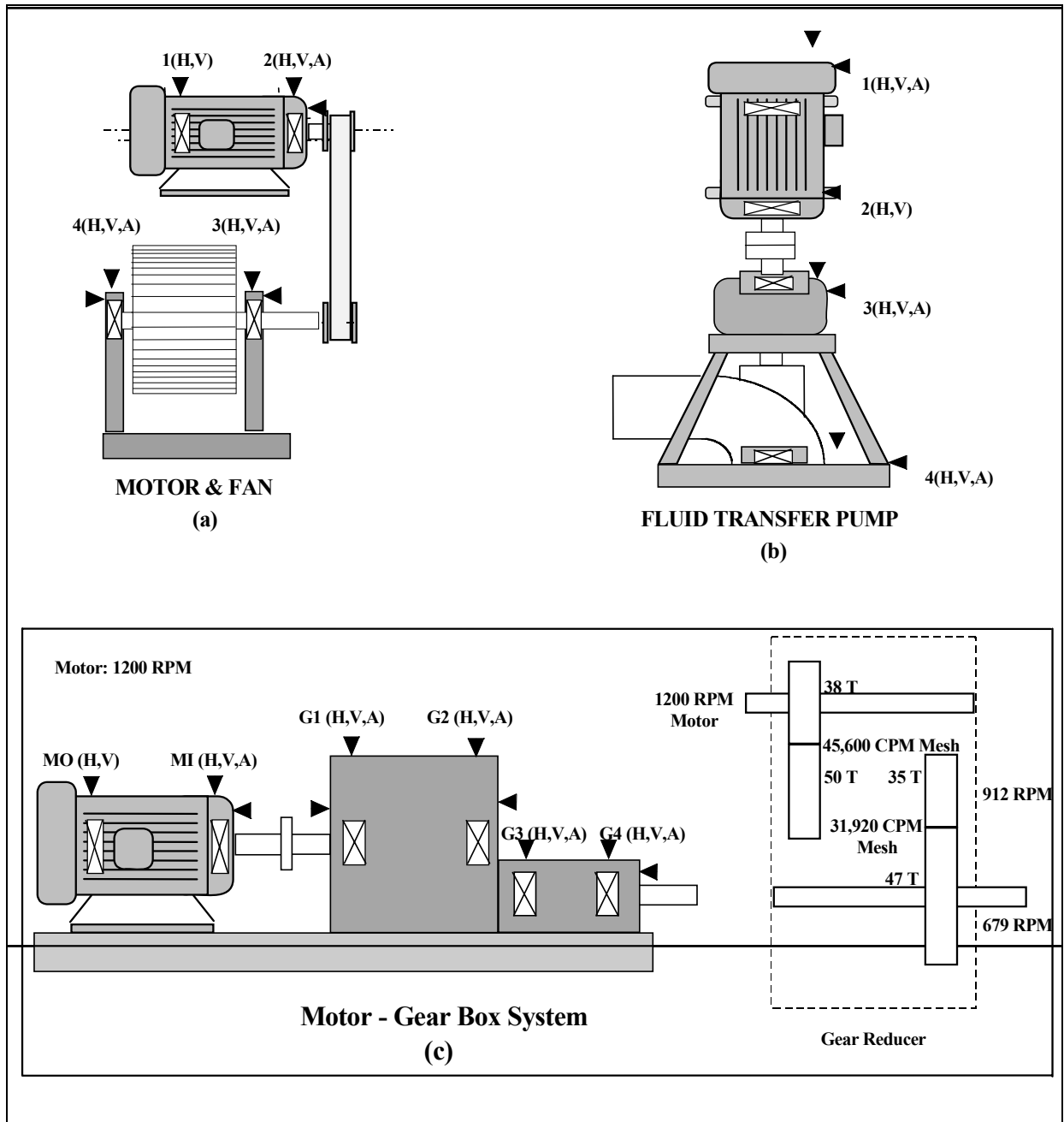
Figure B-4: Typical Vibration Measurement Locations
