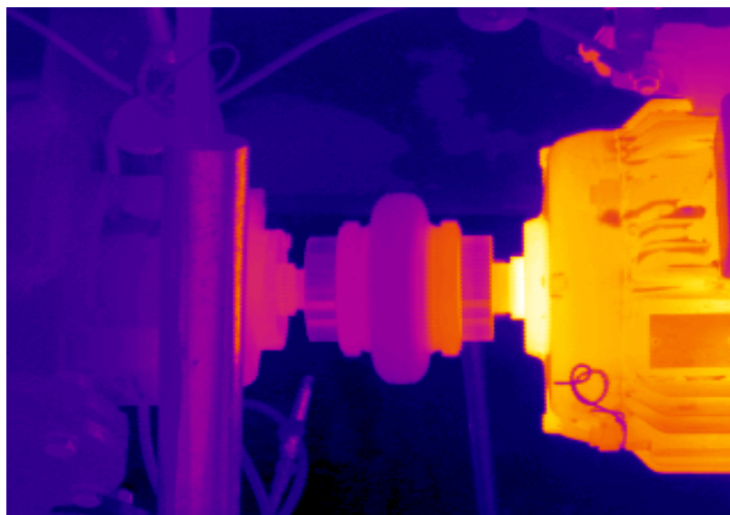
Figure B-10: Infrared Image of Motor/coupling 11
