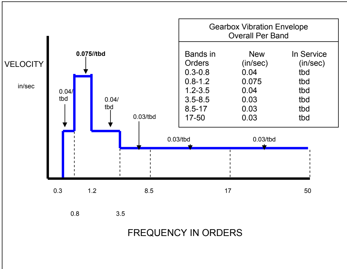
Figure 2-8: Gearbox Vibration Envelope Overall Per Band
