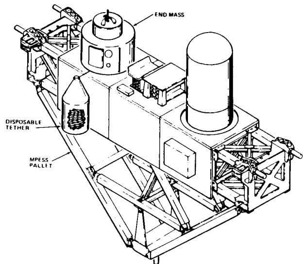
SEDS SYSTEM INTEGRATED TO AN MPESS PALLET
