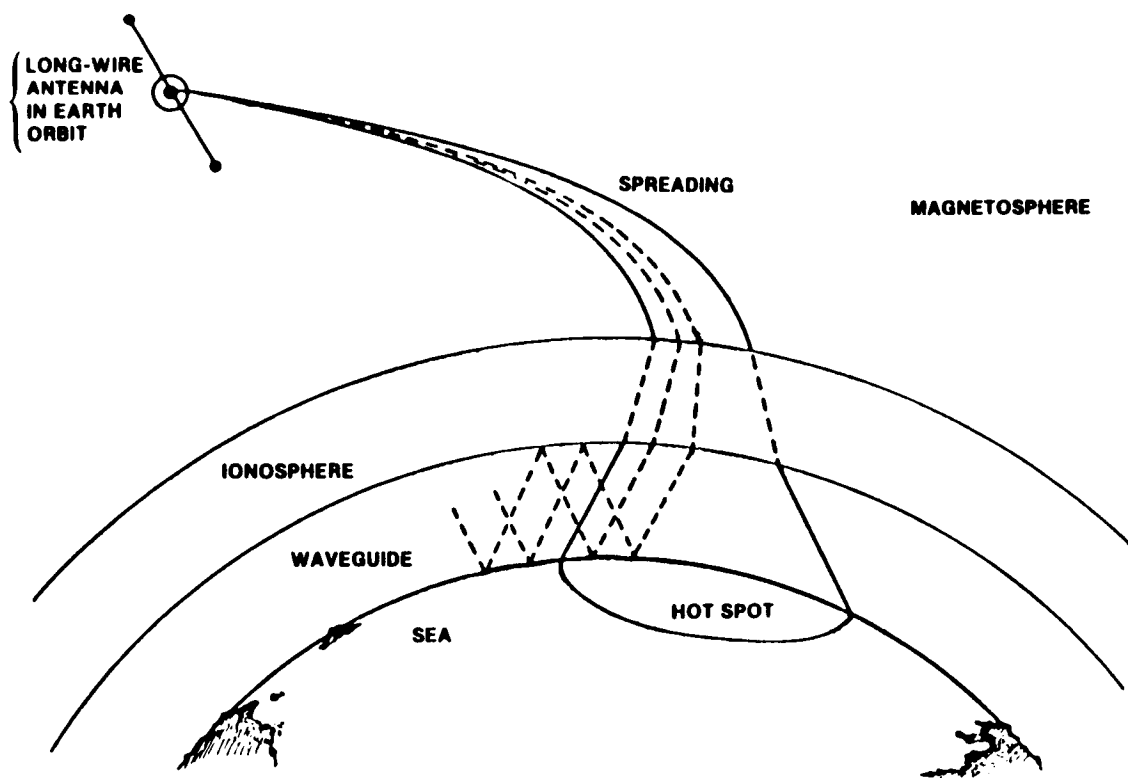
Figure 2.19. Propagation of ULF/ELF/VLF Waves To The Earth's Surface From An Orbiting Tether Antenna [reference 15]
