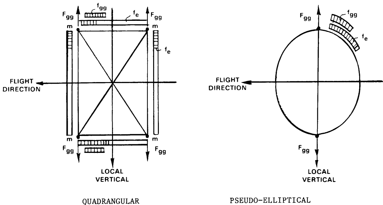
Figure 2.9. Two Designs of ESC 2-D Constellations Where Shape Stability is Provided by Electromagnetic Forces [Ref. 10, p. 174]
