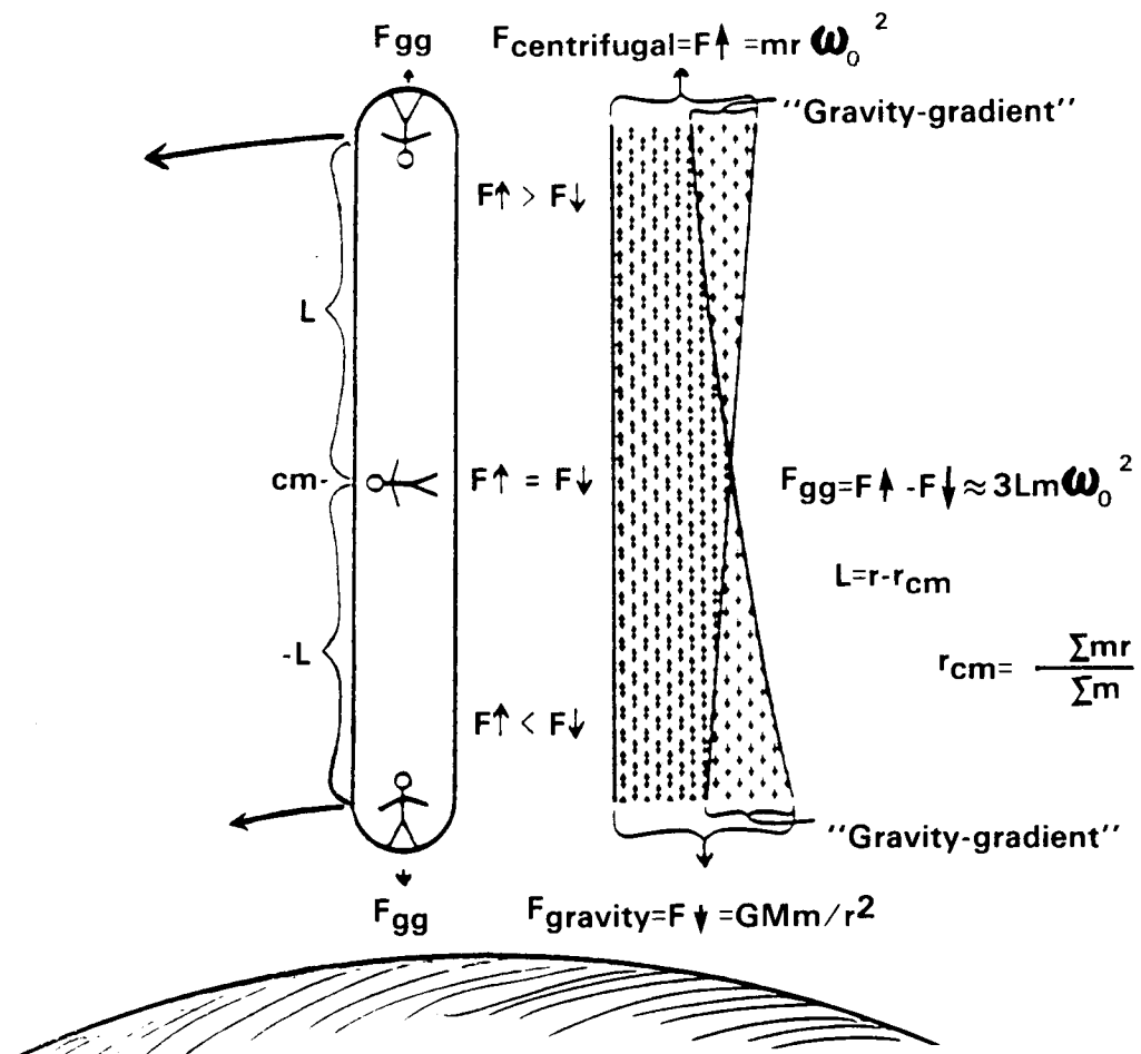
Figure 2.3. Origin of Gravity-Gradient Forces
